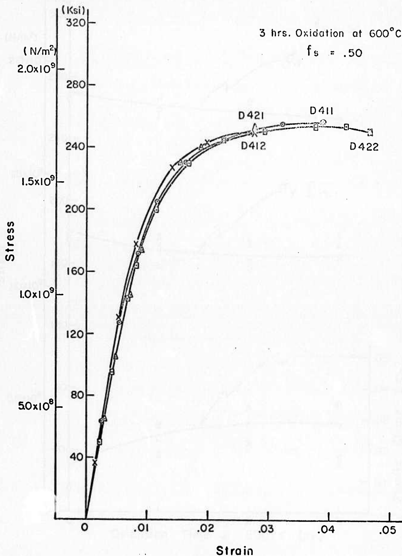
Figure 10. The Stress-Strain Curves for Specimens with 3 hrs. Oxidation at 600°C.
