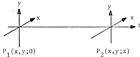
Fig. 1. Geometry of planes P_1 and P_2 .
