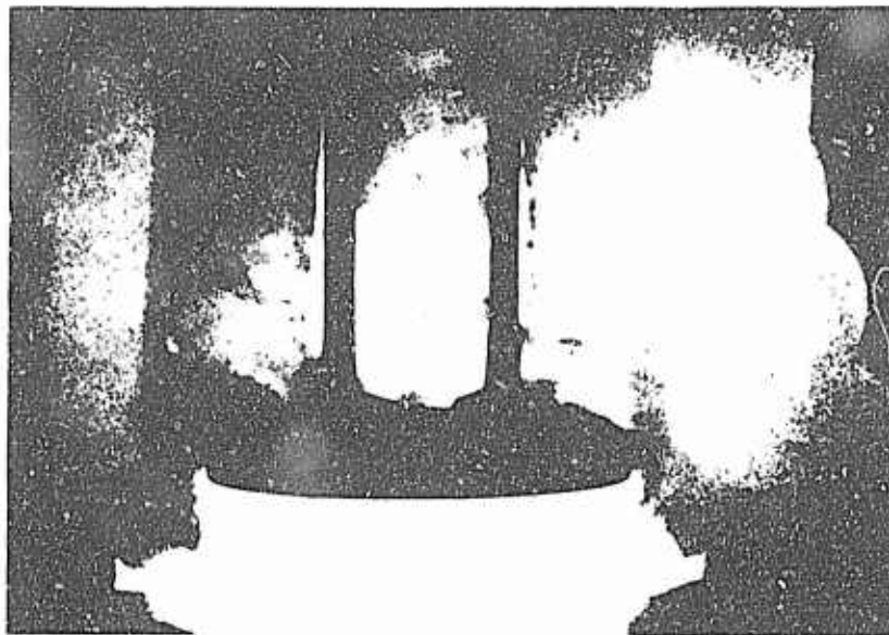
Figure 6. Plate anchor excavated after load test in snow showing the backfill and in-situ snow. (From Reference 10.)
