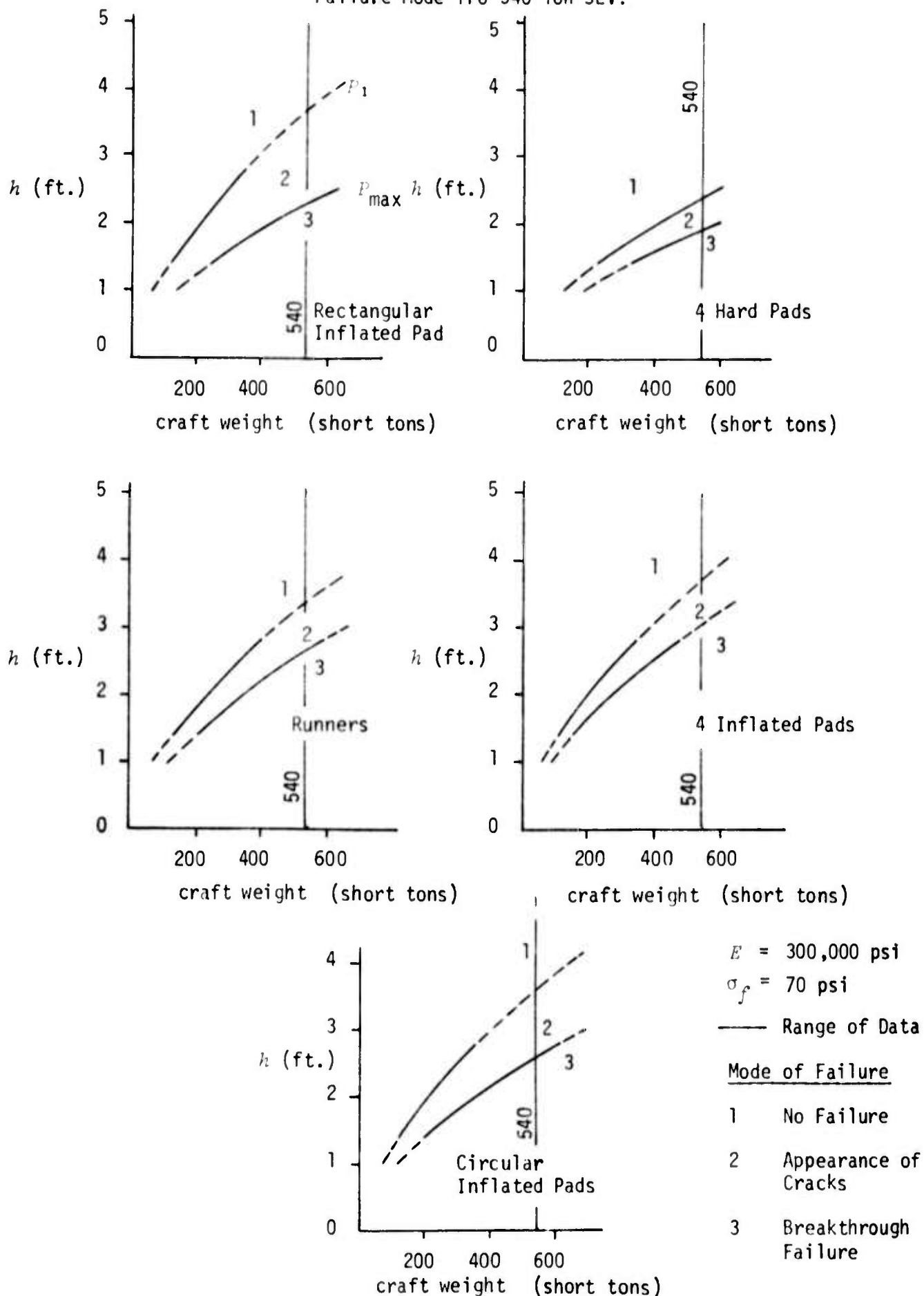
Failure Mode from 540 Ton SEV.
