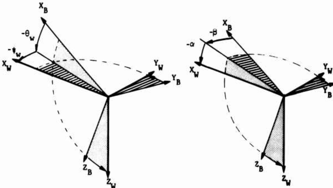
(a) Rotations With Wind Tunnel Angles.
