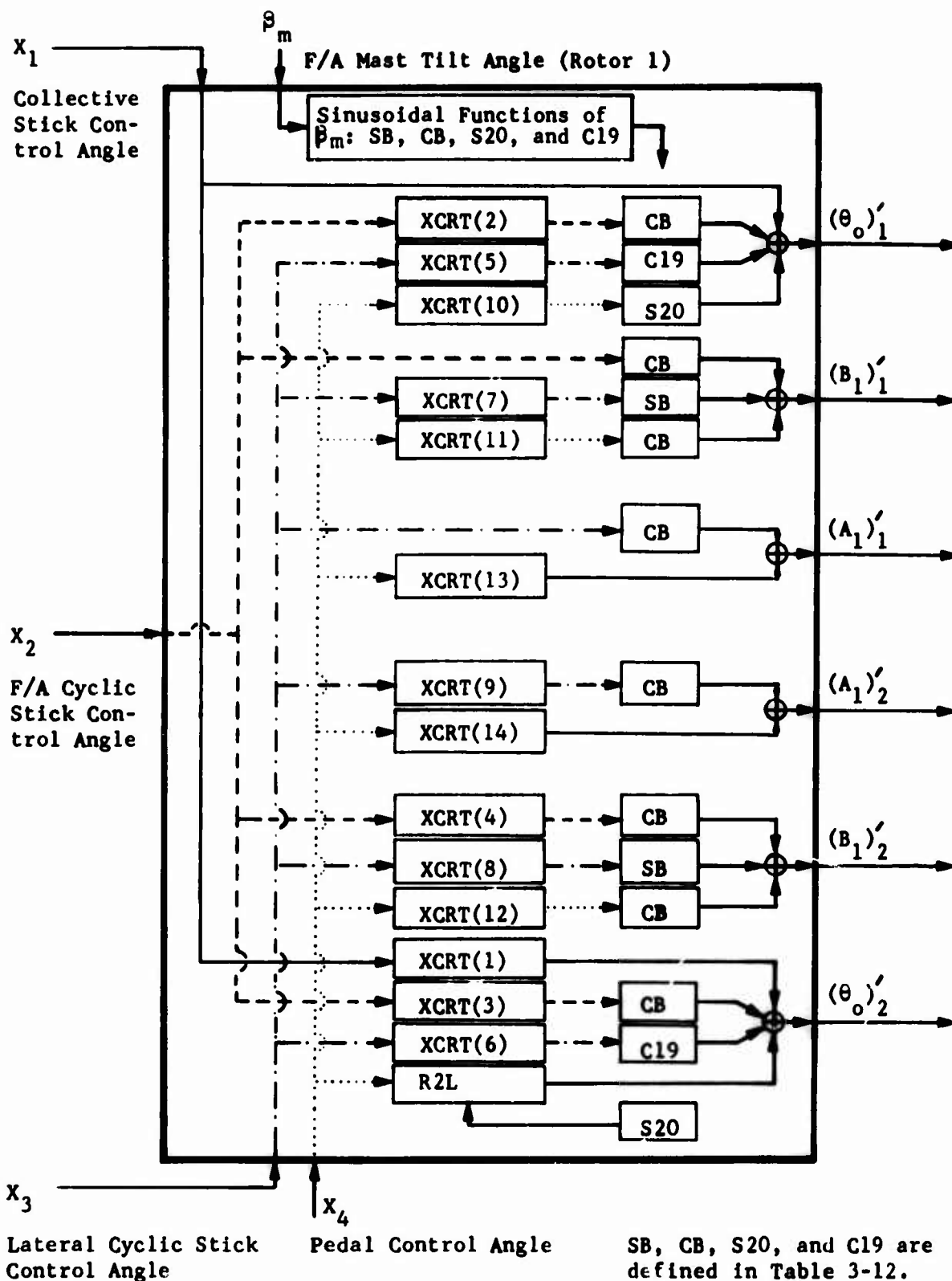
Figure 3-12. Schematic Diagram of Control Coupling/Mixing Box.
