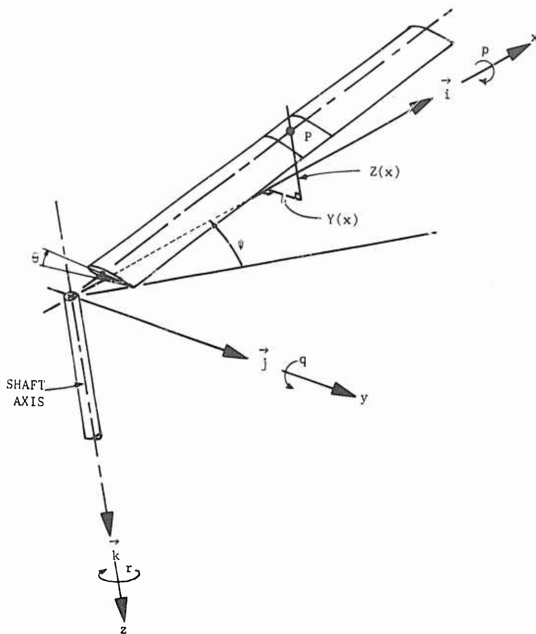
Figure 3-1. Reference System for Rotor Analysis.
