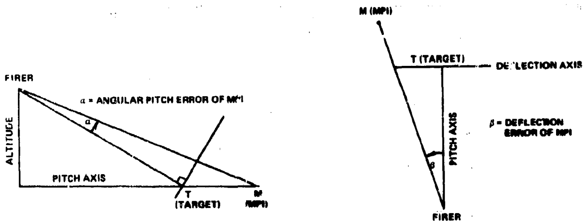
FIGURE A-1. Line of Sight Transformation of Error of the MPI
