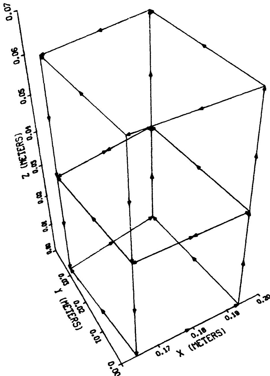
Figure 7. Finite-element idealization of the top half of one stave of the cylinder.
