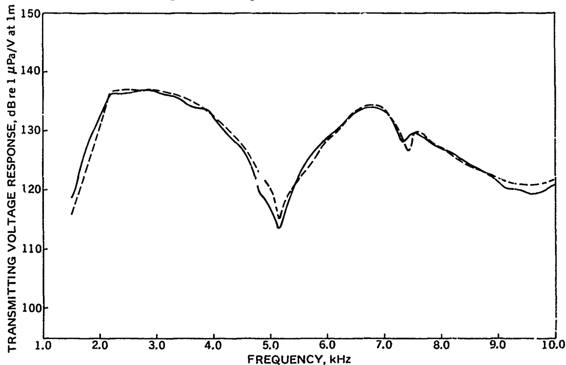
Figure 10. Transmitting voltage response of Cylinder A as a function of frequency. Solid line is for experiment and dashed line for theory.
