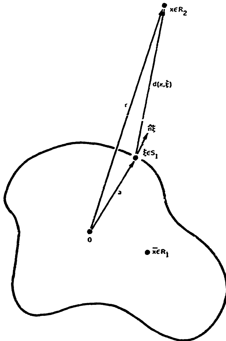
Figure 2. Euclidean 3-space divided into two regions, R_1 and R_2 , by the closed surface S_1 . x is a point in R_2 , \bar{x} a point in R_1 , and \xi a point on S_1 .
