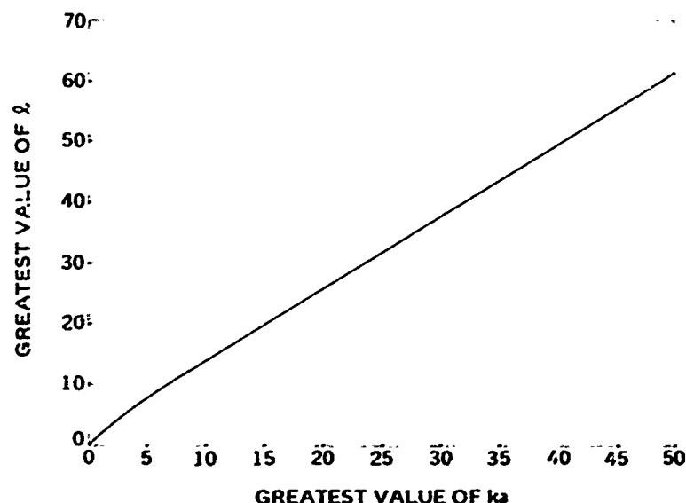
Figure 4. Plot of the greatest value of l that is needed in the spherical harmonic expansion as a function of the non-dimensional frequency ka .
