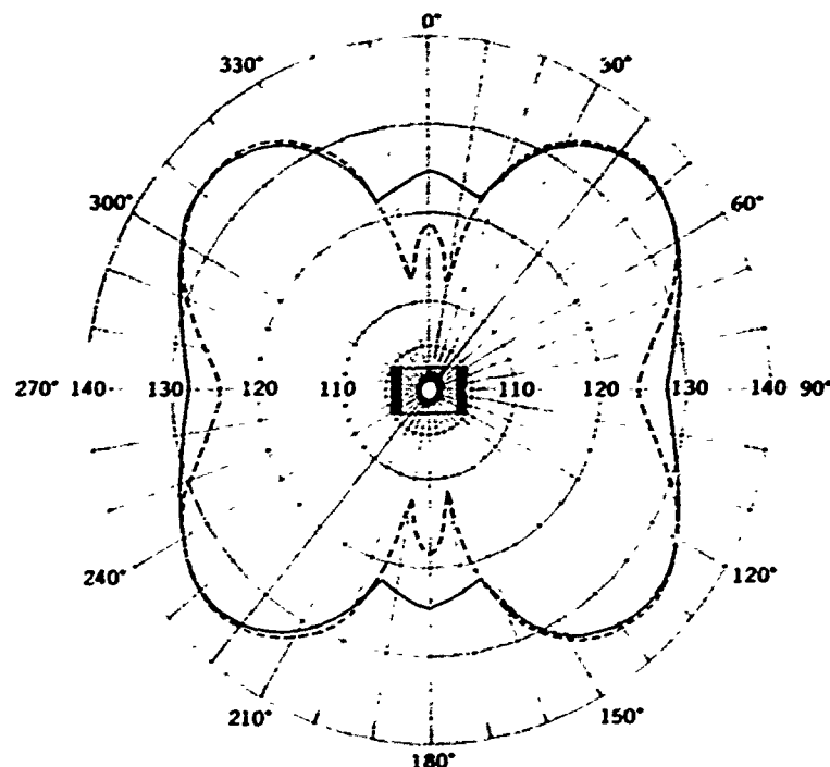
Figure 21. Vertical directivity pattern for Cylinder Cat 10,000 Hz. Solid line is for experiment and dashed line for theory. Pressures are plotted in dB re 1 \mu Pa for 1 V input at 1 m.
