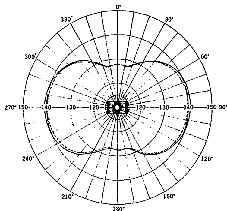
Figure 15. Vertical directivity pattern for Cylinder B at 4,500 Hz. Solid line is for experiment and dashed line for theory. Pressures are plotted in dB re 1 \mu\text{Pa} for 1 V input at 1 m.
