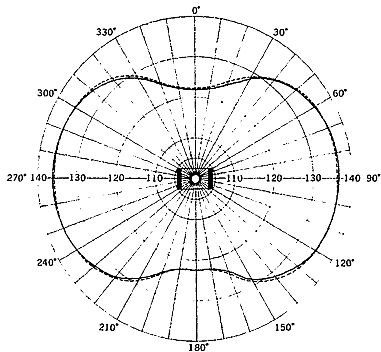
Figure 11. Vertical directivity pattern for Cylinder A at 3,000 Hz. Solid line is for experiment and dashed line for theory. Pressures are plotted in dB re 1 \mu\text{Pa} for 1 V input at 1 m.
