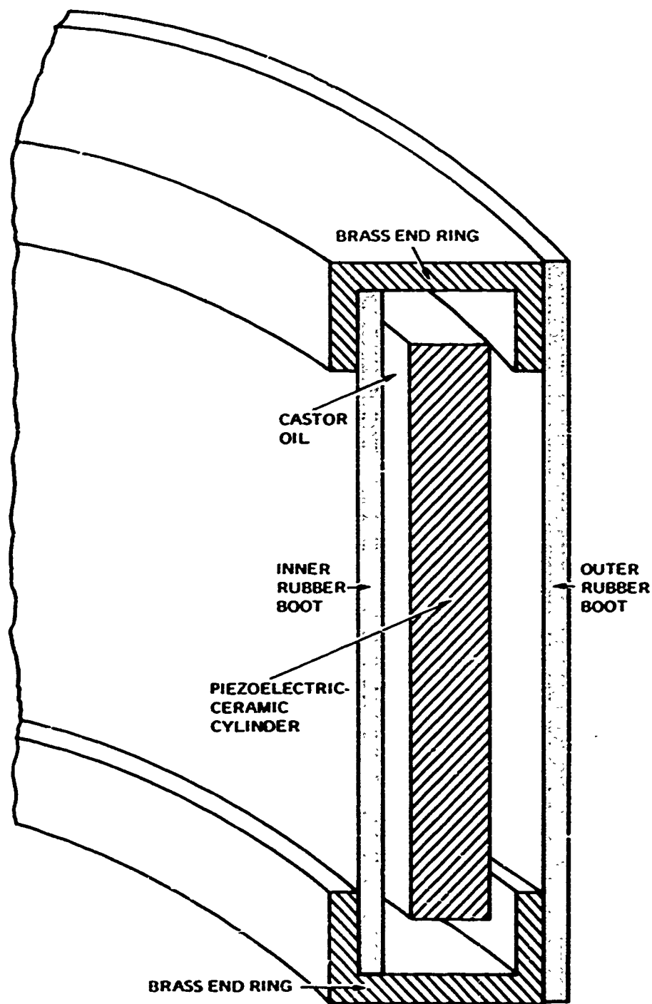
Figure 8. Cross-sectional drawing of a typical free-flooded cylinder transducer in its case, including the ceramic cylinder, brass end rings, inner and outer rubber boots, and castor oil filling of the case.
