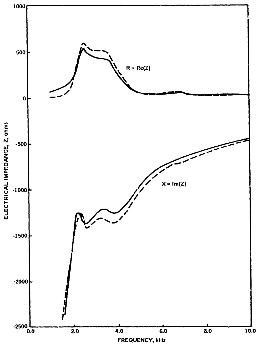
Figure 9. In-water complex electrical impedance of Cylinder A as a function of frequency. Solid lines are for experiment and dashed lines for theory.
