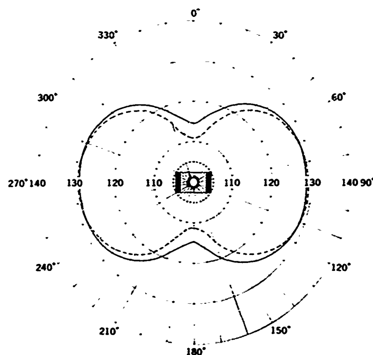
Figure 20. Vertical directivity pattern for Cylinder Cat at 6,000 Hz. Solid line is for experiment and dashed line for theory. Pressures are plotted in dB re 1 \mu\text{Pa} for 1 V input at 1 m.
