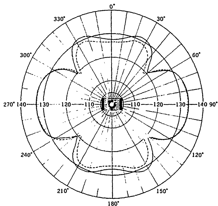
Figure 12. Vertical directivity pattern for Cylinder A at 7,000 Hz. Solid line is for experiment and dashed line for theory. Pressures are plotted in dB re 1 \mu\text{Pa} for 1 V input at 1 m.
