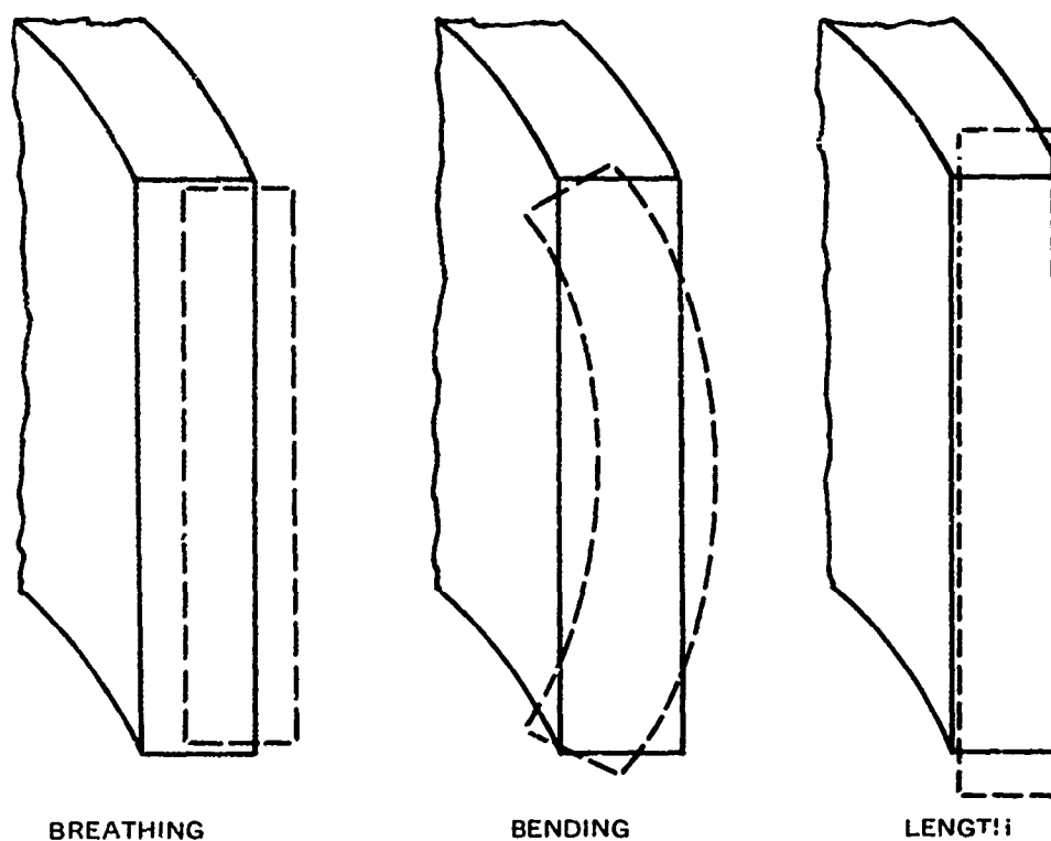
Figure 3. Cross-sectional drawing of the first three resonant modes of a free-flooded cylinder.
