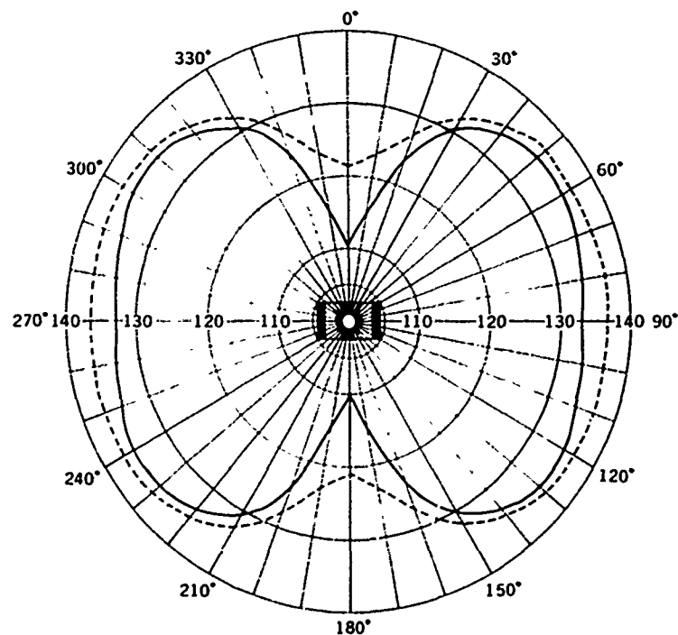
Figure 16. Vertical directivity pattern for Cylinder B at 6,000 Hz. Solid line is for experiment and dashed line for theory. Pressures are plotted in dB re 1 \mu\text{Pa} for 1 V input at 1 m.
