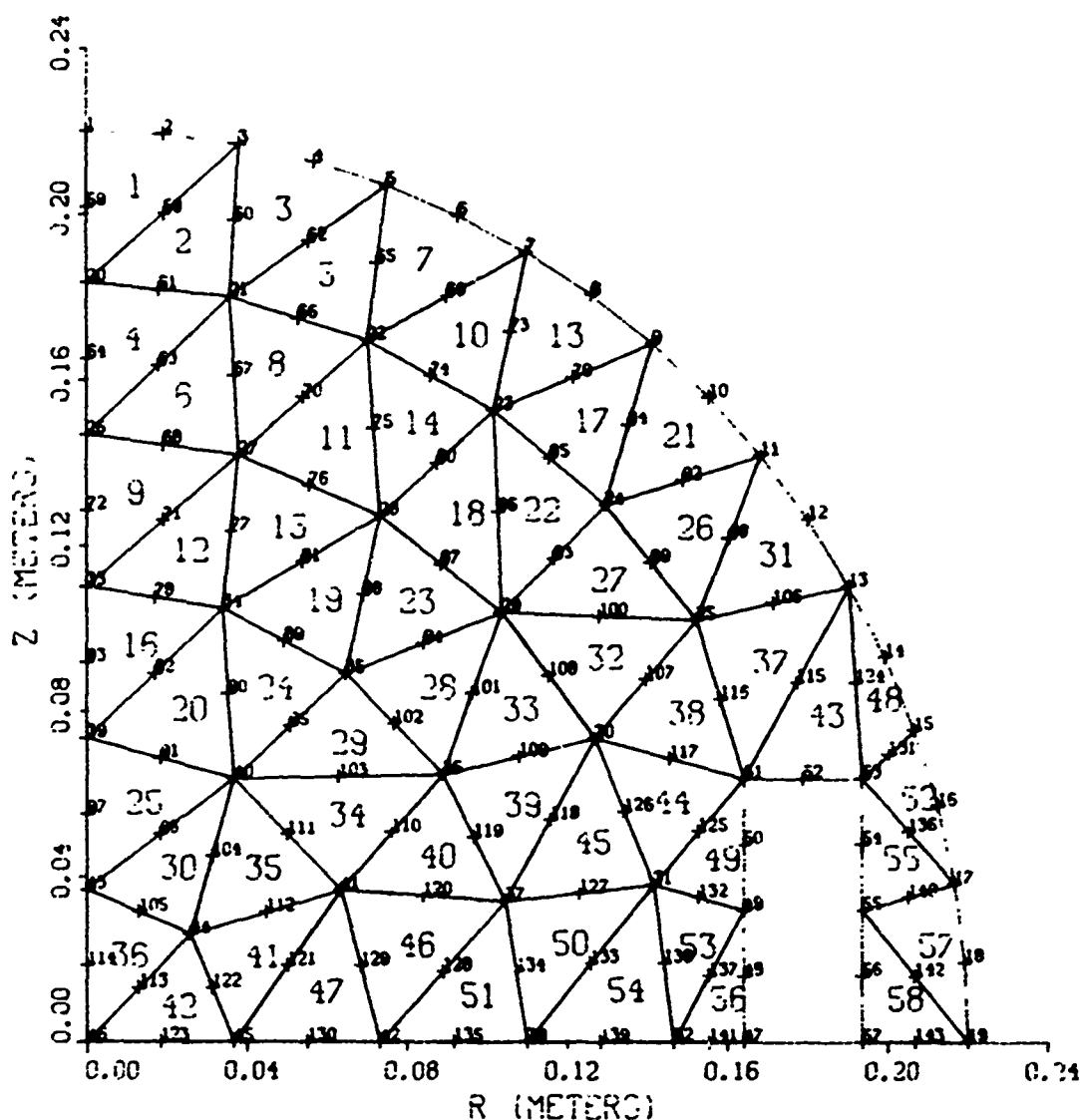
Figure 6. Cross-sectional display of the finite-element idealization of the top half of the acoustic fluid sphere that encloses the cylinder.
