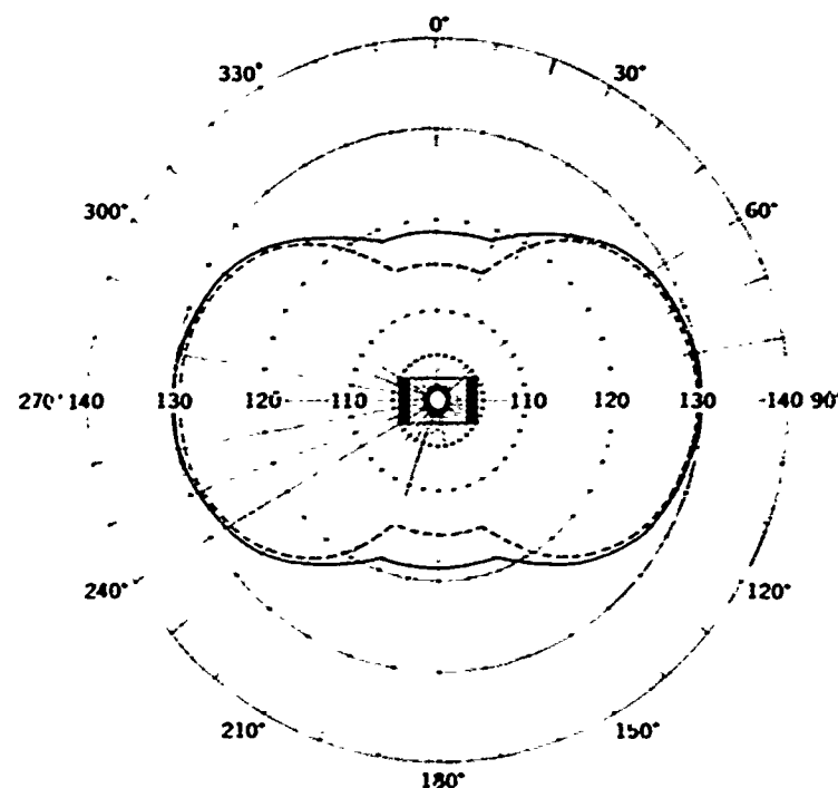
Figure 19. Vertical directivity pattern for Cylinder Cat at 4,000 Hz. Solid line is for experiment and dashed line for theory. Pressures are plotted in dB re 1 \mu\text{Pa} for 1 V input at 1 m.
