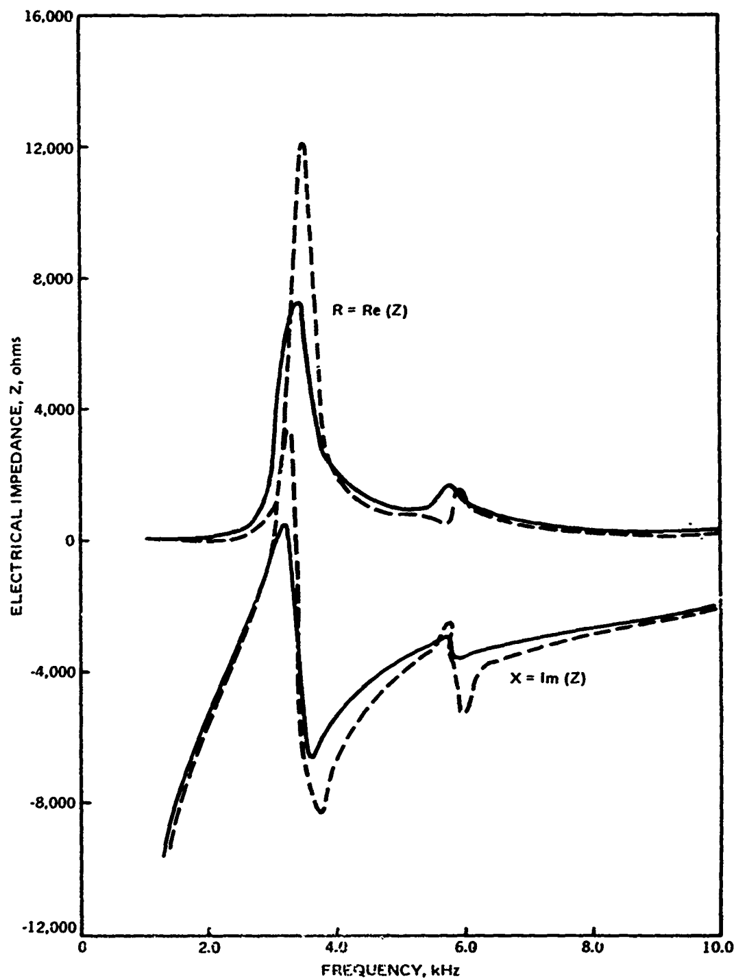
Figure 17. In-water complex electrical impedance for Cylinder C as a function of frequency. Solid lines are for experiment and dashed lines for theory.
