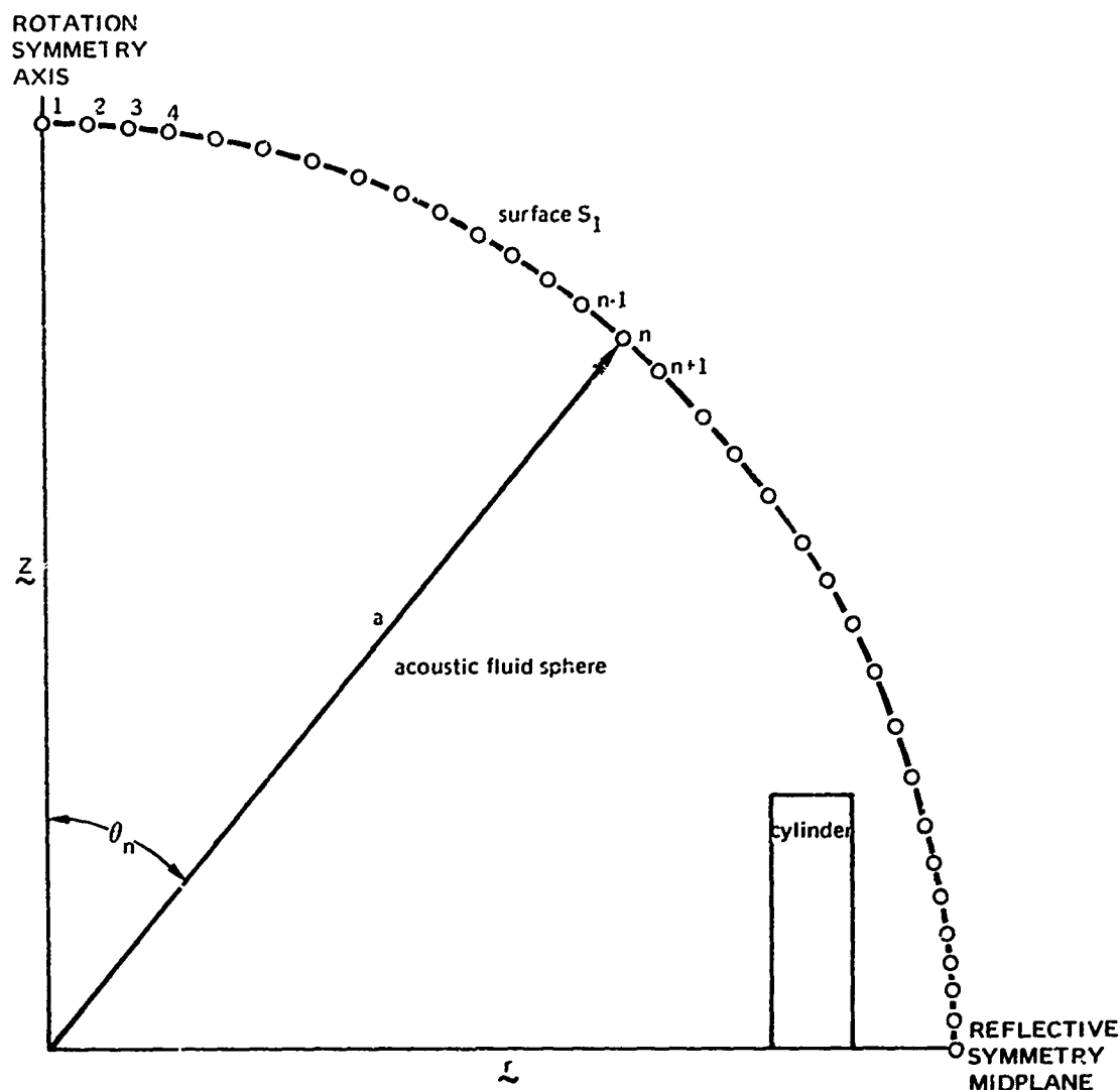
Figure 5. Cross-sectional drawing of the cylinder and fluid sphere surface showing the rotational symmetry axis and reflective symmetry midplane.
