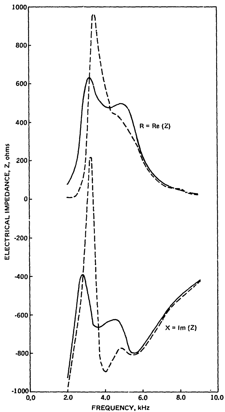
Figure 13. In-water complex electrical impedance of Cylinder B as a function of frequency. Solid lines are for experiment and dashed lines for theory.
