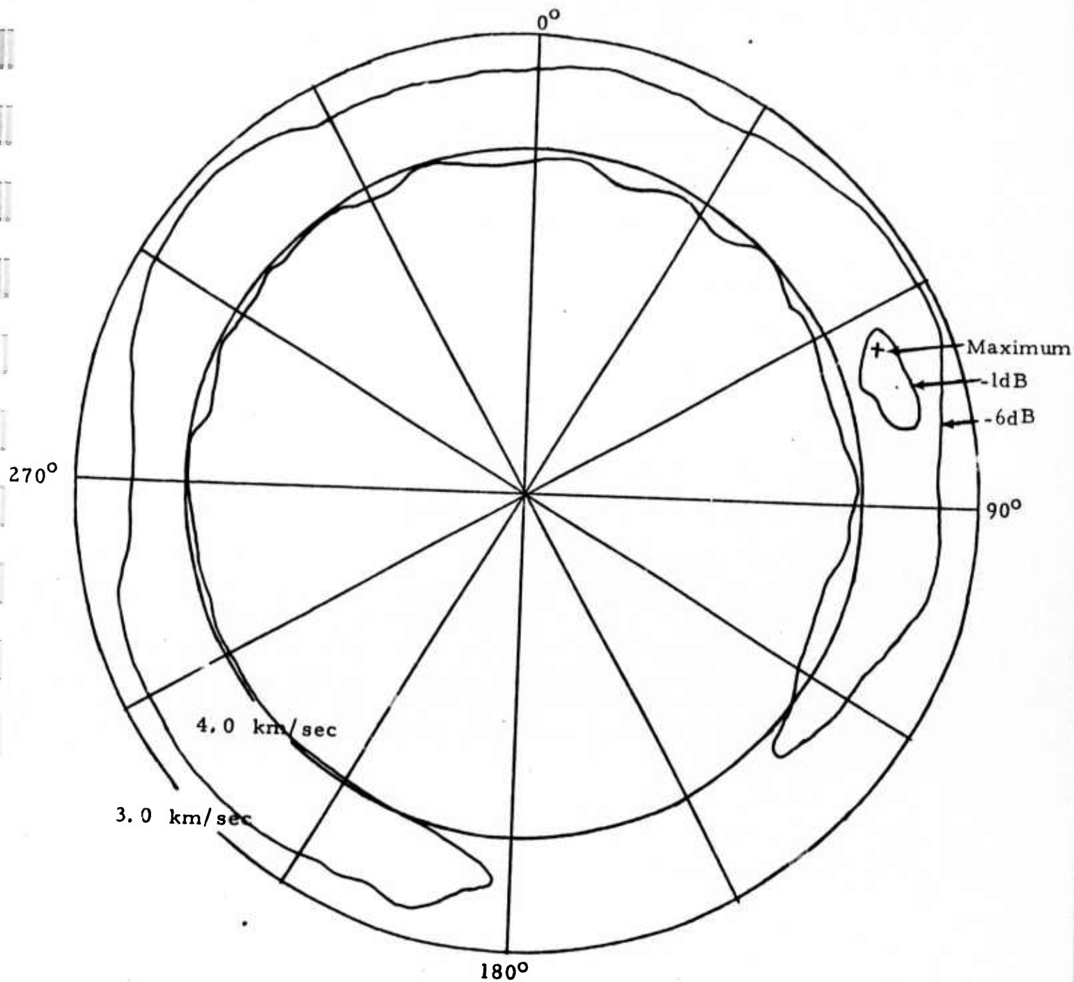
FIGURE III - 10 HIGH RESOLUTION F-K SPECTRA OF NOISE FROM 23 JULY 1972 AT 0.06 Hz
