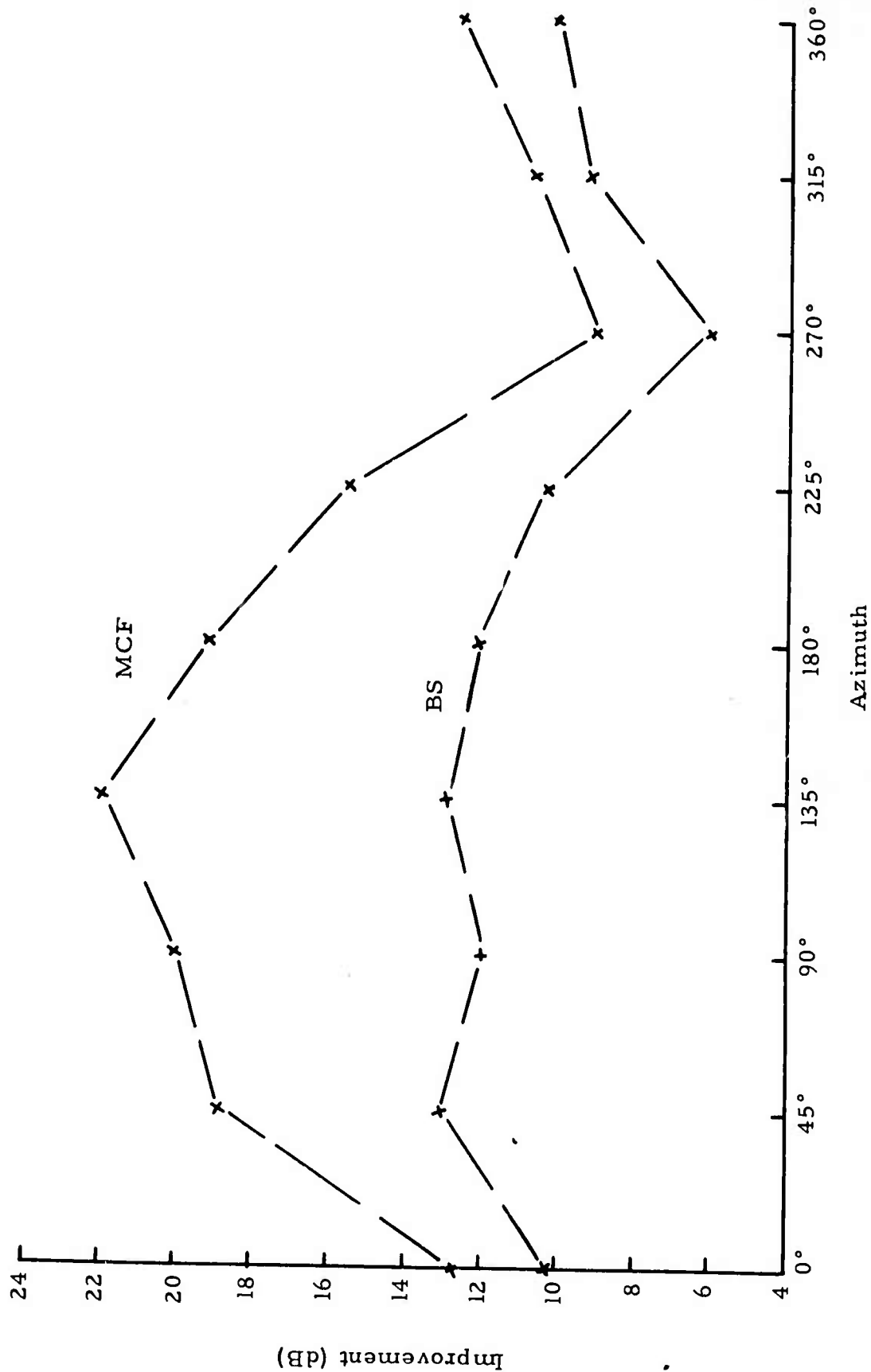
FIGURE IV-6 IMPROVEMENT vs. AZIMUTH FOR MCF AND BS PROCESSORS 0.02-0.10 Hz, On-Design Noise, Day 019, 1972
