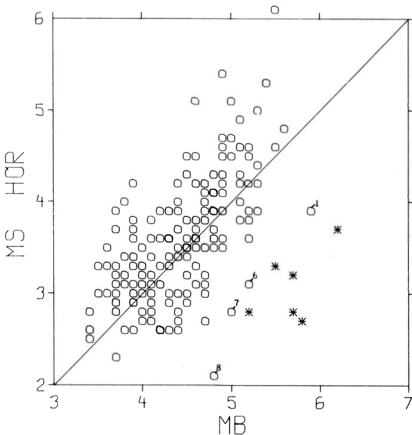
FIGURE VII-2 M_s VS. m_b DISCRIMINANT 1972 EVENTS
