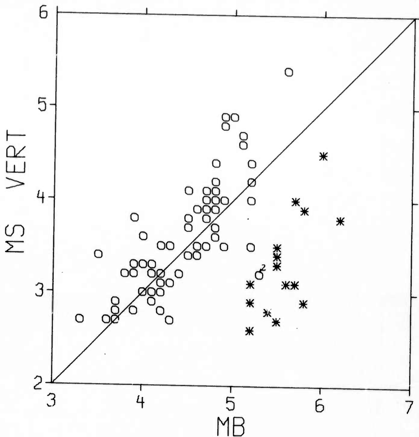
FIGURE VII-3 M_s VS. m_b DISCRIMINANT KURILE, KAMCHATKA AND OKHOTSK EVENTS
