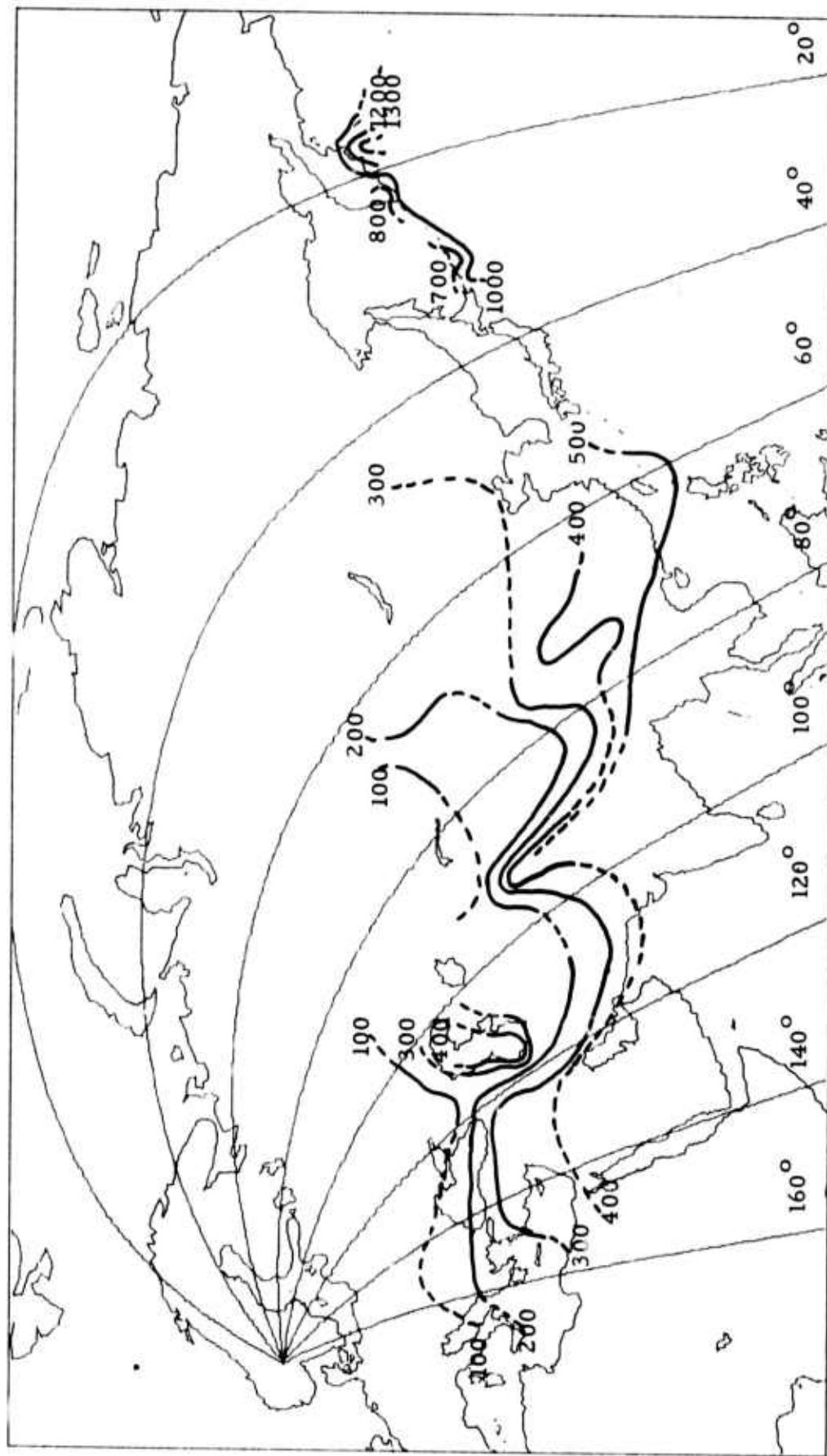
FIGURE V-2 OPTIMUM CHIRP FILTER LENGTHS (IN SECONDS) FOR RAYLEIGH WAVES AT NORSAR FOR THE PASSBAND 0.025 - 0.059 Hz
