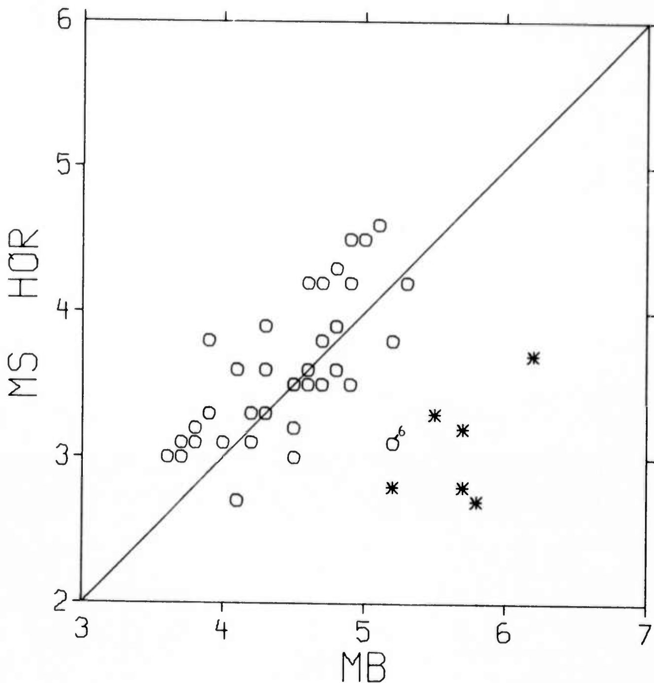
FIGURE VII-4 M_s VS. m_b DISCRIMINANT KURILE, KAMCHATKA AND OKHOTSK EVENTS
