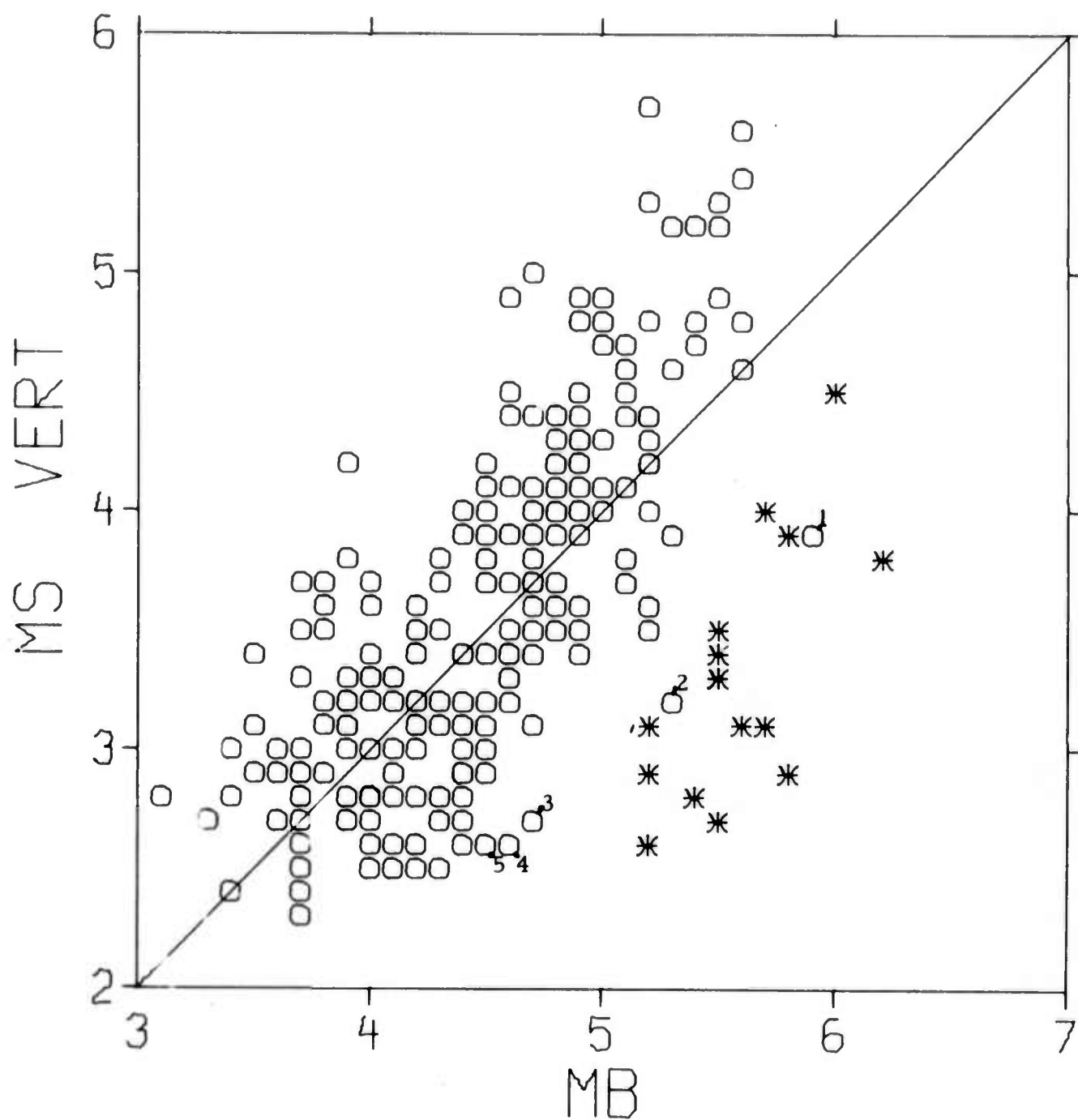
FIGURE VII-1 M_s VS. m_b DISCRIMINANT COMBINED 1971 AND 1972 EVENTS
