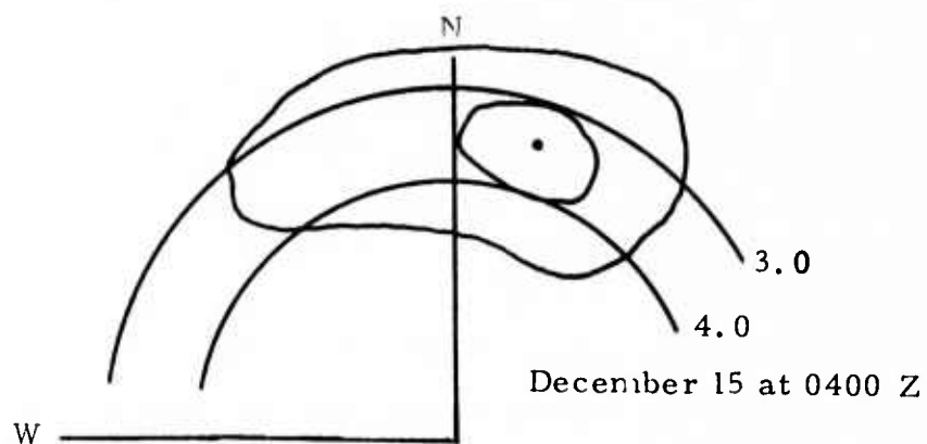
FIGURE III-4 HIGH RESOLUTION F-K SPECTRA POWER LEVELS, 13, 14 AND 15 DECEMBER 1971 AT 0.06 Hz
