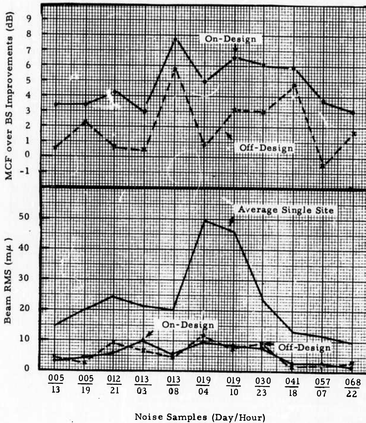
FIGURE IV-2 PROFILES OF ARRAY GAINS (0.025-0.059 Hz)
