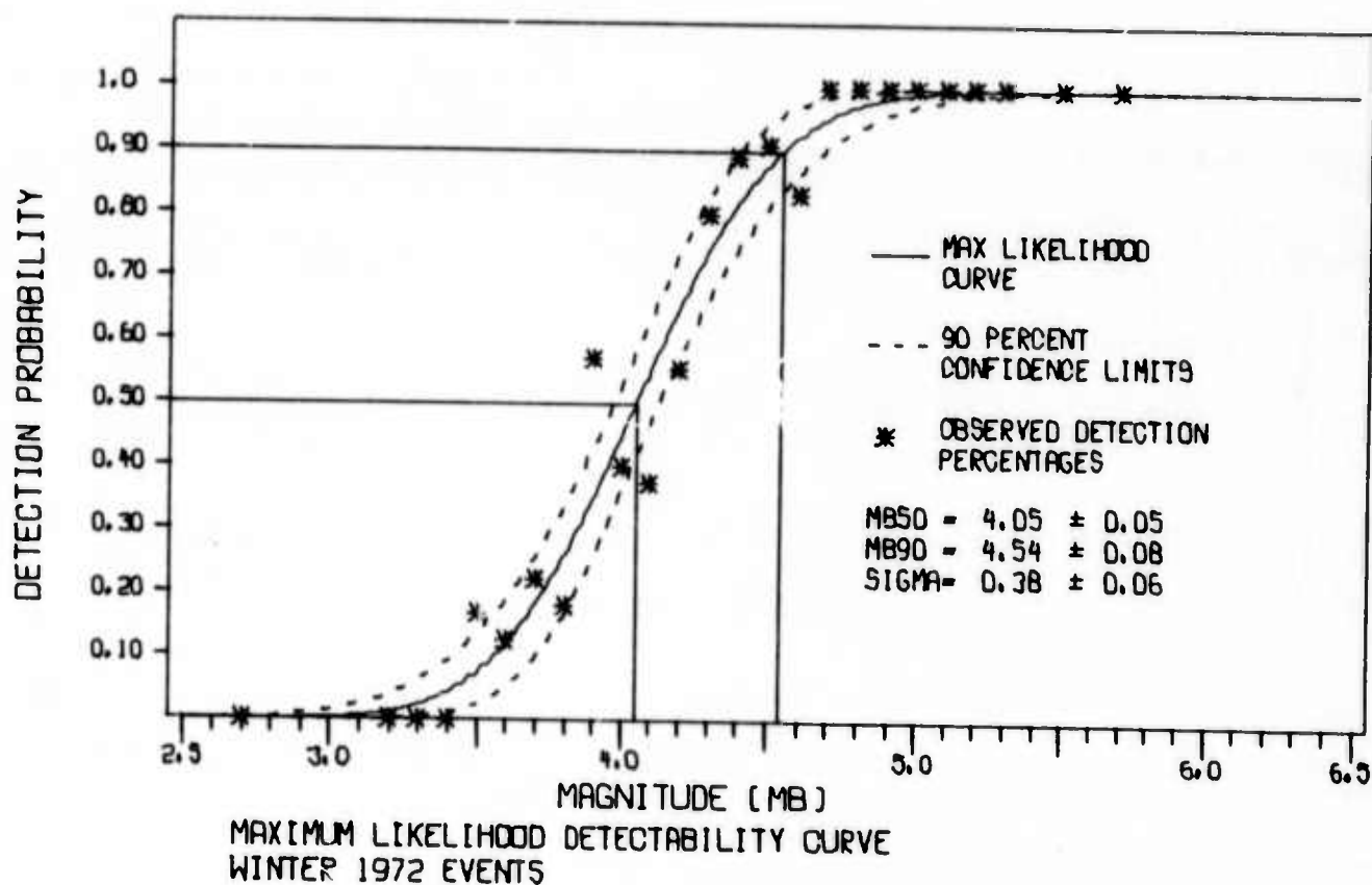
FIGURE VI-5 NORSAR L P SURFACE WAVE DETECTION STATISTICS FOR THE 1972 WINTER EVENTS
