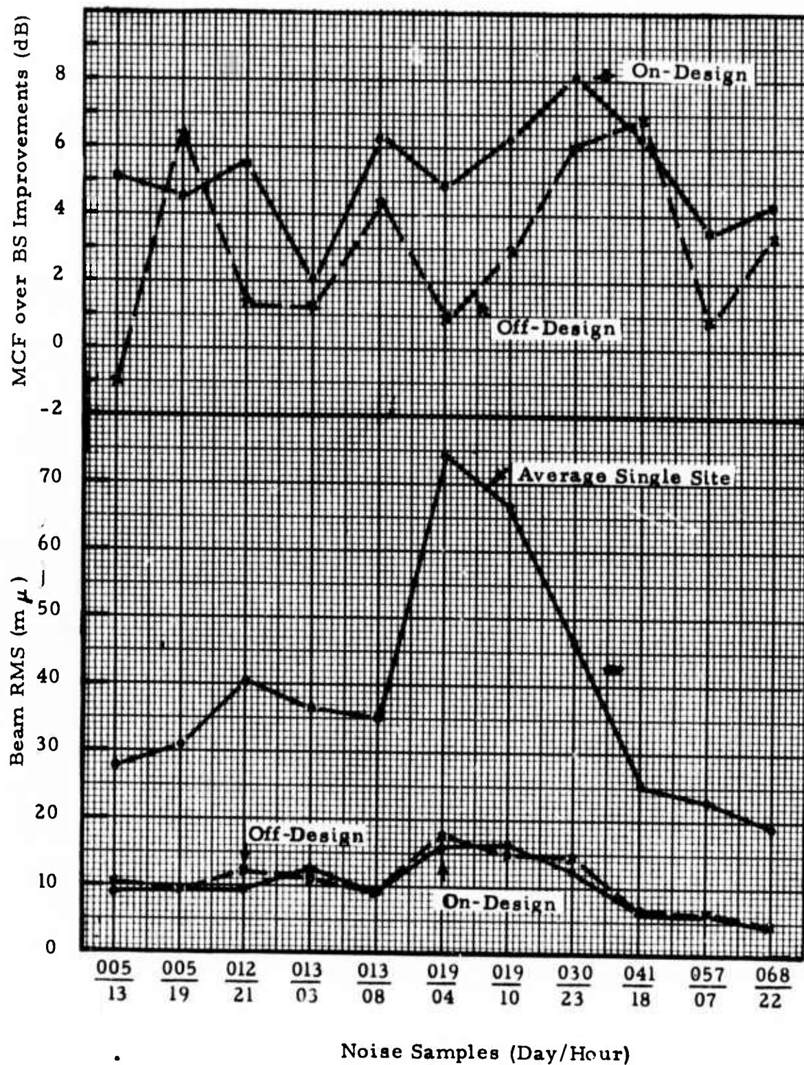
FIGURE IV-3 PROFILES OF ARRAY GAINS (0.02-0.10 Hz)
