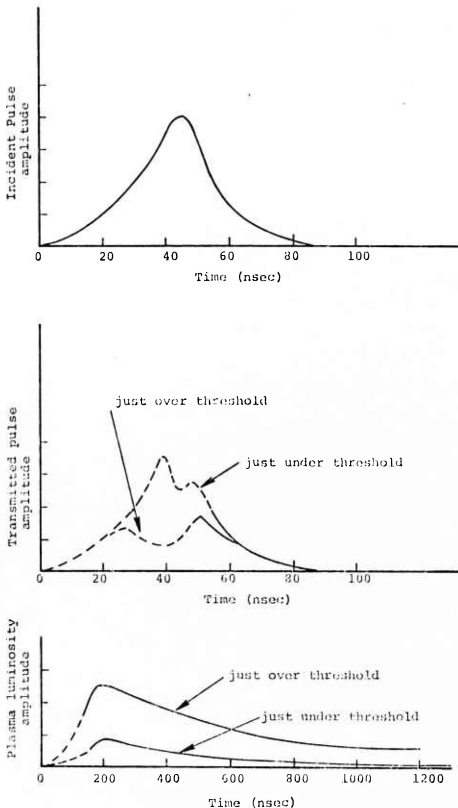
Figure 20. A plot of the incident and transmitted laser pulse with a 68\mu carbon fiber located at the focus. Also shown is the emission from the breakdown plasma.
