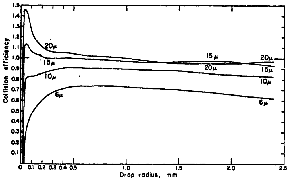
Figure 8. Collision Efficiencies. Collecting-drop radii are indicated on the abscissa. Radii of the collected droplets are indicated by the curves. [3]
