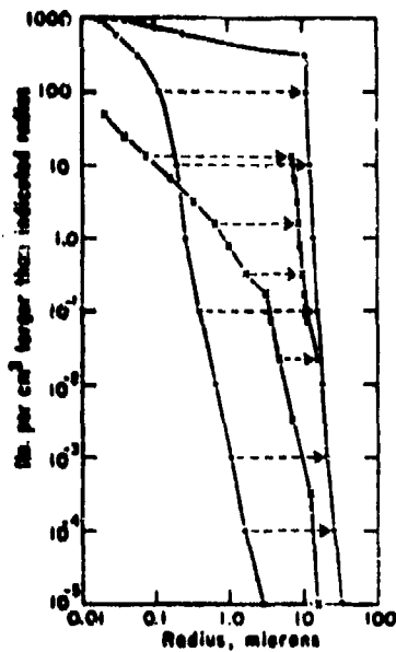
Figure 6. Initial and Final Distributions of Particle and Droplet Sizes as Computed by Mordy (1959) (points marked x) and by Weiburger and Chien (1960) (points with heavy dots). The dashed arrows connect initial with final sizes. (from Byers [3])
