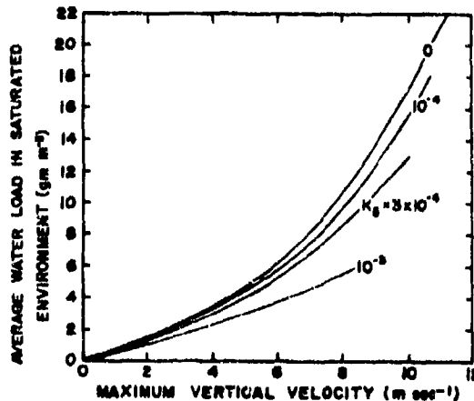
Figure 2. Average Liquid Water Content in a Vertical Column 10 Km High, in Relation to the Maximum Vertical Air Speed and Mixing Rate K_5 . The diagram applies to steady state conditions in saturated model updraft columns in saturated environments [11].
