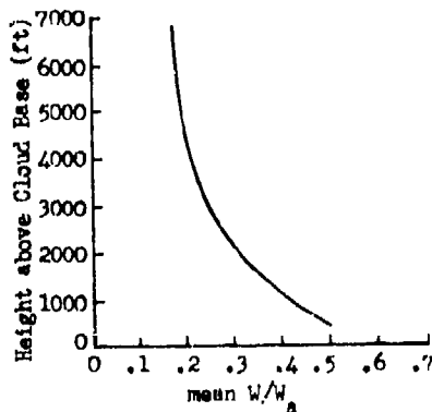
Figure 3b. Mean Ratio W/W_a versus Height above Base. [22]
