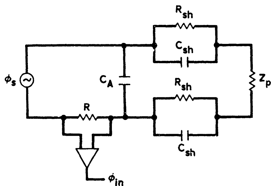
Fig. 51. Equivalent circuit for the linear sheath model of the dual-sphere electric antenna.
