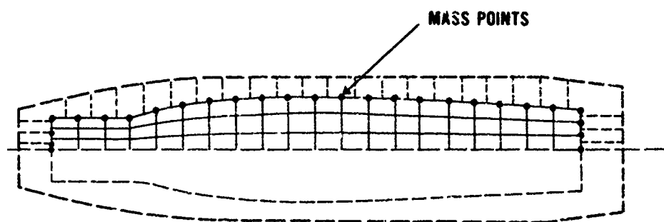
FIG. 1 COMPUTATION GRID
