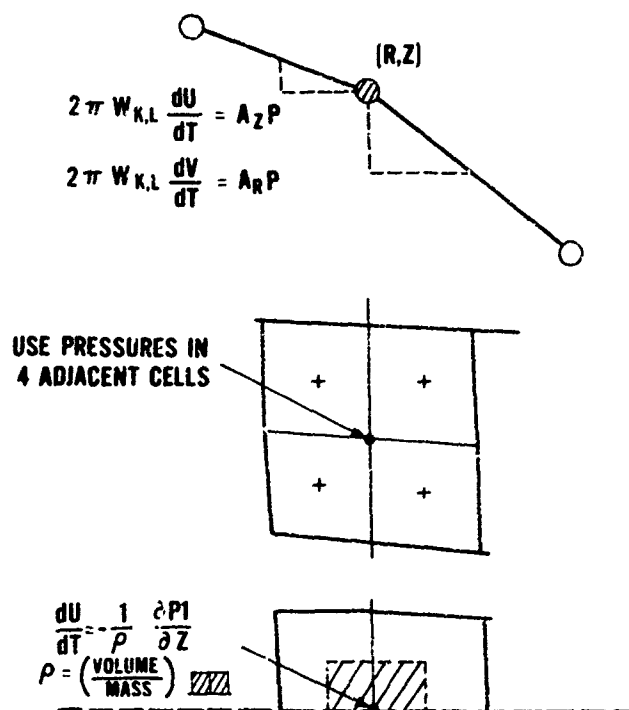
FIG. 8 VELOCITY CALCULATIONS
