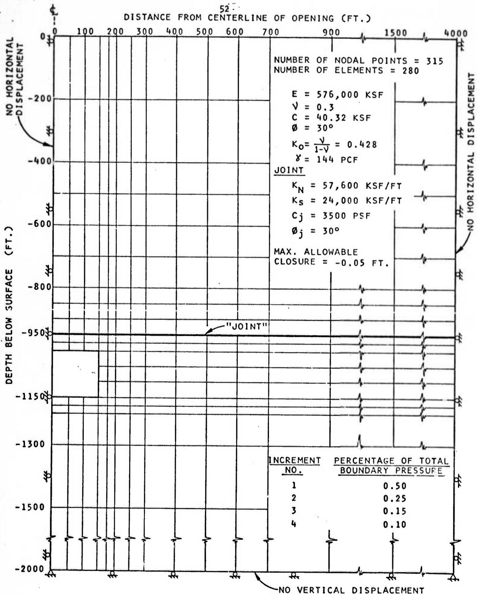
FIG. I-7 - FINITE ELEMENT MESH FOR ANALYSIS OF A RECTANGULAR OPENING
