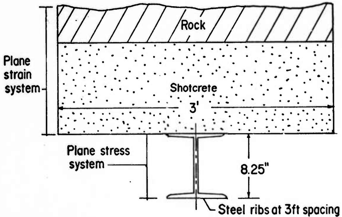
(b) Representative Slice.
