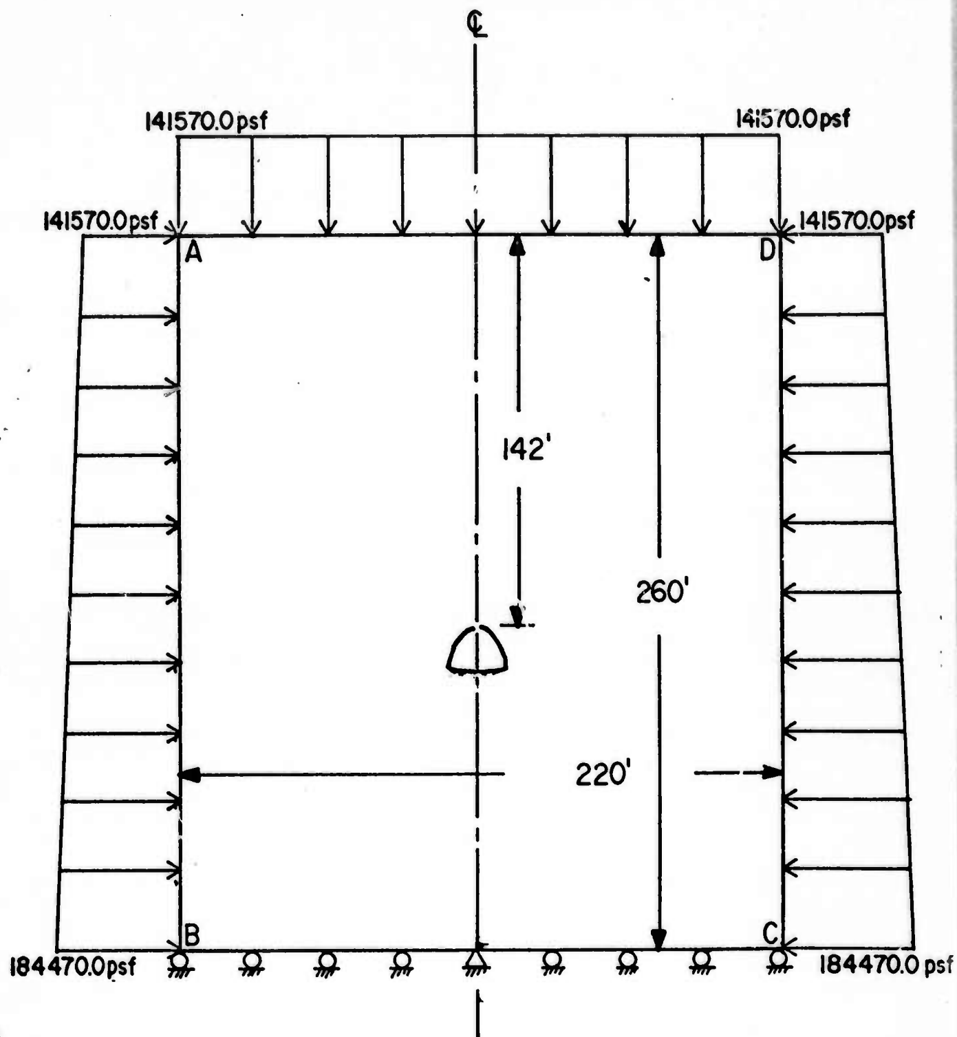
FIGURE 2. - Boundary Conditions on the Finite Element Model.
