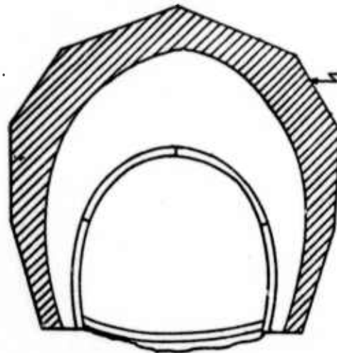
(b) Tunnel Cross-Section Showing Rock Load for Case b.
