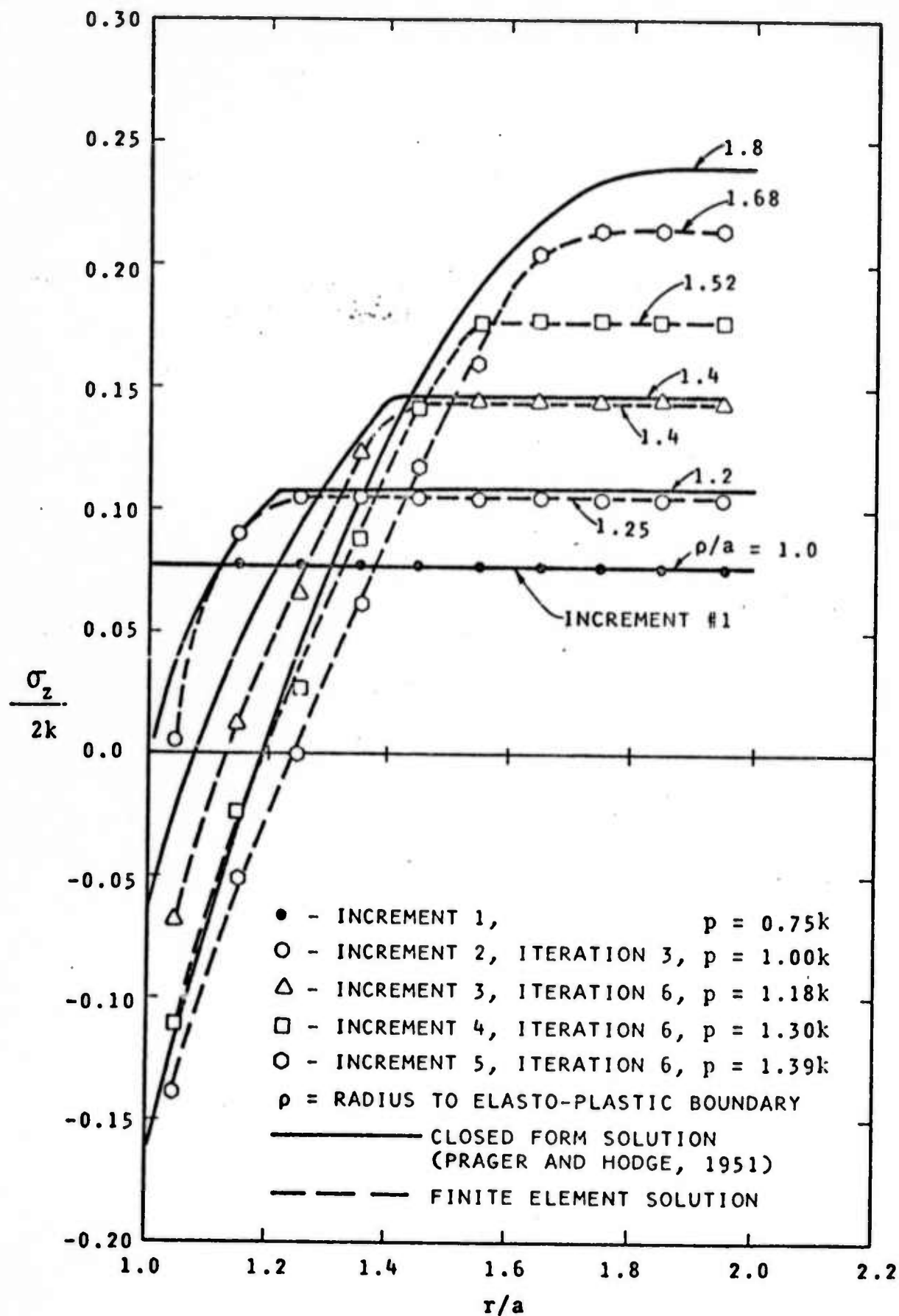
FIG. I-3 - DISTRIBUTION OF AXIAL STRESS FOR A THICK-WALLED CIRCULAR TUBE
