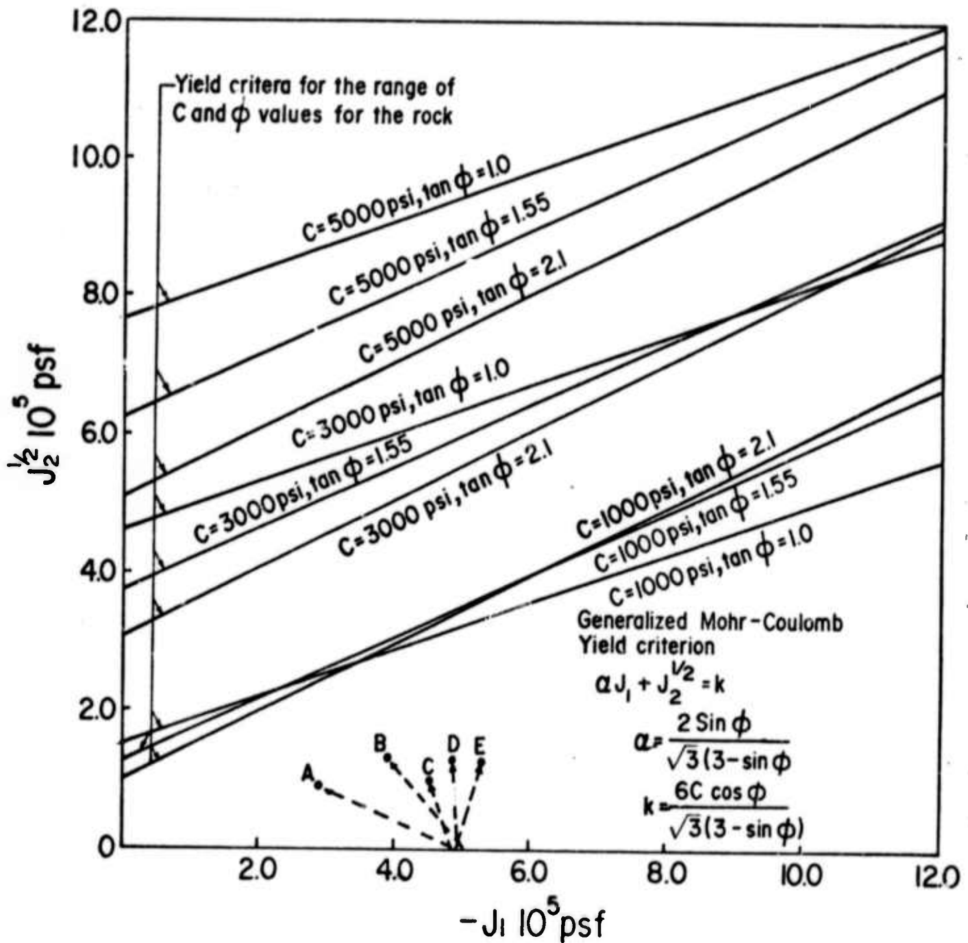
FIGURE 6. - Stress Paths for Points Around the Underground Opening (for location of points see FIG. 5).
