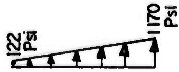
FIGURE 11. - Longitudinal Stress Distribution at Critical Sections (Reduction of E from 1.0 \times 10^6 to 0.4 \times 10^6 psi).
