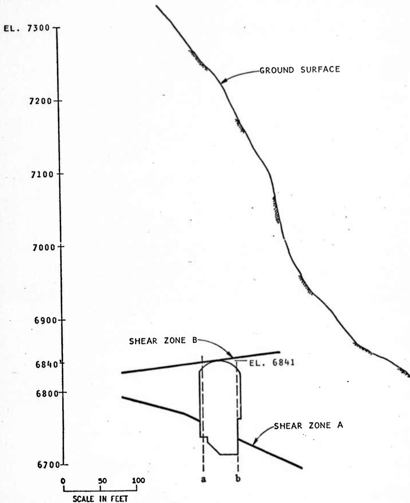
FIG. 12 - CROSS-SECTION A-A' (LINE 4 + 12 FT) OF THE POWERPLANT CHAMBER, MORROW POINT POWERPLANT
