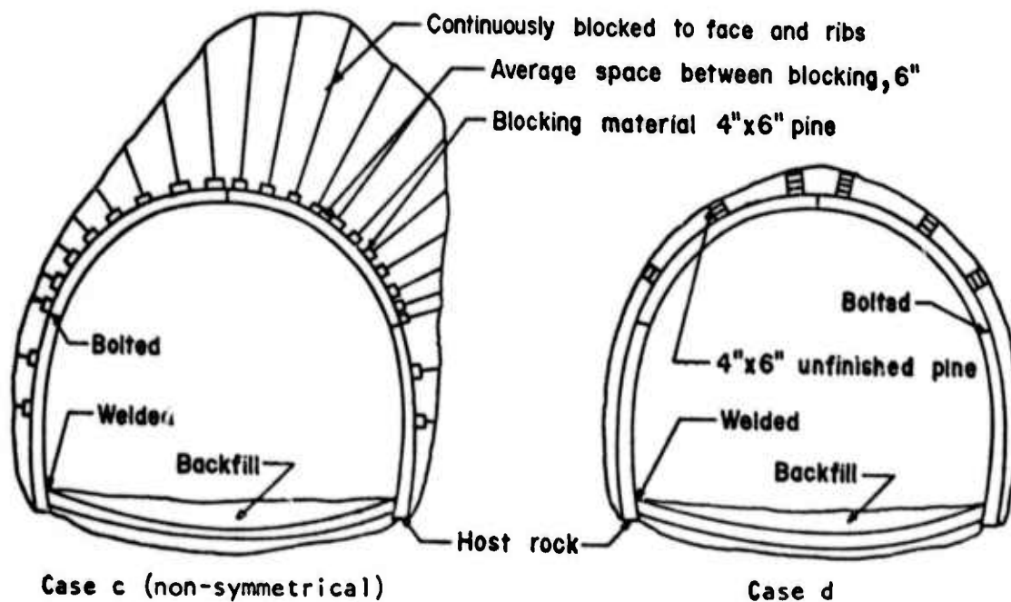
FIGURE 1. - Tunnel Excavation and Support Blocking Configuration.
