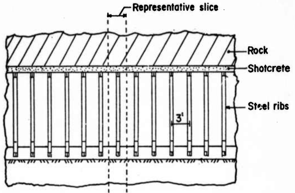
(a) Longitudinal Cross-Section of Tunnel.
