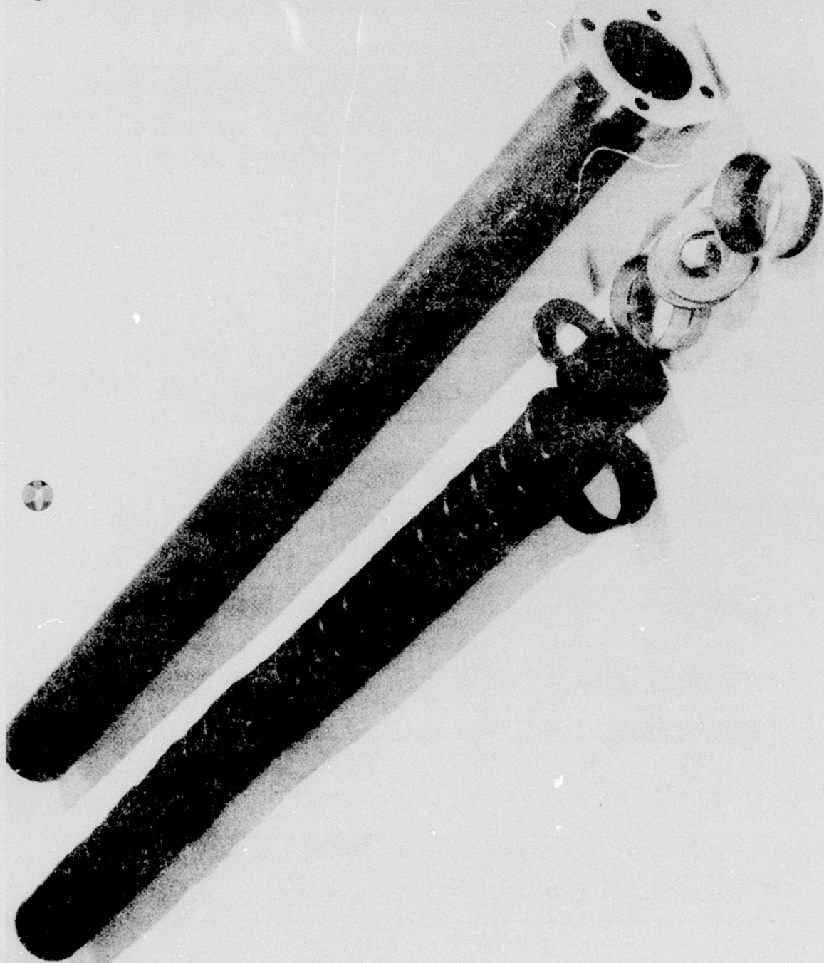
Figure 24. Muffler Model, Configuration 045, Showing Arrangement of 2-1/8-inch OD Washers and Spacer Rings in 32-inch Housing
