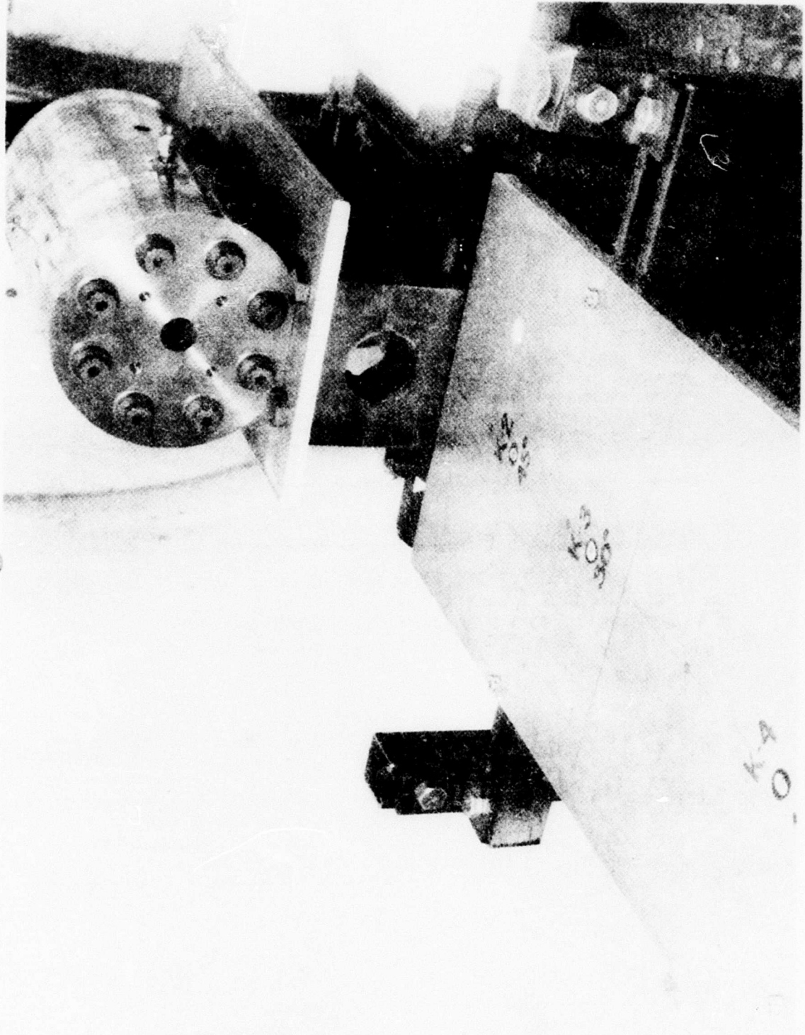
Figure 36. Installation of Shock-Tube Cylinder in Gun Firing Range Tunnel (transducer positions are indicated on surface plate)
