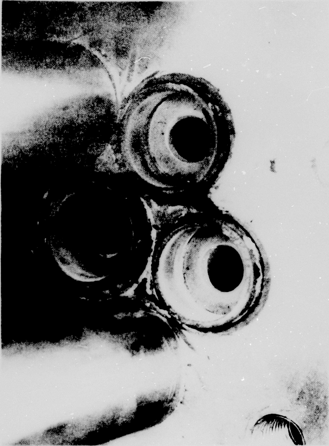
Figure 47. Photograph of Seven-Tube Suppressor After Firing with Gun Propellants (three tubes are removed showing first washer and spacer exposed to multinozzle jet discharge)
