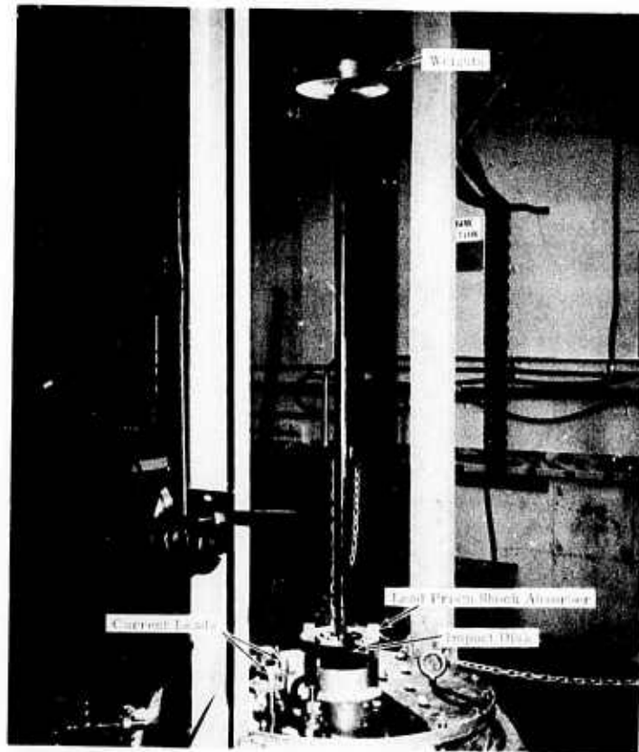
Figure 3. Test Apparatus for Exciting Linear Shocks
