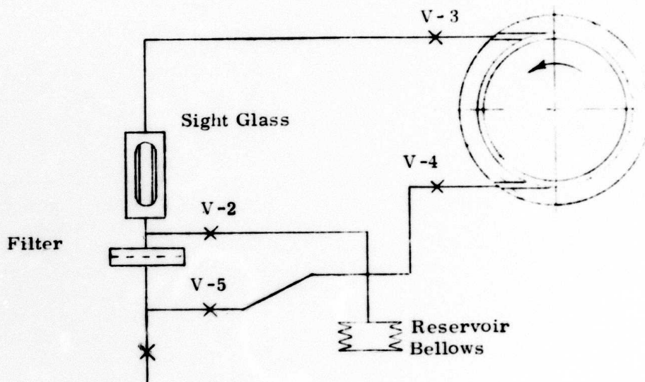
Figure 42. Gallium Handling System
