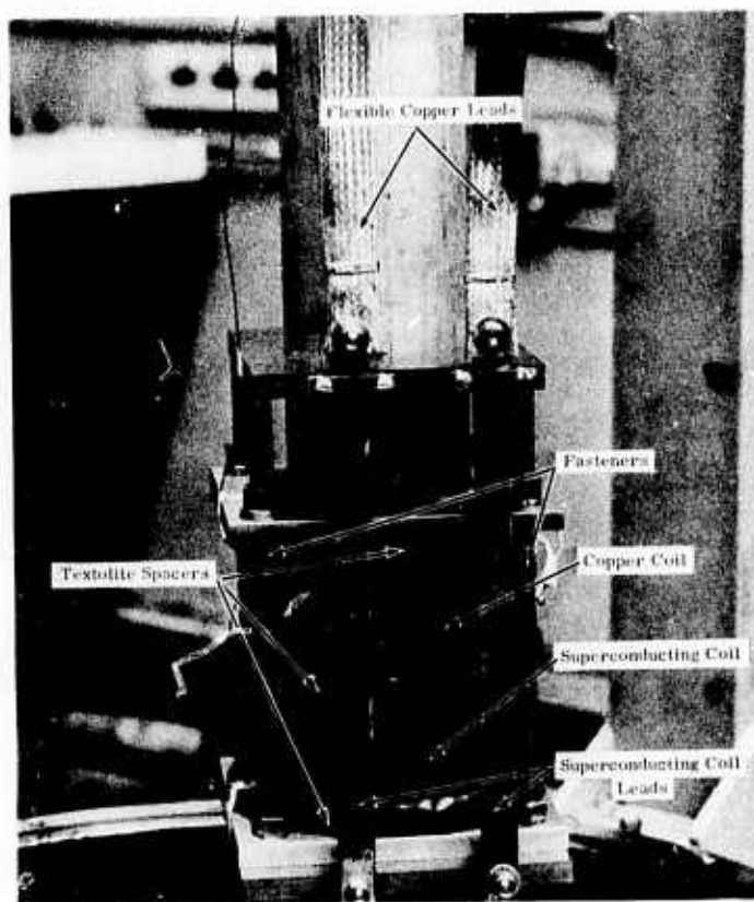
Figure 8. Coil Assembly with Principal Axis Vertical
