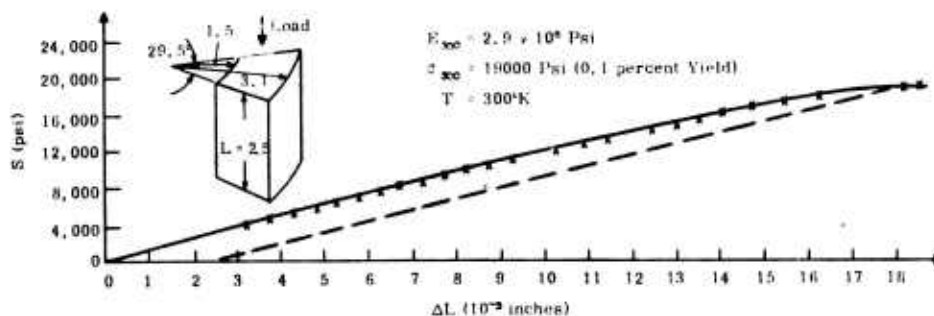
Figure 33. Stress Versus Contraction for Axially Compressed Coil Specimens at 300°K
