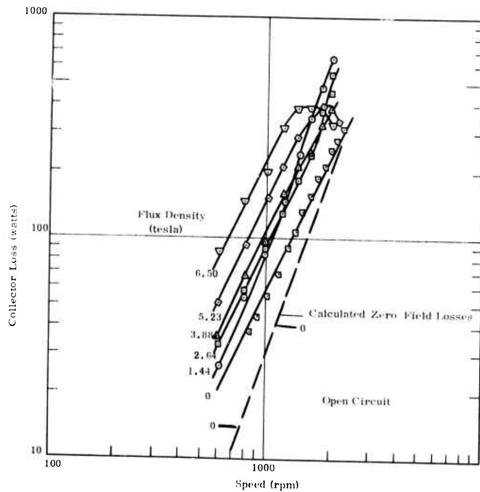
Figure 46. Open Circuit Collector Loss
