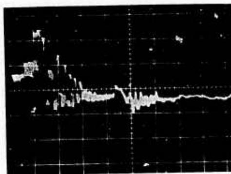
Test 5 -- Oscilloscope Sensitivity = 2140 g/cm Vertically and 0.2 ms/cm Horizontally (SC is energized at 445 amperes and stays superconductive after the shock.)
