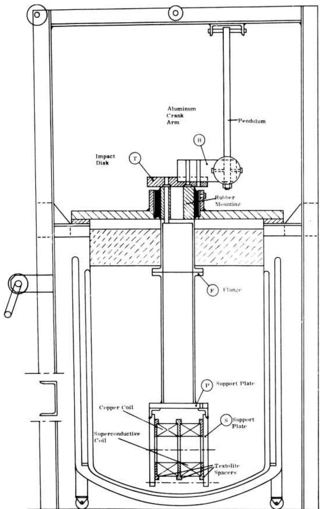
Figure 2. Apparatus Setup for Torsional Shock Test Applications
