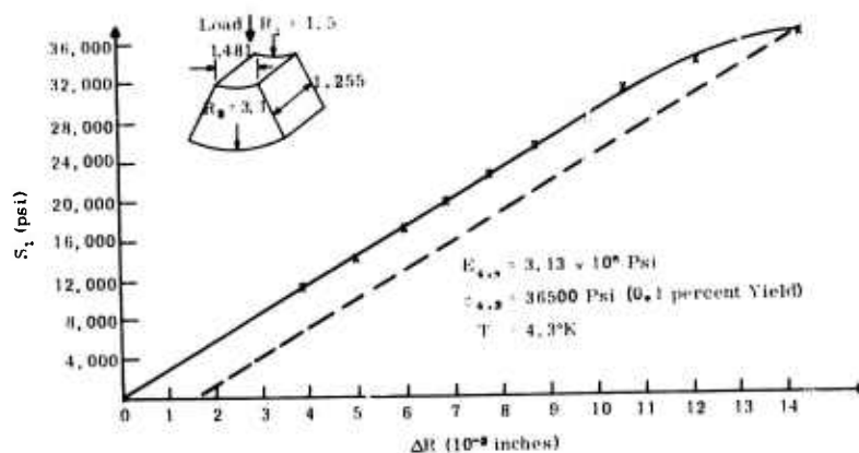
Figure 32. Bore Stress Versus Contraction for Radially Compressed Coil Specimens at 4.3°K
