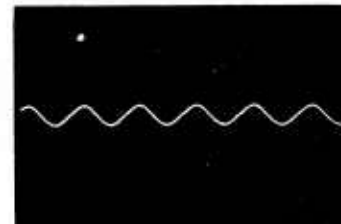
Output Voltage of Test Accelerometer with Shunt Capacitance of 0.0033 mF at 5-g Acceleration and 1000-Hertz Frequency (Oscilloscope sensitivity is 0.2 V/cm vertically and 0.2 ms/cm horizontally.)
