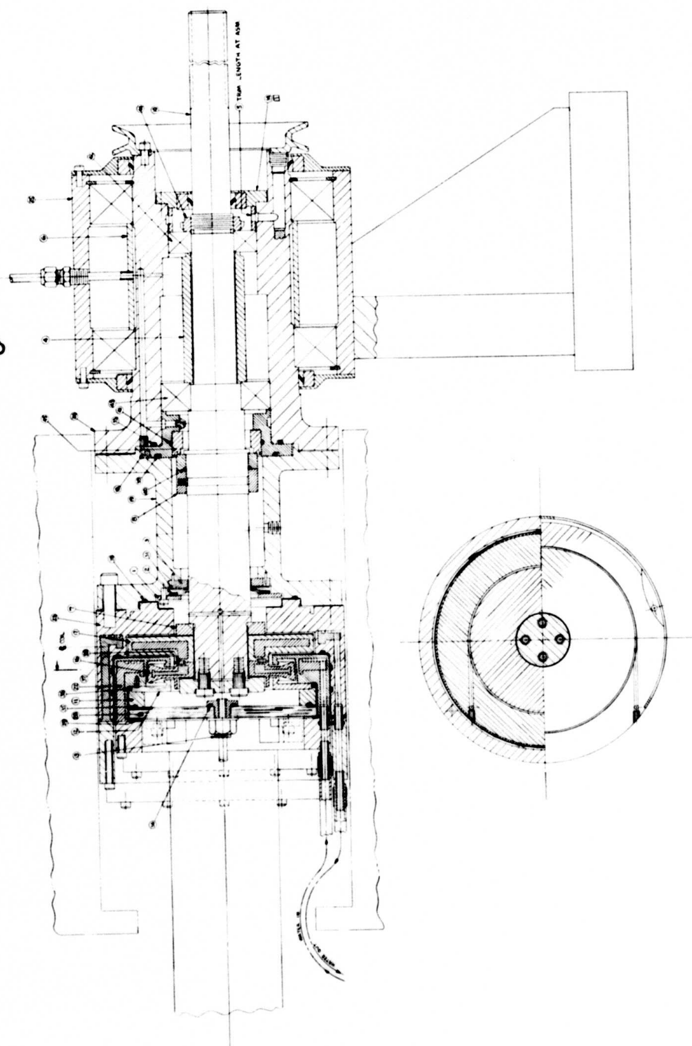
Figure 35. Current Collector Cross Section
