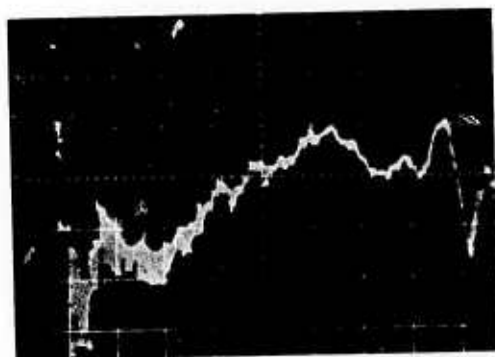
Test 1 -- Oscilloscope Sensitivity = 214 g/cm Vertically and 0.5 ms/cm Horizontally (SC is energized at 300 amperes and remains superconducting after the shock.)
