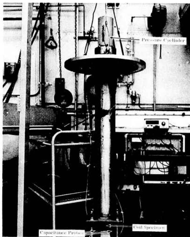
Figure 29. Test Apparatus and Instrumentation for Coil Composite Strength Experiments
