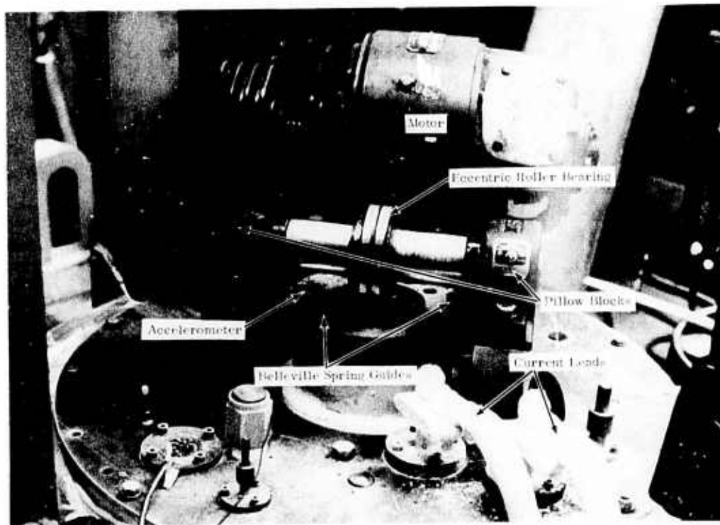
Figure 5. Vibrator Assembly for Linear Vibration Applications
