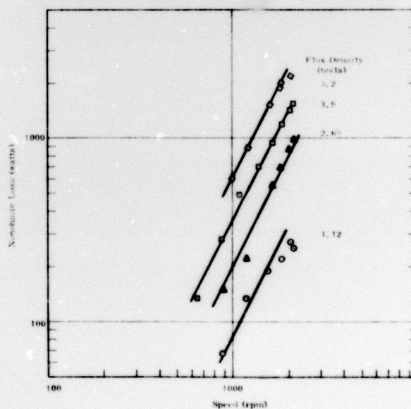
Figure 50. Collector Loss ( R_{Load} = 220 \mu\Omega )
