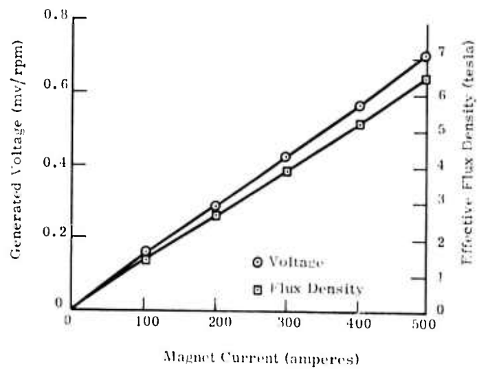
Figure 45. Open Circuit Voltage
