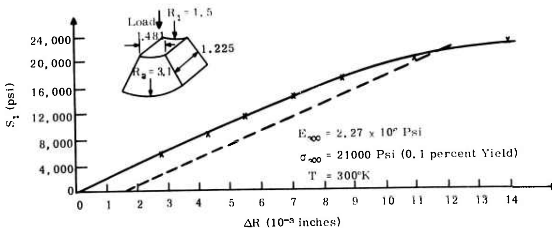
Figure 31. Bore Stress Versus Contraction for Radially Compressed Coil Specimens at Room Temperature (300° K)
