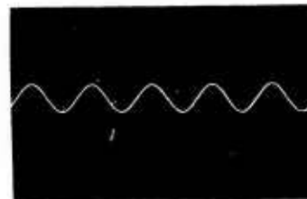
Output Voltage of Test Accelerometer with Shunt Capacitance of 0.0033 mF at 40-g Acceleration and 100-Hertz Frequency (Oscilloscope sensitivity is 1 V/cm vertically and 5 ms/cm horizontally.)
