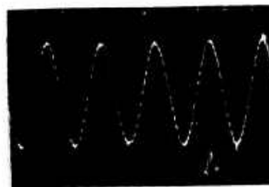
Test Accelerometer Output at 10-g Acceleration 100-Hertz Frequency (Oscilloscope sensitivity is 4.0 V/cm vertically and 5 ms/cm horizontally.)
