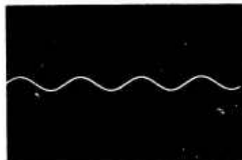
Output Voltage of Test Accelerometer with Shunt Capacitance of 0.0033 mF at 5-g Acceleration and 2000-Hertz Frequency (Oscilloscope sensitivity is 0.2 V/cm vertically and 0.2 ms/cm horizontally.)
