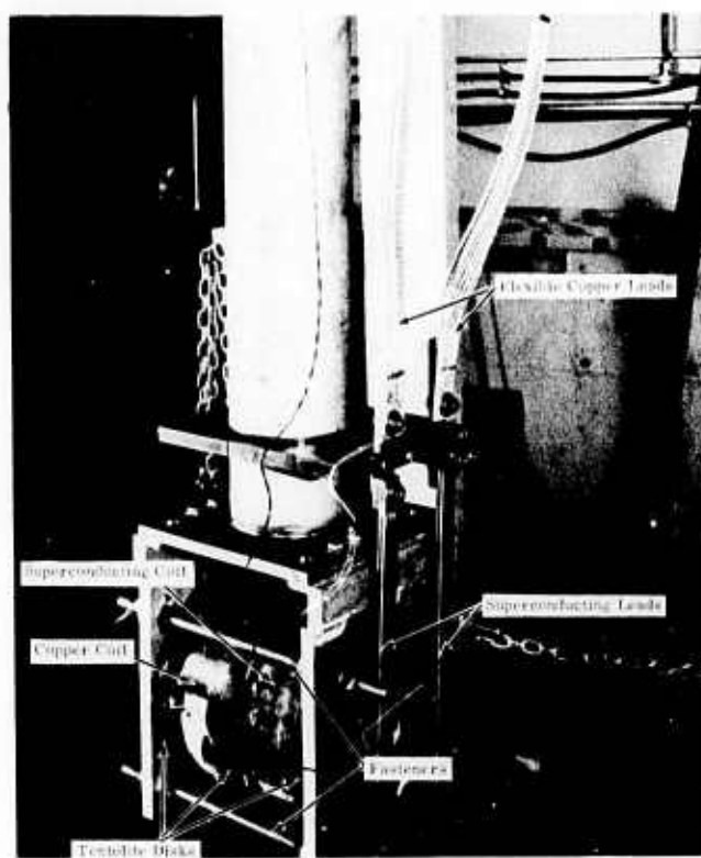
Figure 10. Coil Assembly with Principal Axis Horizontal
