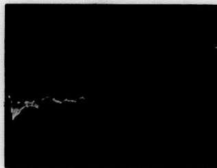
Test 3 -- Oscilloscope Sensitivity = 856 g/cm Vertically and 0.5 ms/cm Horizontally (SC is energized at 420 amperes and it remained superconductive after the shock.)
