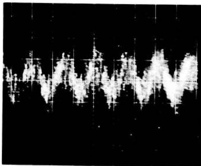
Figure 25. Accelerometer Output at 6-Inch Radius for Torsional Vibration Tests of Coils with Axis Horizontal (Oscilloscope sensitivity is 21.4 g/cm vertically and 10 ms/cm horizontally.)
