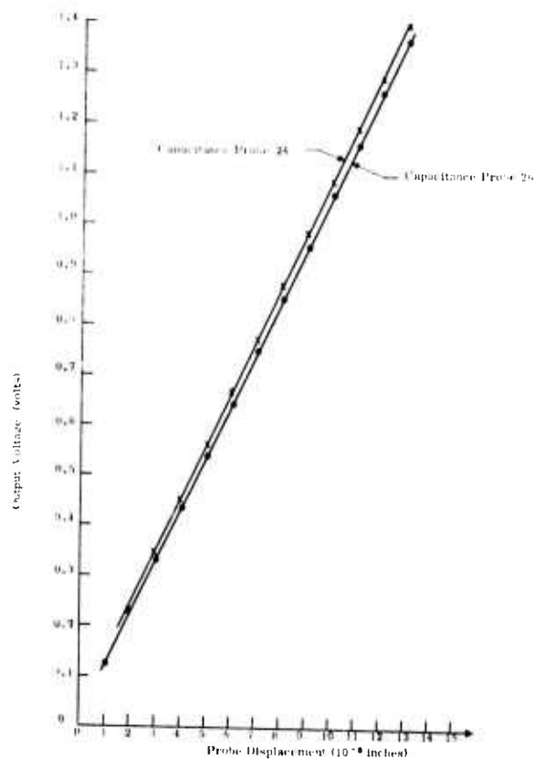
Figure 30. Calibration of Capacitance Probe Sensors in Micrometer Fixture
