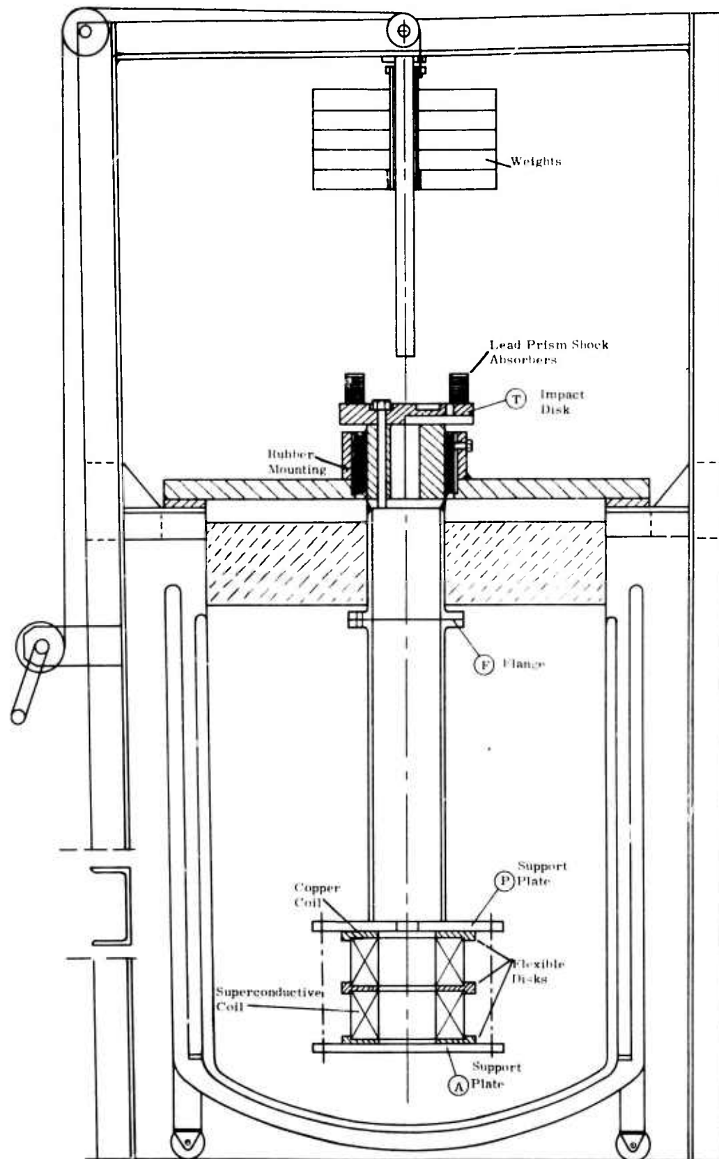
Figure 1. Apparatus Setup for Linear Shock Test Applications
