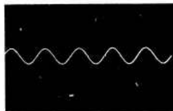
Output Voltage of Test Accelerometer with Shunt Capacitance of 0.0033 mF at 20-g Acceleration and 100 Hertz Frequency (Oscilloscope sensitivity is 0.5 V/cm vertically and 5 ms/cm horizontally.)
