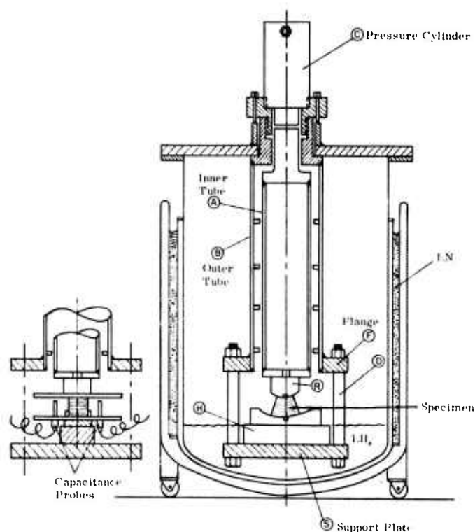
Figure 26. Test Apparatus Setup for Radial Compression Tests of Core Composite Specimens
