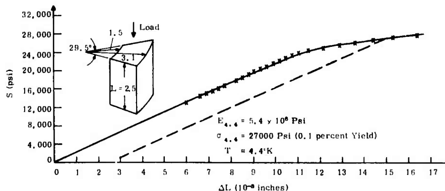
Figure 34. Stress Versus Contraction for Axially Compressed Coil Specimens at 4.4°K
