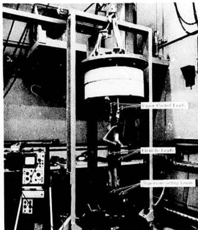
Figure 9. Overall Assembly of Coils, Leads, and Supports with Coil Axis Vertical
