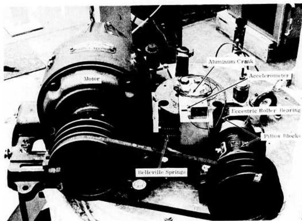
Figure 6. Vibrator Assembly for Torsional Vibration Applications
