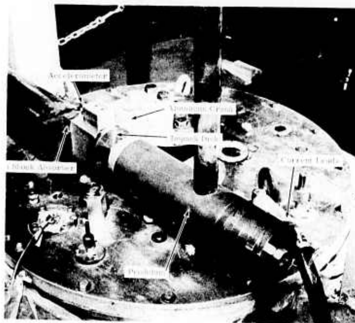
Figure 4. Test Apparatus for Exciting Torsional Shocks
