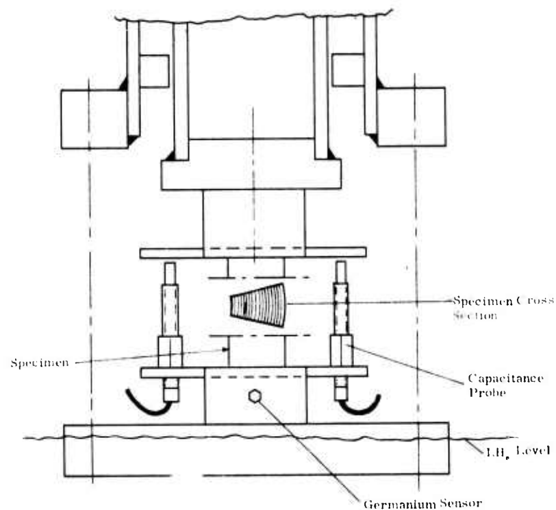
Figure 28. Arrangement for Testing Coil Composite Specimens in Axial Compression
