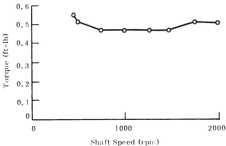
Figure 44. Bearing and Seal Torque
