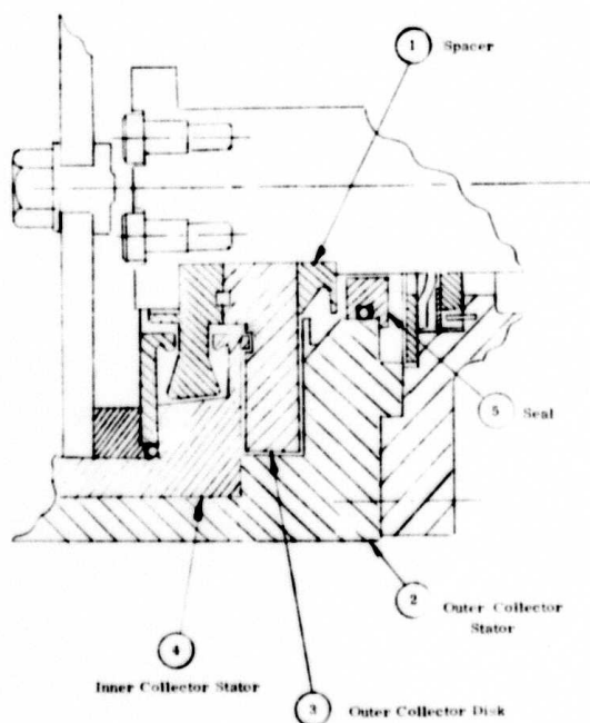
Figure 43. Test Assembly Modification
