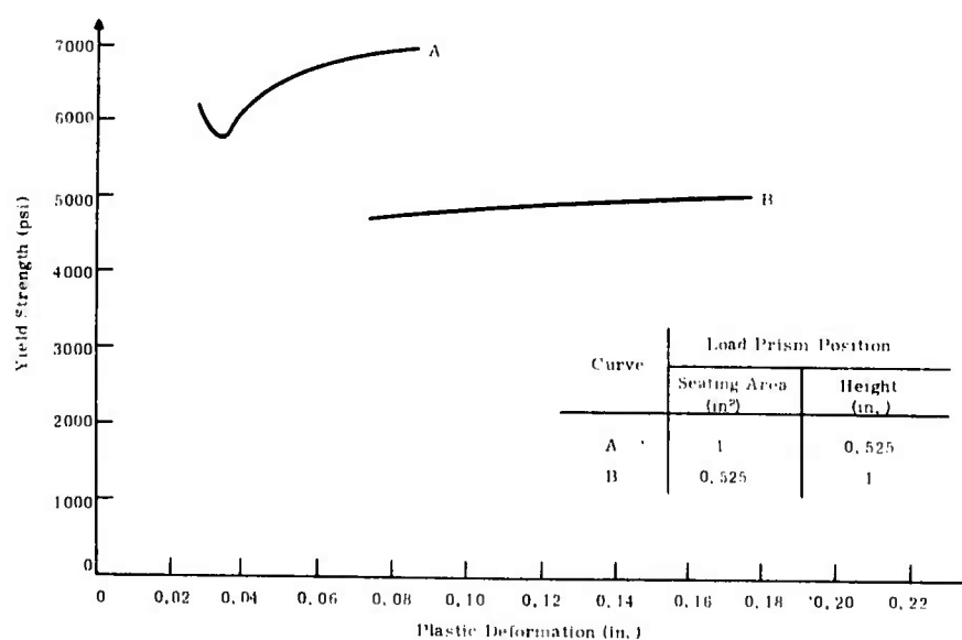
Figure 17. Average Yield Strength Versus Deformation for Lead Prisms (1 x 1 x 0.525 inch)
