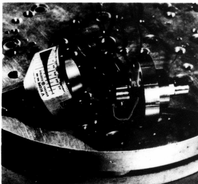
Figure 11. Test Accelerometer Mounted Back-to-Back with Standard Accelerometer for Dynamic Calibration
