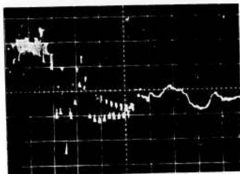
Test 4 -- Oscilloscope Sensitivity = 856 g/cm Vertically and 0.2 ms/cm Horizontally (SC is energized at 440 amperes and stays superconductive following the shock.)
