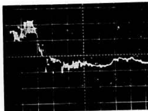
Test 3 -- Oscilloscope Sensitivity = 856 g/cm Vertically and 0.2 ms/cm Horizontally (SC is energized at 440 amperes and remains superconductive following the shock.)
