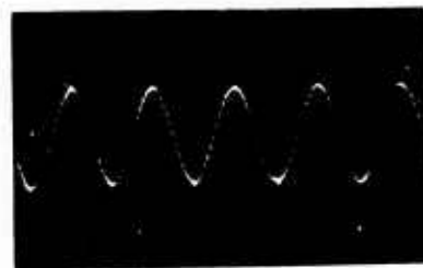
Test Accelerometer Output at 5-g Acceleration, 100-Hertz Frequency (Oscilloscope sensitivity is 0.2 V/cm vertically and 5 ms/cm horizontally.)
