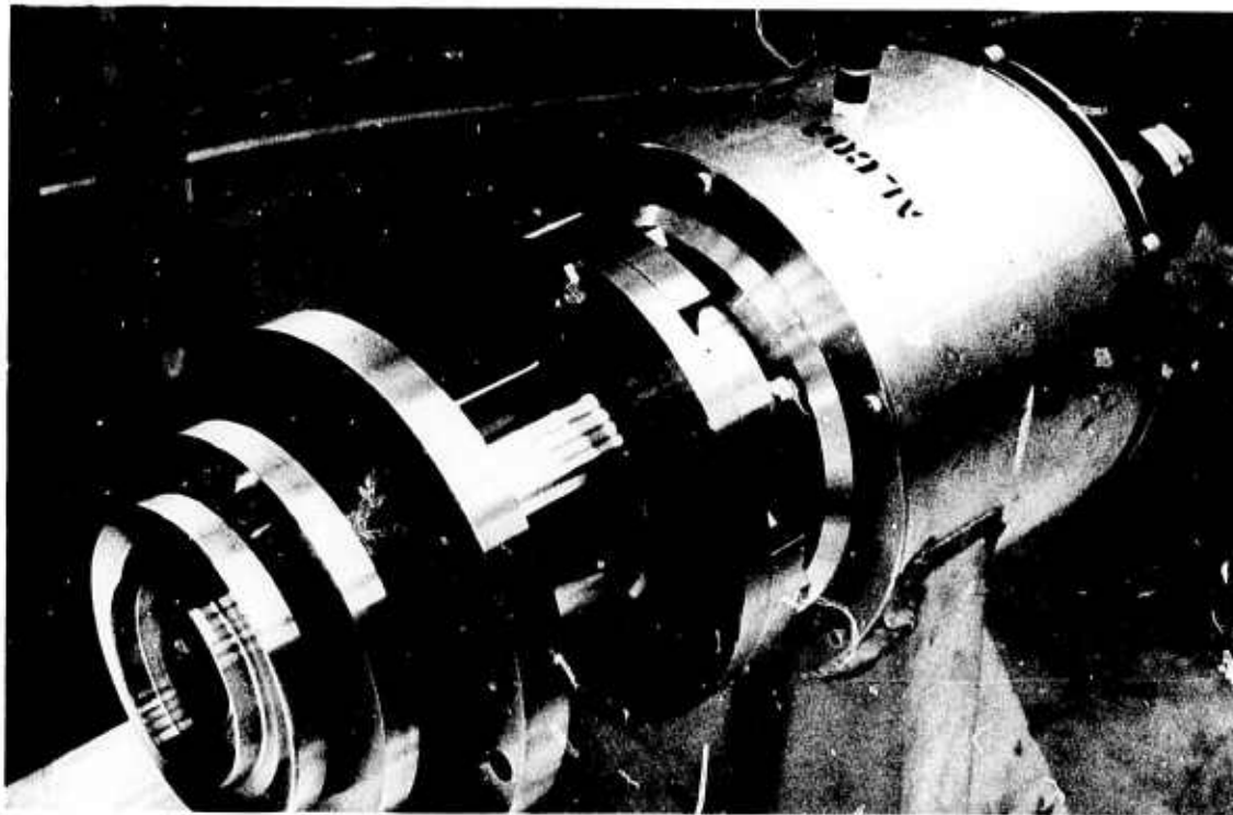
Figure 40. Rotor Assembly
