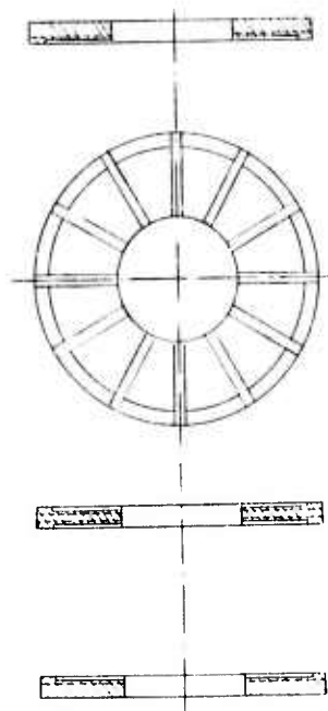
Figure 7. Textolite Disks for Coil Alignment and Cooling
