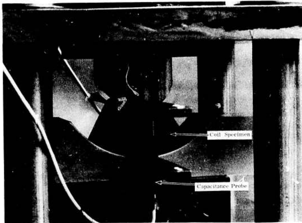
Figure 27. Coil Composite Specimen Setup for Radial Compression Tests
