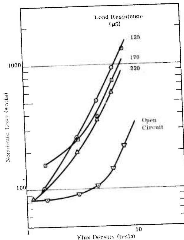
Figure 47. Collector Loss (Speed = 1000 Rpm)
