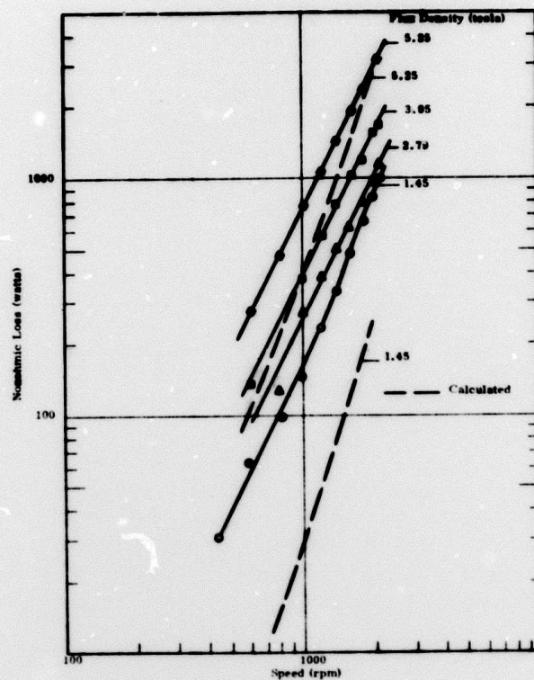
Figure 49. Collector Loss ( R_{Load} = 170 \mu\Omega )
