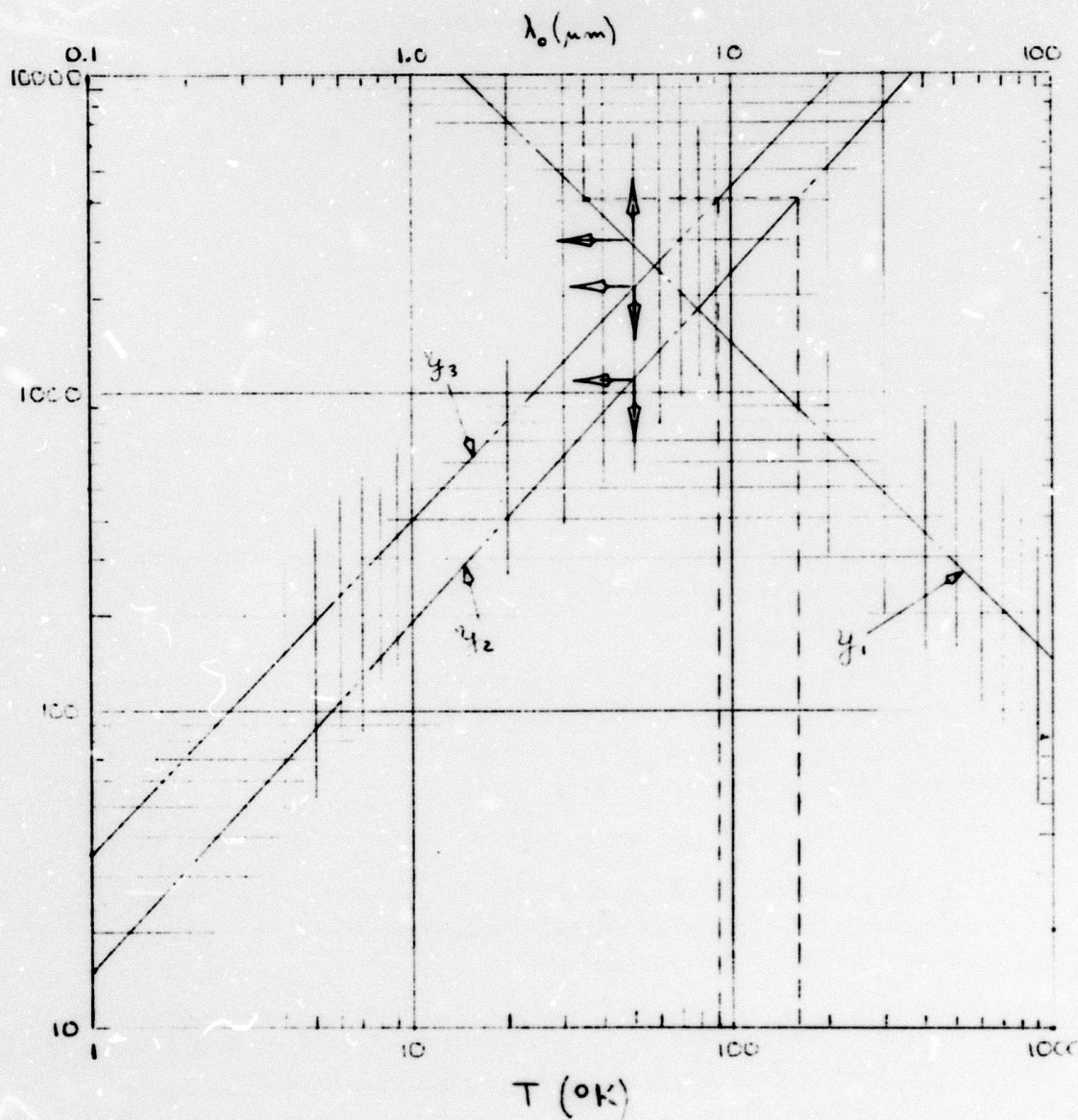
FIGURE 2 NOMOGRAM FOR DETERMINING T_{MAX} FOR A GIVEN \lambda_0
