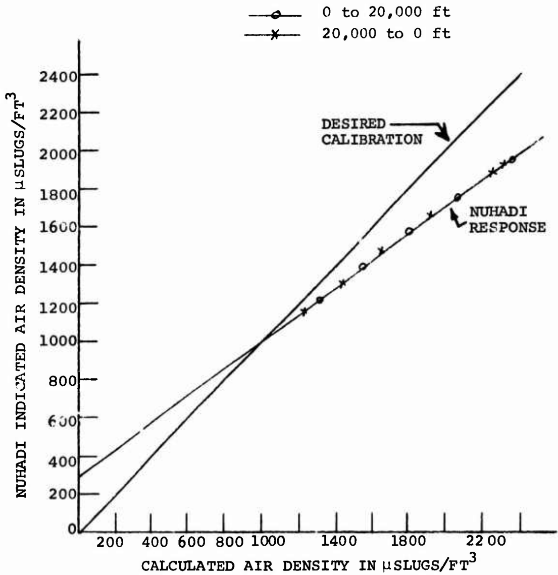
Figure 14. NUHADI Readout Versus Chamber Air Density.
