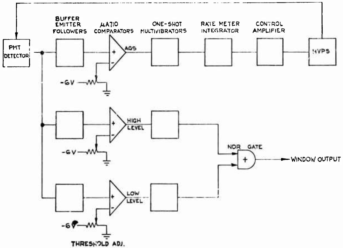
Figure 8. Detector Electronics.
