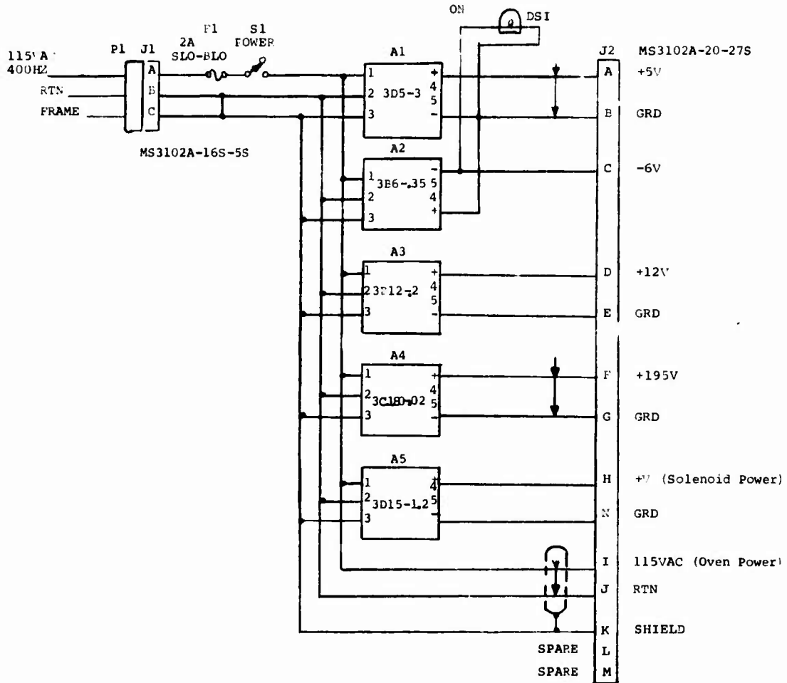
Figure 12. NUHADI Power Supply.
