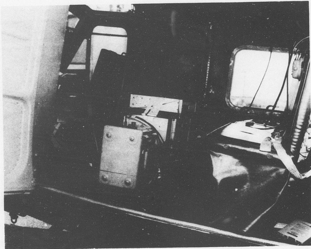
Figure 18. NUHADI Flight Test Installation of Electronics/Display Unit.
