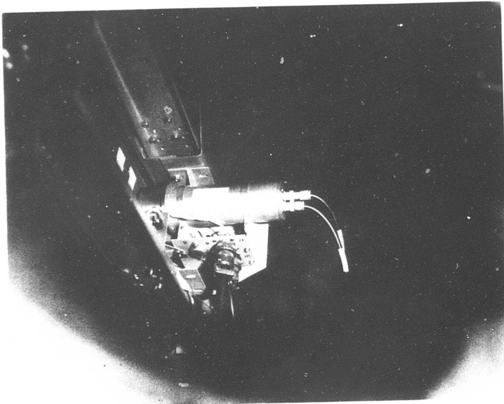
Figure 16. NUHADI Sensor Mounting - Interior View Looking Forward.
