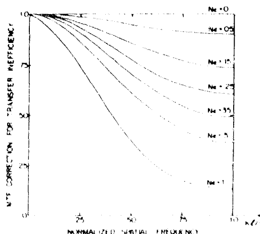
Fig. 4 MTF Correction for Transfer Inefficiency For a Single-Field Readout
