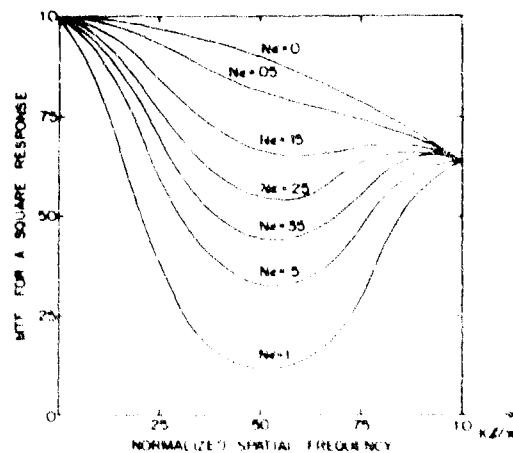
Fig. 6 MTF vs. Spatial Frequency for a Two-Field Readout
