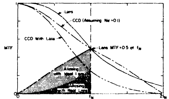
Fig. 7 Effect of Lens MTF on Aliasing
