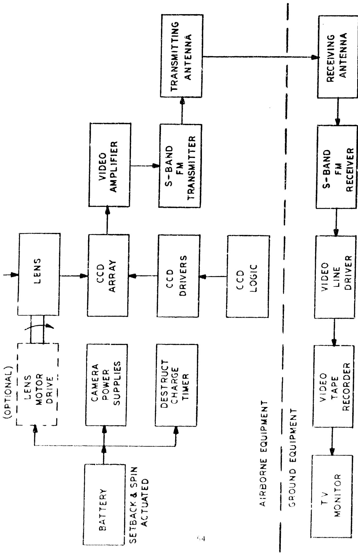
FIGURE 13. CCD TV RECONNAISSANCE SYSTEM BLOCK DIAGRAM
