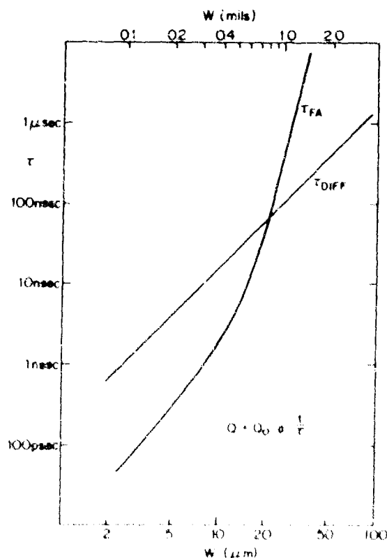
Fig. 16. Field-Aided and Diffusion Time Constants as a Function of Cell Spacing
