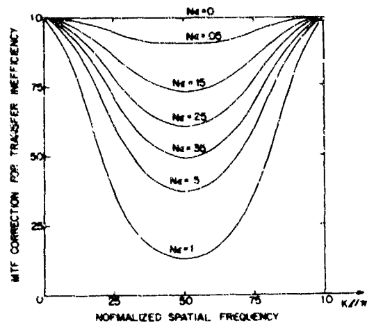
Fig. 5 MTF Correction for Transfer Inefficiency for a Two-Field Readout
