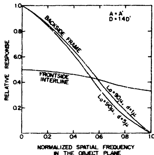
Fig. 3 Relative Response vs. Spatial Frequency for Frame and Interline Transfer From Barbe & White, CCD Applications Conference Proceedings
