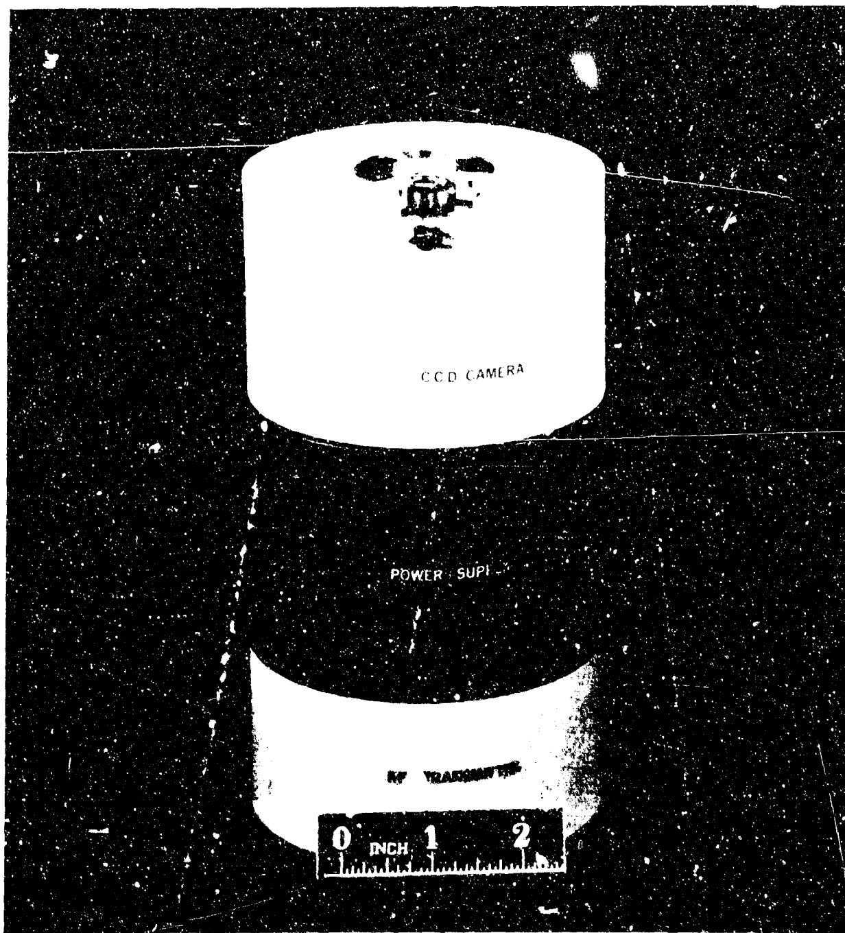
FIGURE 3. CUTAWAY MOCK-UP OF THE CCD CAMERA SYSTEM TO FIT INTO AN M-485-E2 ILLUMINATING ROUND
