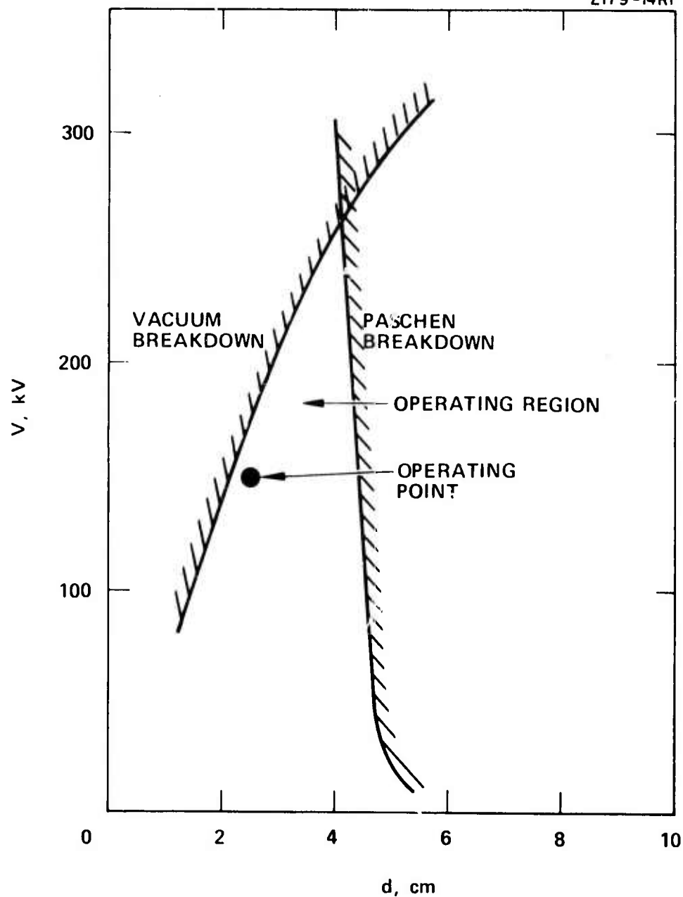
Fig. 2. Low pressure breakdown voltage in the plasma cathode accelerating region as a function of the gap width, d . The Paschen curve is for a pressure of 50 mTorr.
