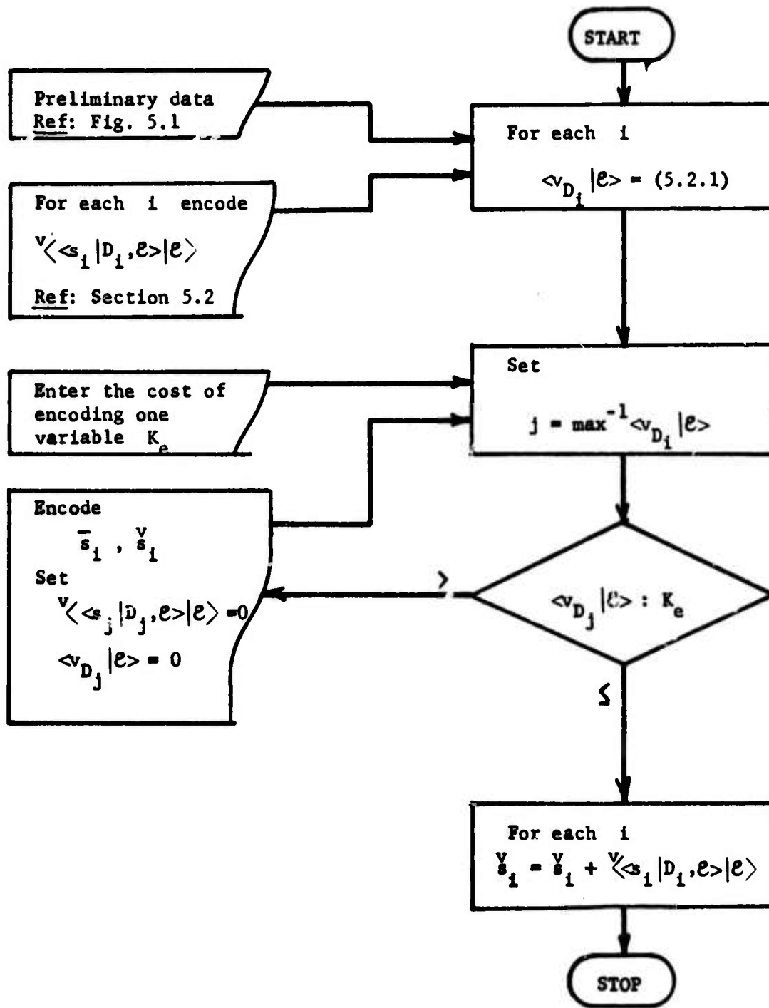
Figure 5.3 Iterative encoding of state variables
