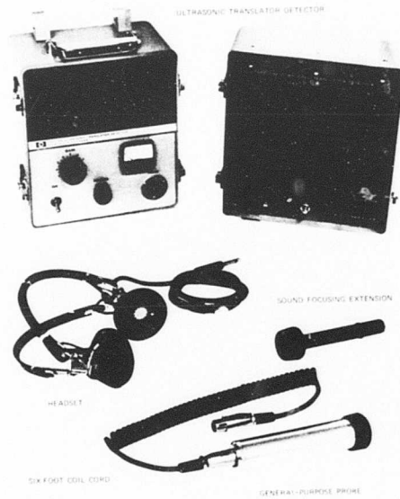
Figure 32. Ultrasonic Translator Detector.
