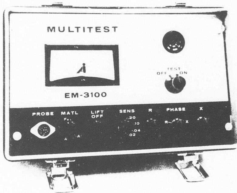
Figure 15. Multitest EM-3100 Eddy Current Instrument.
