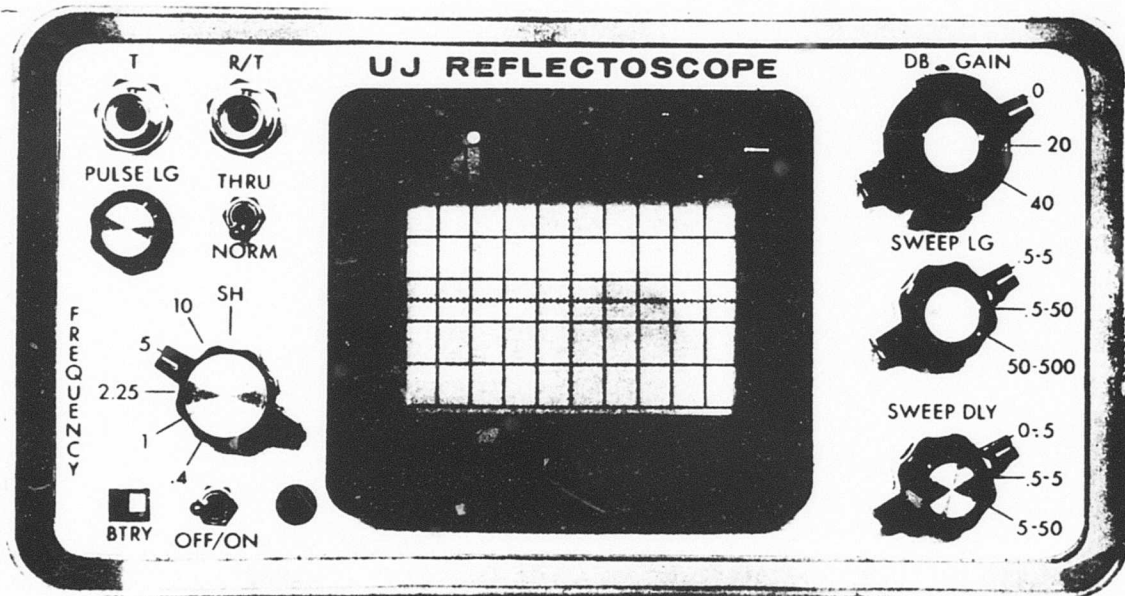
Figure 21. Ultrasonic Reflectoscope.
