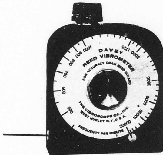
Figure 37. Reed Vibrometer.
