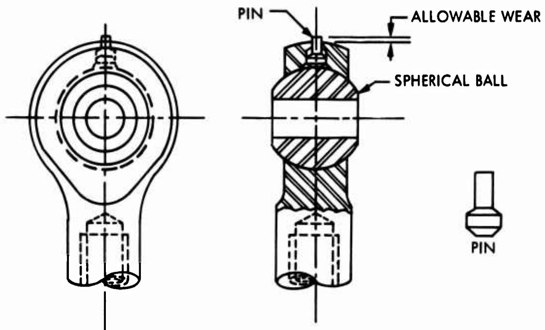
Figure 28. Rod End Bearing Wear Pin Installation.
