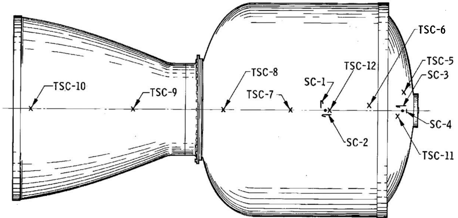
Fig. 7 Motor Case Thermocouple and Strain-Gage Locations
