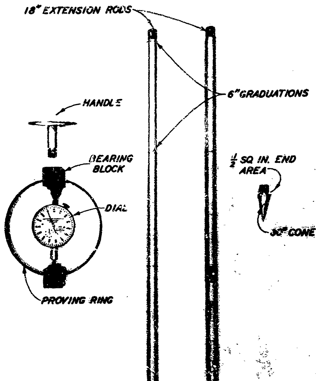
Fig. 9-1: Cone Penetrometer Disassembled.
