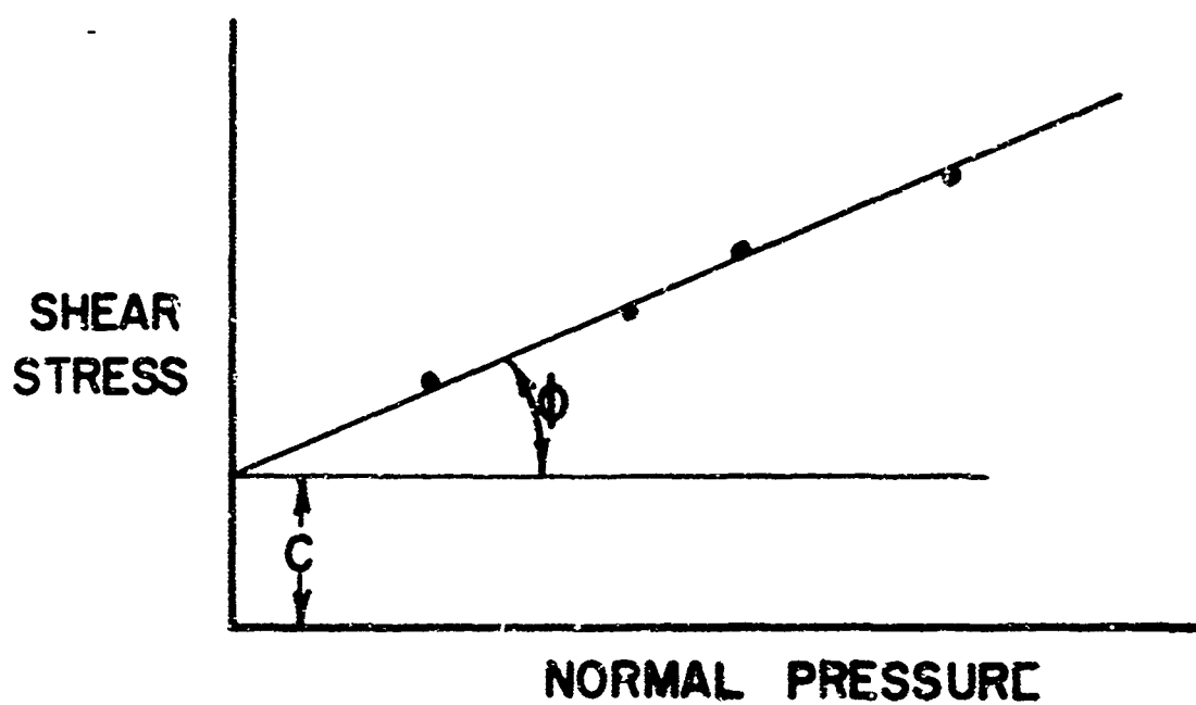
FIG. 8-6. DETERMINATION OF C AND \phi
