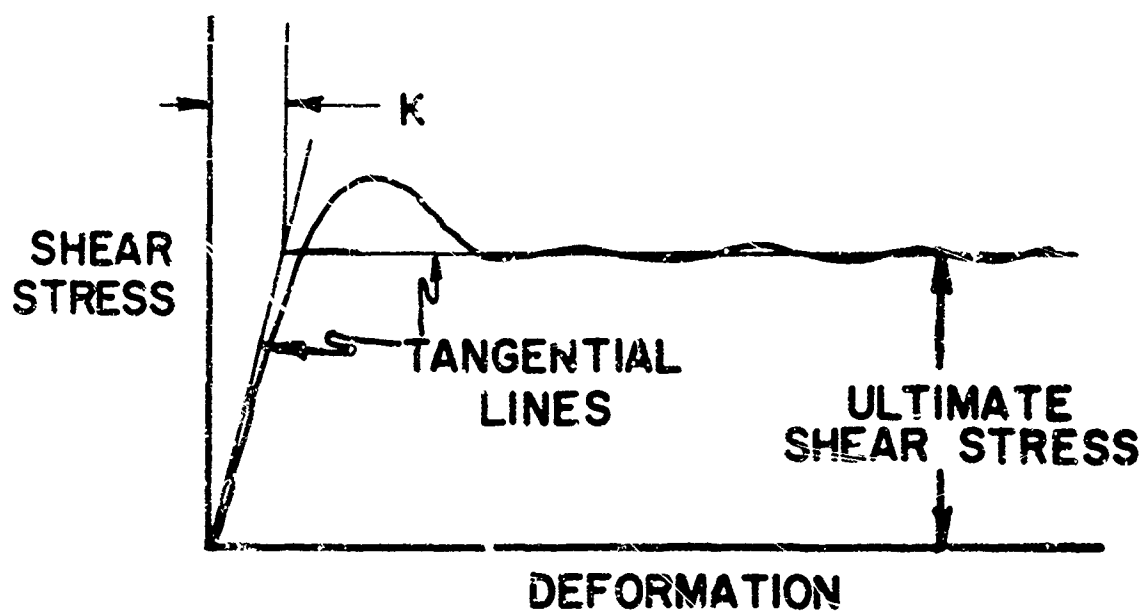
FIG. 8-5. ULTIMATE SHEAR STRESS AND K
