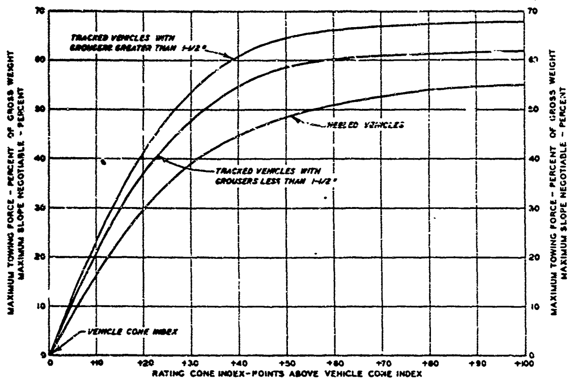
Fig. 9-6. Maximum continuous tractive effort on level ground; maximum slope and maximum towing force versus rating cone index expressed as points above vehicle cone index
