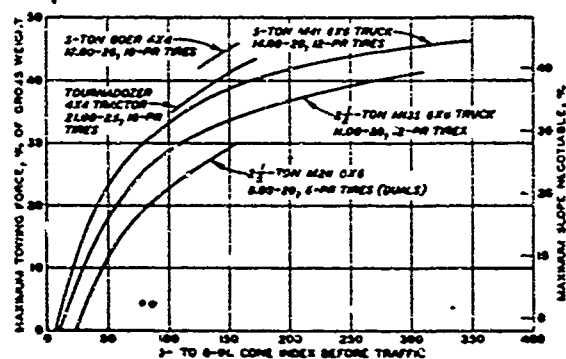
Fig. 9-10. Effect of tire size on vehicle performance on dry-to-moist sand. Vehicles operated at 10-psi tire pressure
