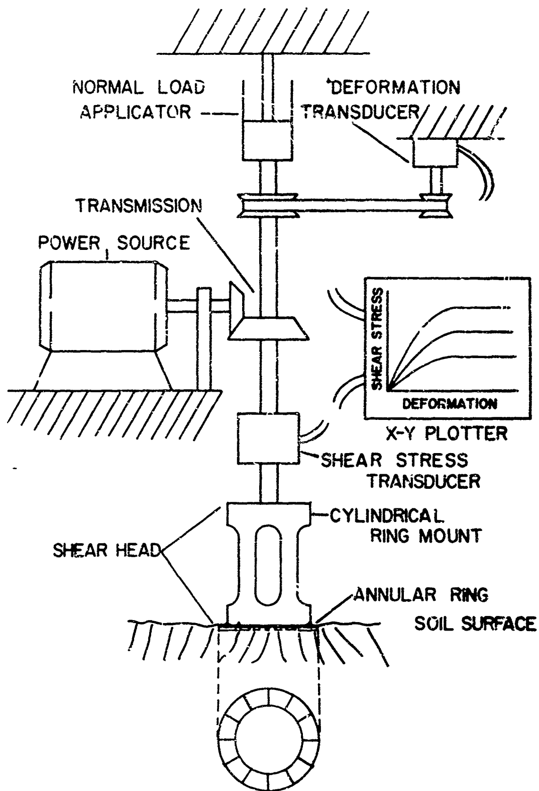
FIG. 8-3. SCHEMATIC OF A SHEAR TEST DEVICE
