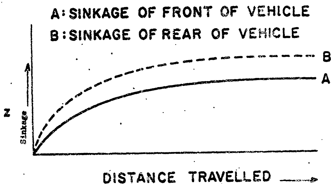
Fig. 4-3. Examples of Continuous Traces of Sinkage Measurements
