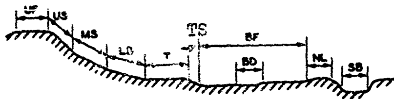
Fig. 9-11. Topographic classification
