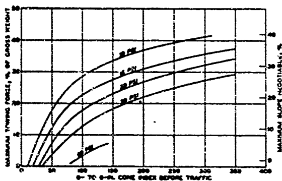
Fig. 9-9. Effect of tire pressure on vehicle performance on dry-to-moist sand. M34 and M135, 2-1/2-ton, 6x6 trucks; 11.00-20, 12-FR, NDCC tires
