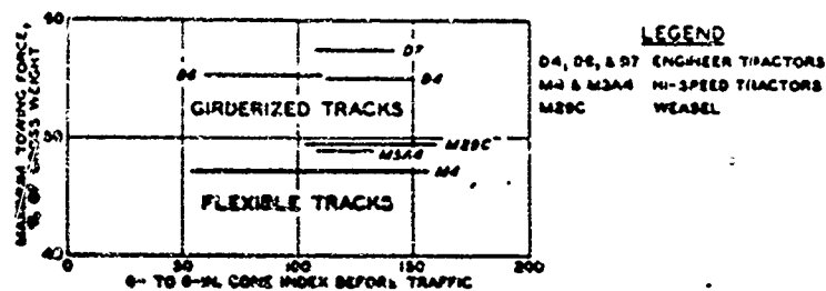
Fig. 9-8. Performance of tracked vehicles in dry-to-moist sand
