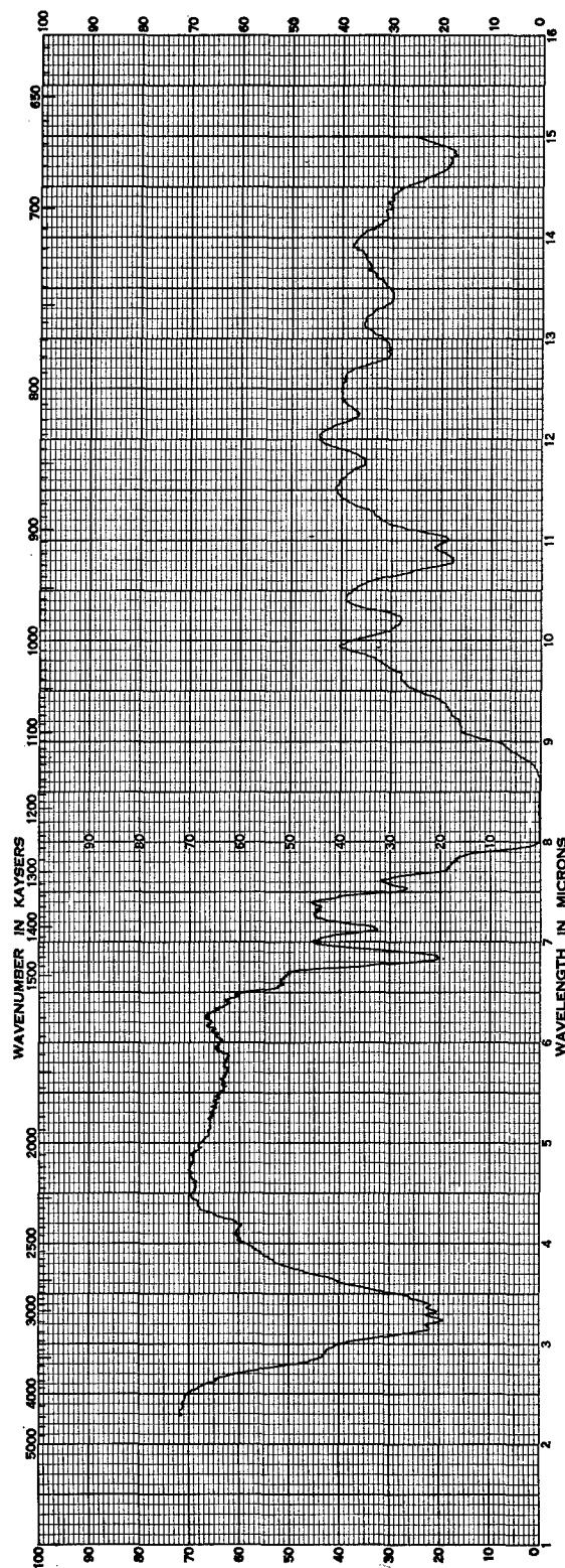
Fig. 5 Poly(perfluorooctene 1, 2, 4-triazole)
