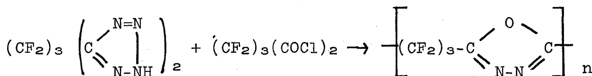
Eq. 5
