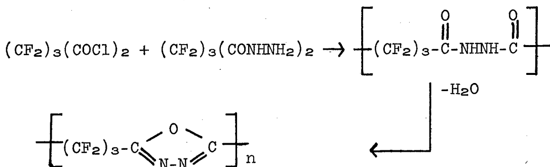
Eq. 7
