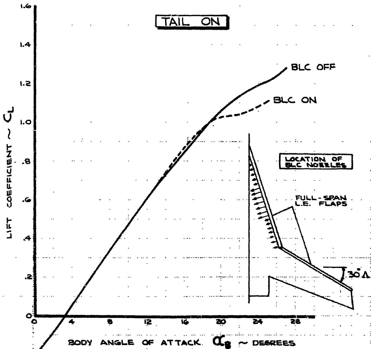
Figure 86. Effect Of Blowing BLC At Strake Leading-Edge On Lift
