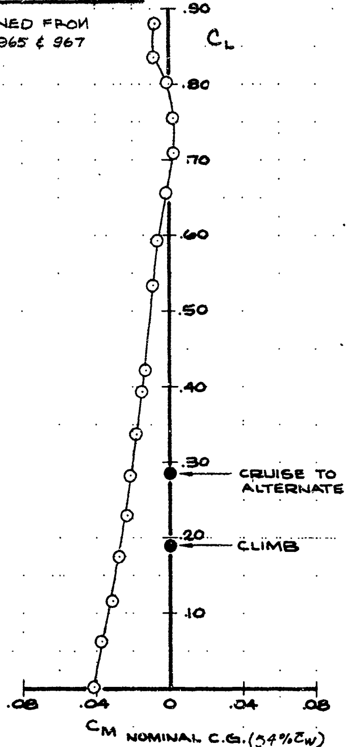
Figure 14. Transonic Longitudinal Stability Characteristics, \Lambda_{LE} = 42
