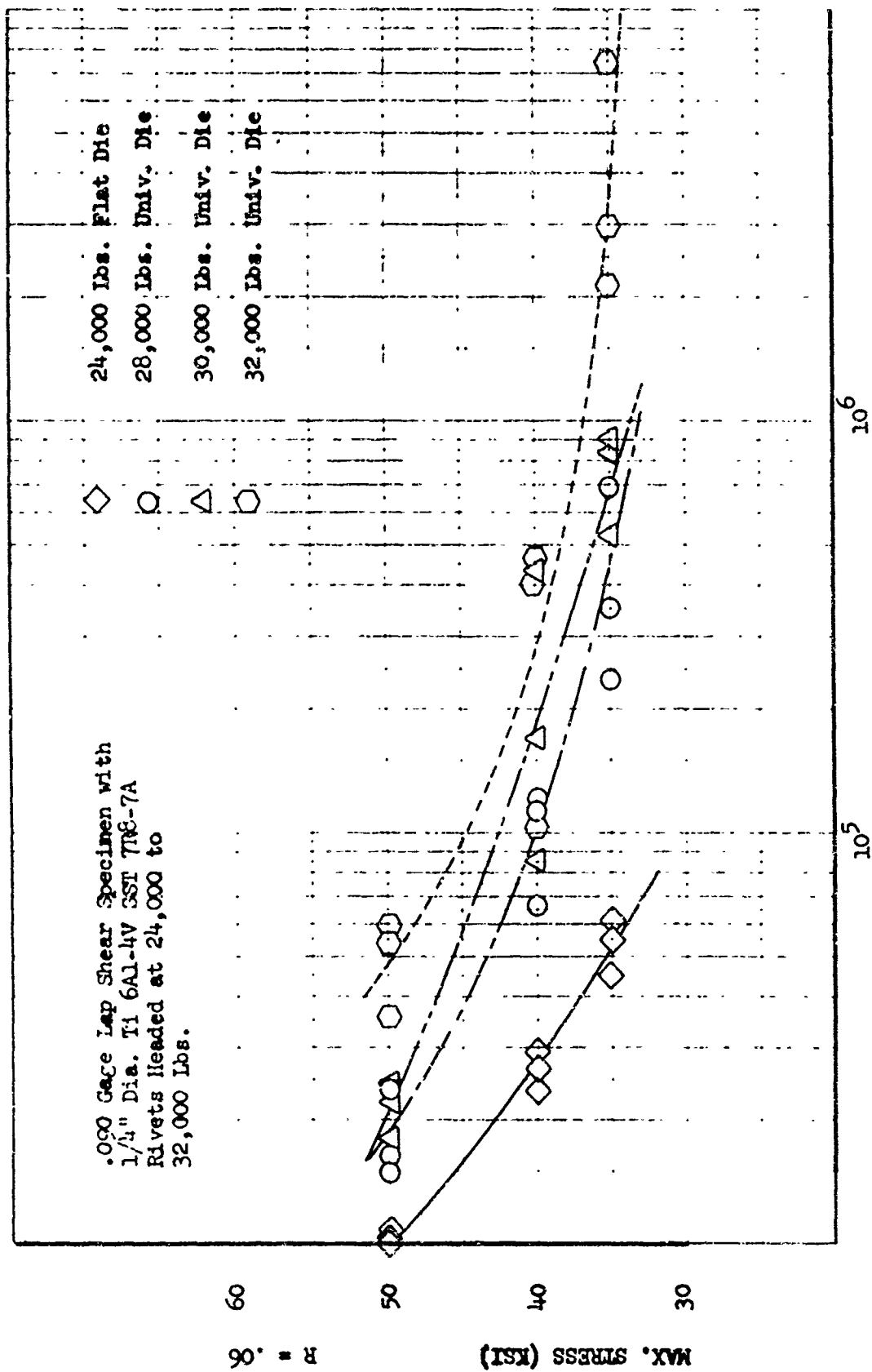
Figure 29. Heading Force Study for Ti 6Al-4V Rivets
