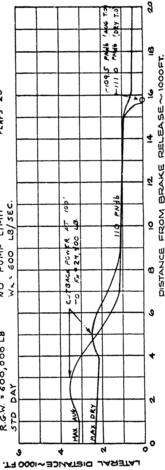
Figure 9. Takeoff Noise Contours - Power Cut-Back
