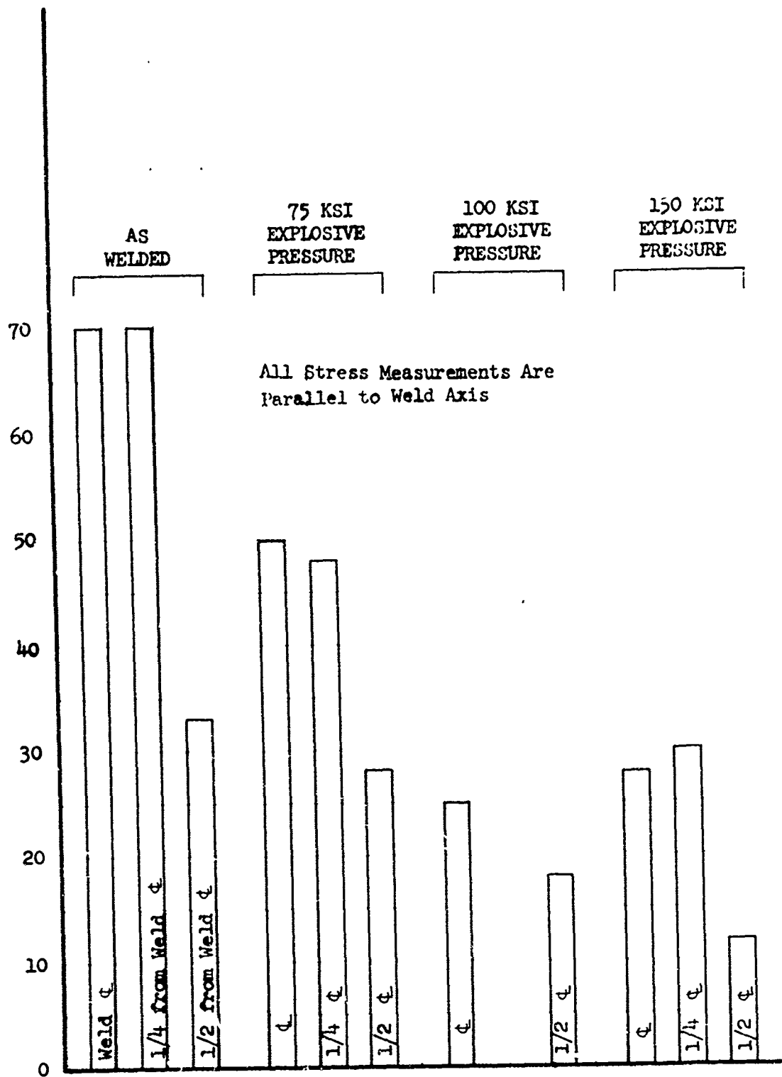
Figure 27. Effect of Explosive Stress Relief on Residual Stress in Welded Ti 6Al-4V
