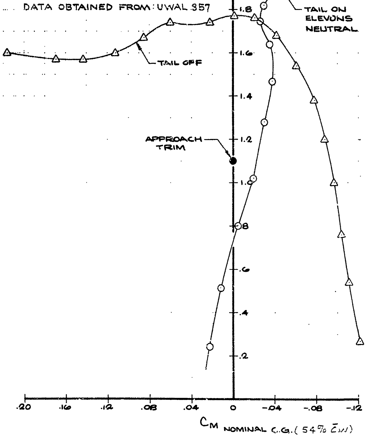
Figure 12. Longitudinal Stability, Landing Configuration
