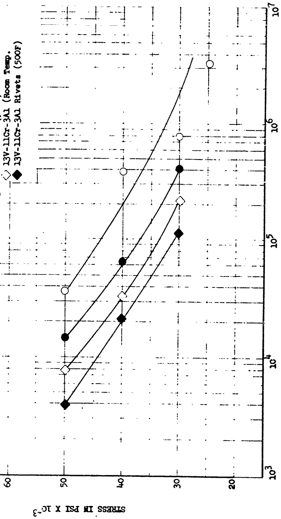
Figure 33. Effect of Temperature on Joining Fatigue Life
