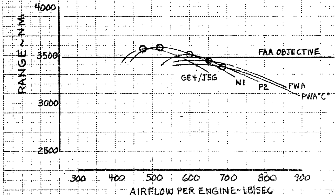
Figure 5. B-2707 Engine Sizing Range
