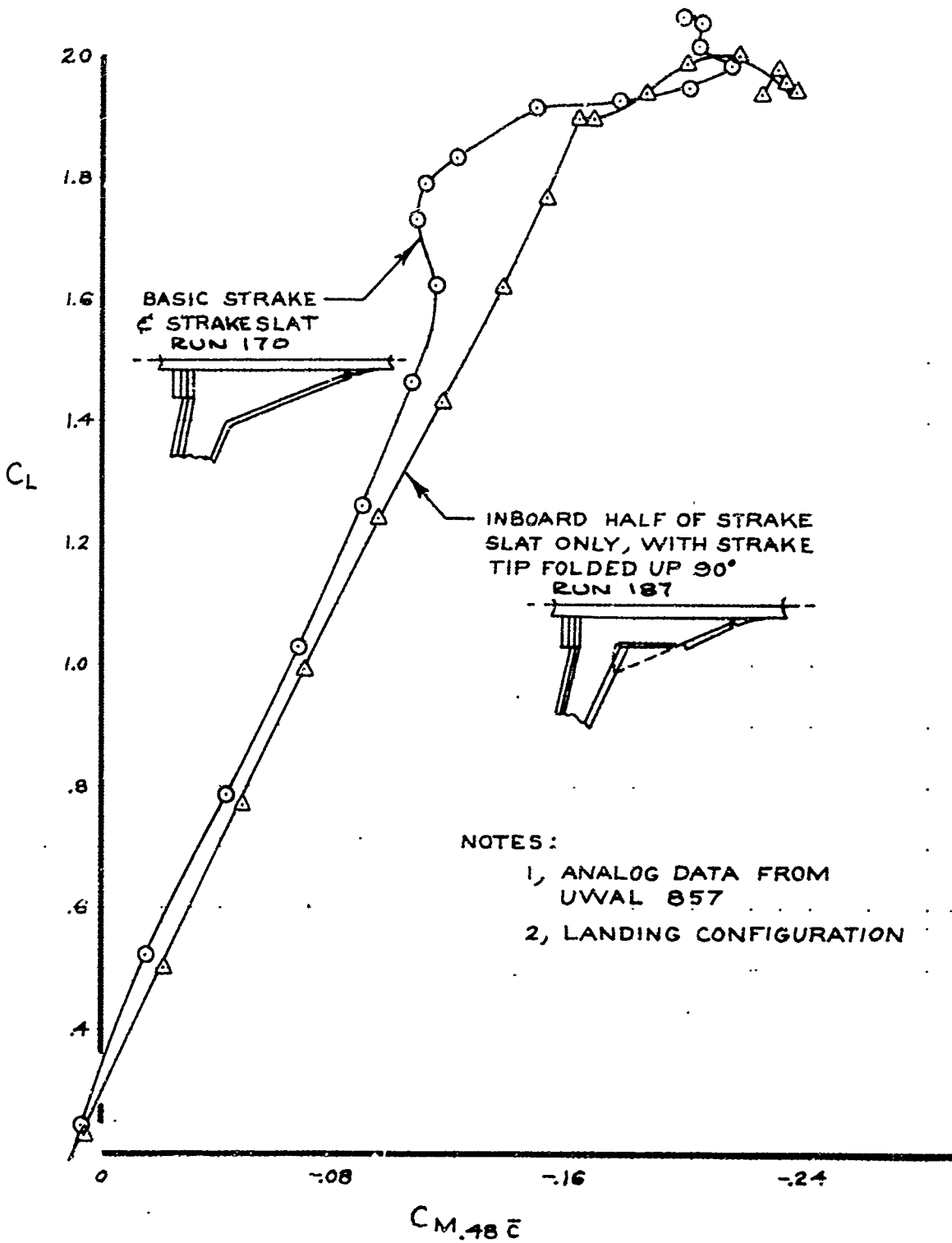
Figure 13. Strake Modification to Improve Flaps-Down Stability
