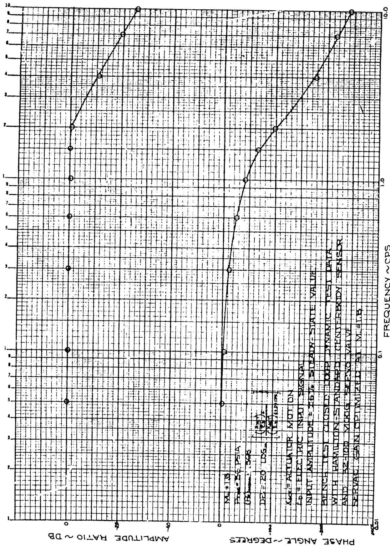
Figure 70. Centerbody Loop Test with Hamilton Standard Sensor, M L = 1.8
