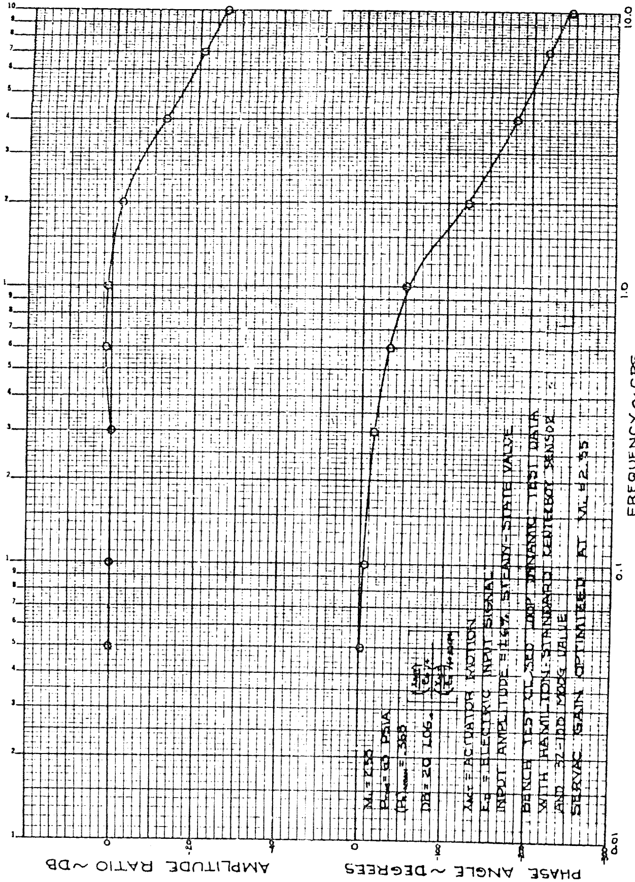
Figure 72. Centerbody Loop Test with Hamilton Standard Sensor, M_L = 2.55 , Optimized
