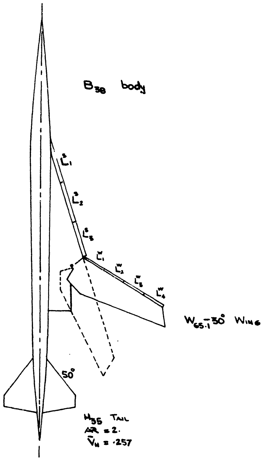
Figure 84. Wind Tunnel Model Platform
