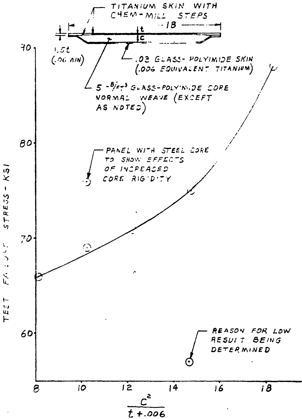
Figure 38. Honeycomb Panel Test Allowables
