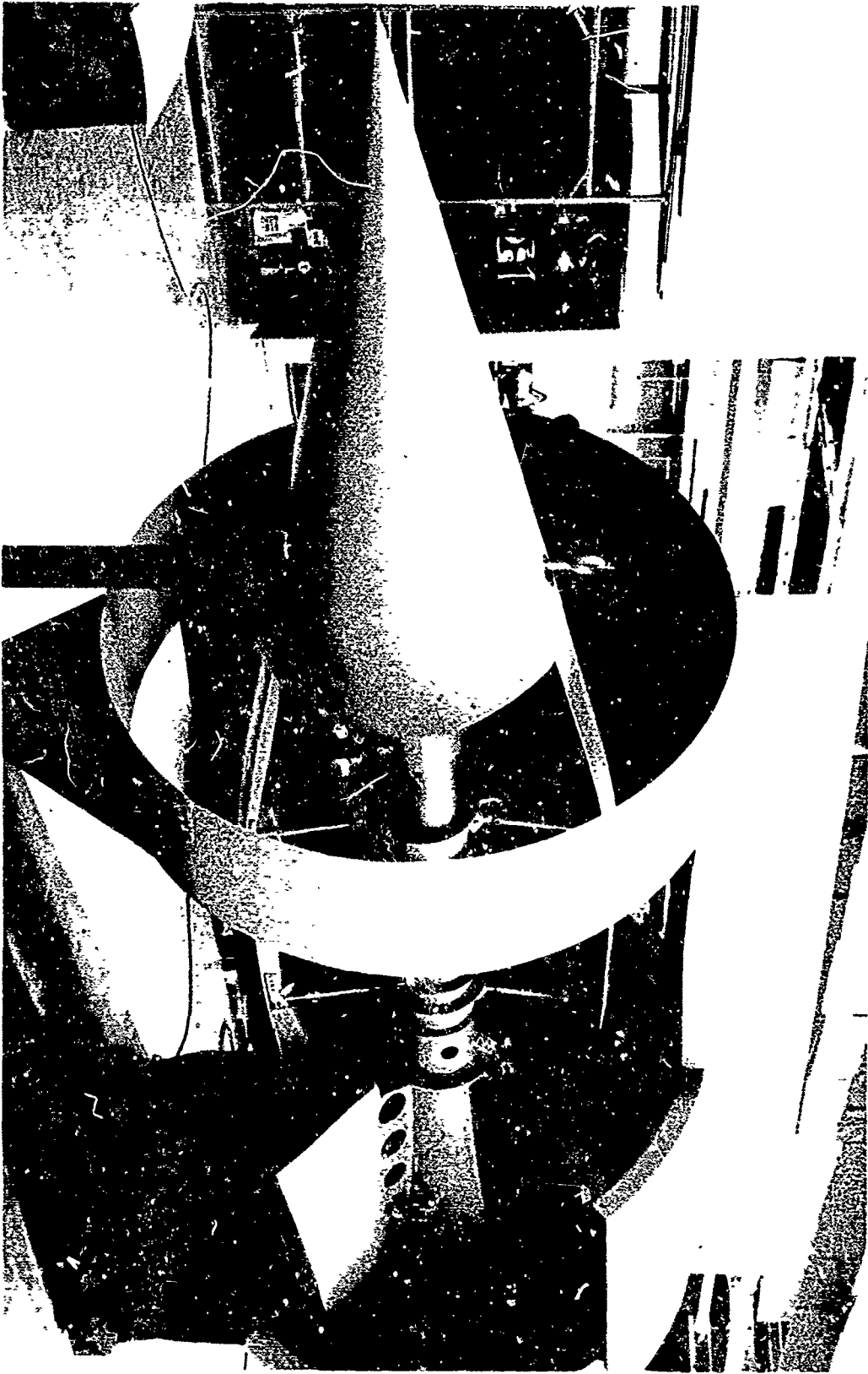
Figure 66. Full-Scale inlet Mockup
