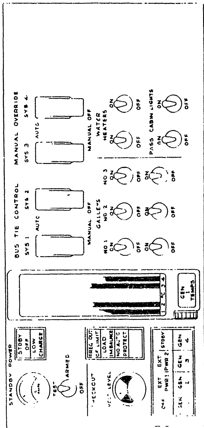
Figure 56. Electrical Panel Diagram
