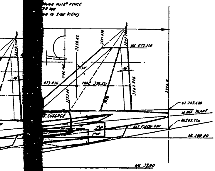
Figure 1. General Arrangement, Model B-2707 (GE)
