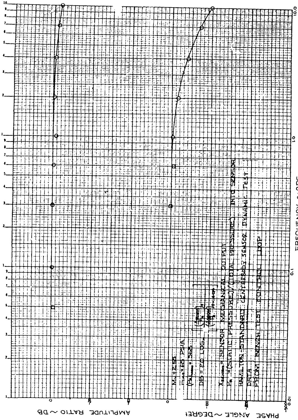
Figure 74. Hamilton Standard Centerbody Sensor Response Characteristics
