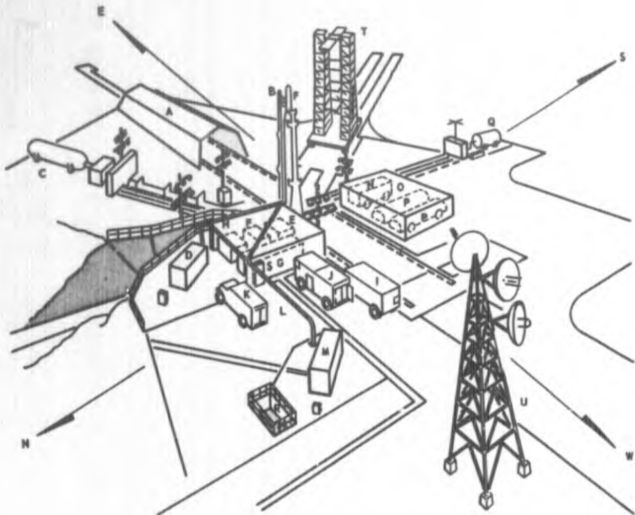
LAUNCH PAD I OF COMPLEX 75-1 VAFB GENERAL ARRANGEMENT
