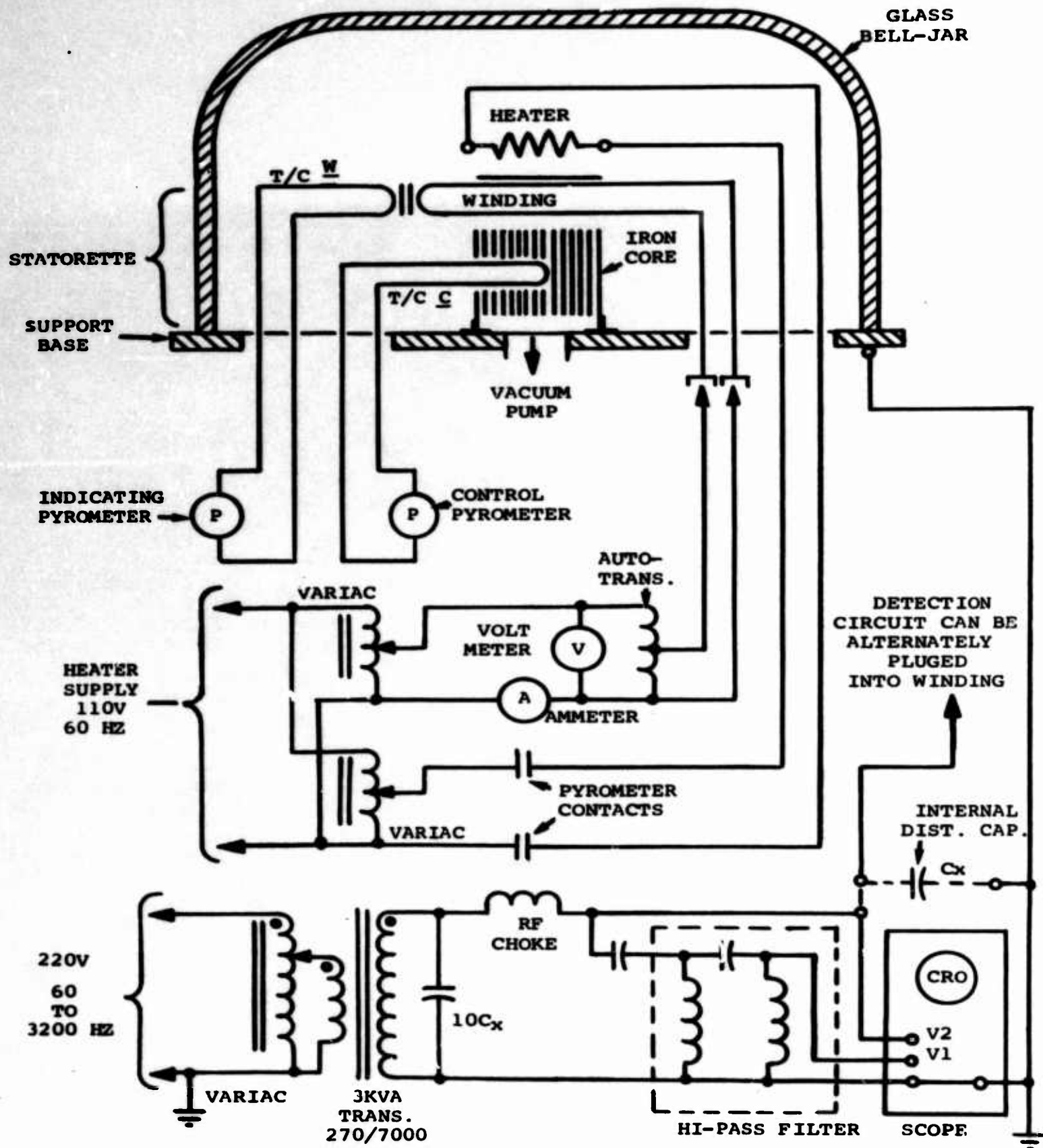
Figure 11. Schematic of Corona Statorettette Test
