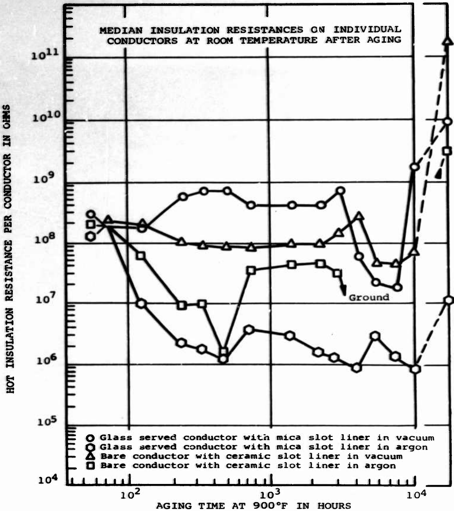
Figure 8. Effect of Time at Temperature on Stator Insulation Electrical Resistance in Vacuum and Argon
