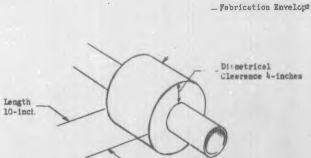
Figure 4. Envelope Requirements Thick Wall Tubing 1-inch Through 16-inch Diameters
