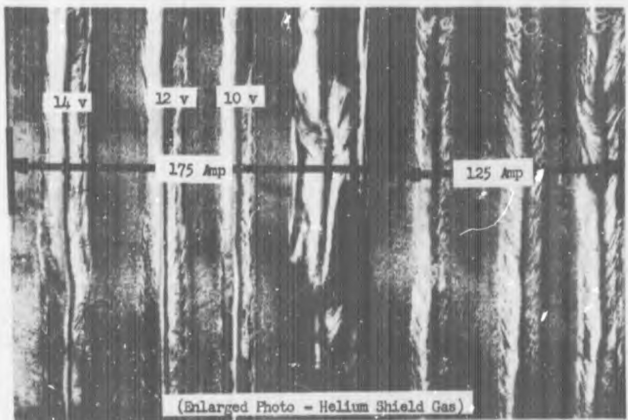
Figure 24 Effect of Shield Gas and Position on Weld Bead Control,(cont.)
