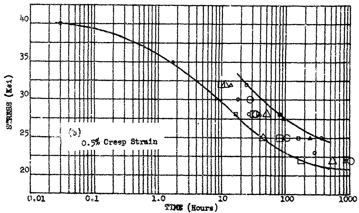
Figure 47 Creep Strain and Creep Rupture Properties of 2618-T61 Aluminum Forgings at 400 F
