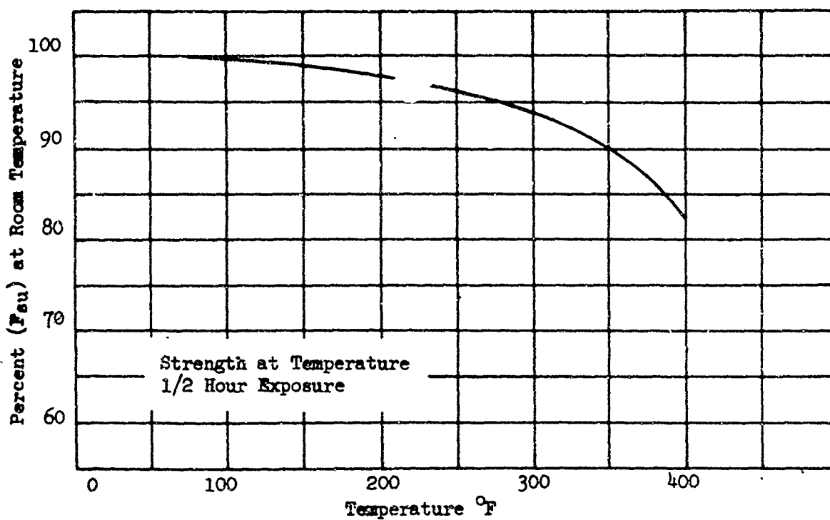
Effect of Temperature on the Ultimate Shear Strength (F su ) of 2618-T61 Aluminum Forgings
