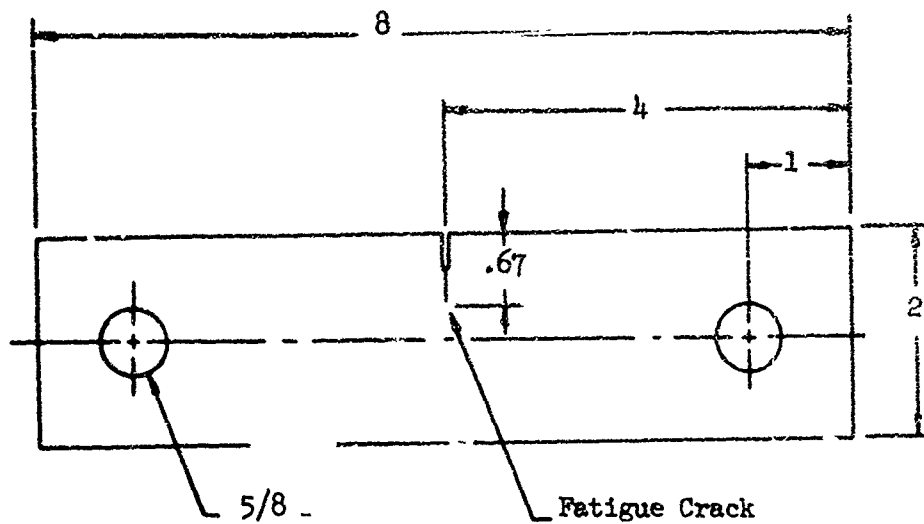
Figure 15 Single-Edge-Notch Fracture Toughness Test Specimen (All dimensions are inches)
