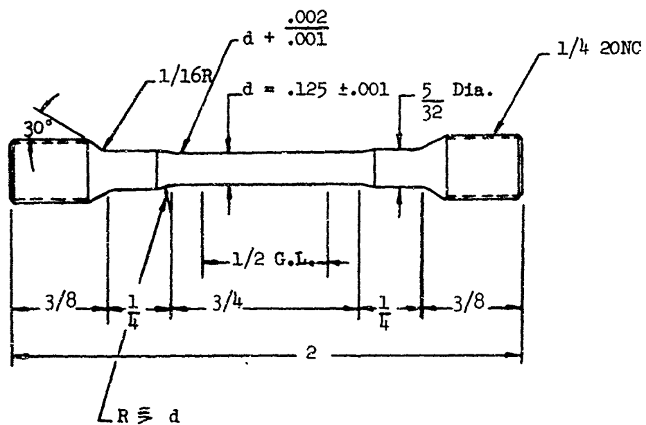
Figure 16 Axial Stress Corrosion Specimen (All dimensions are inches)
