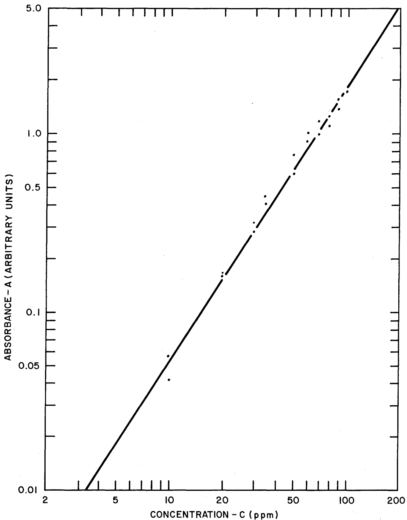
Figure 2 - Calibration Curve for AMOX
