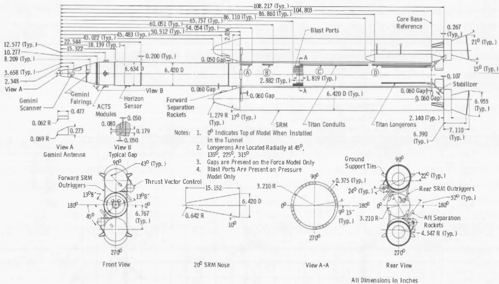
Fig. 5 Titan III/MOL Geometry
