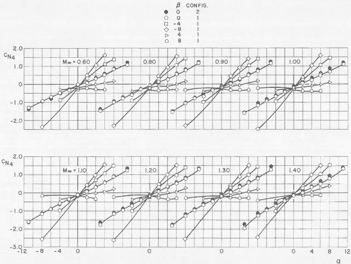
Fig. 39 Variation of SRM Normal-Force Coefficient with Angle of Attack for Configurations 1 and 2
