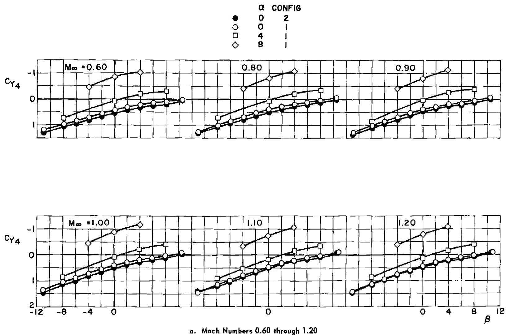
Fig. 41 Variation of SRM Side-Force Coefficient with Sideslip Angle for Configurations 1 and 2
