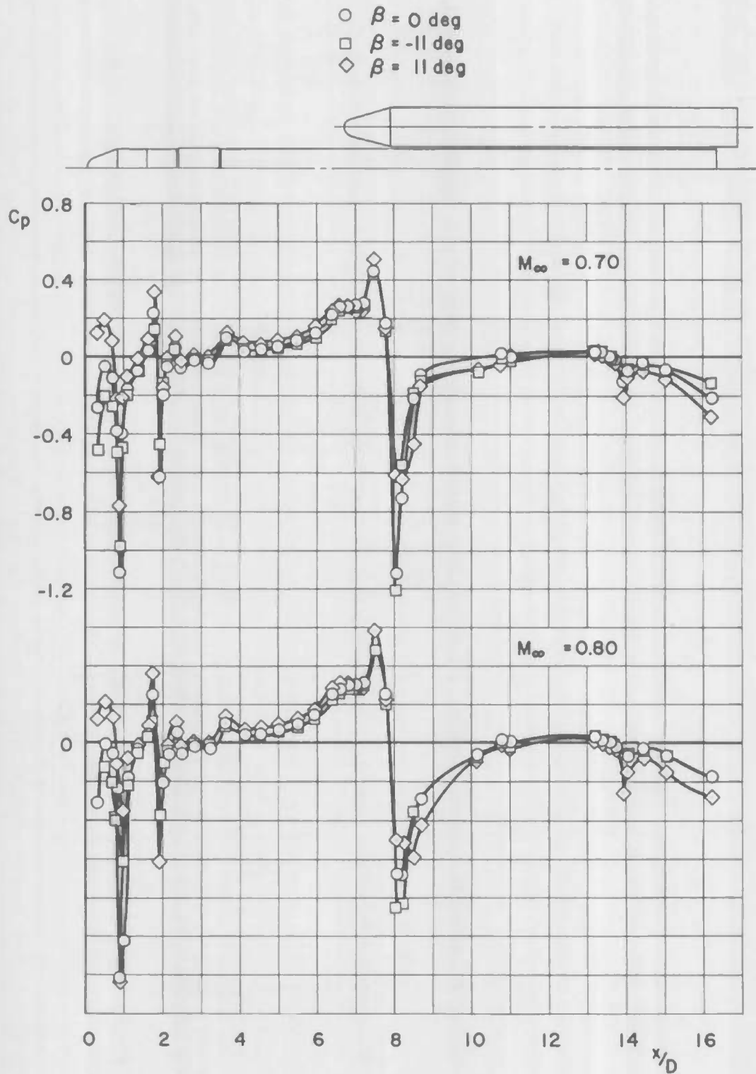
Fig. 51 Variation of Surface Pressure Coefficient with Model Station for Orifices Oriented at 90^\circ for Configuration 3, \alpha = 0
