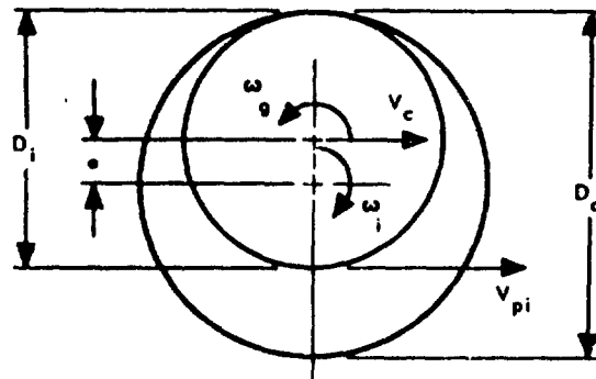
Figure 30. Diagram — Determination of \omega_g/\omega_1
