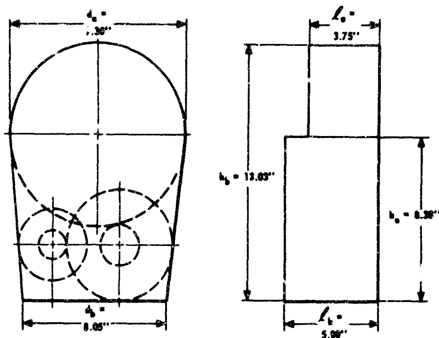
Figure 16. Configuration for Calculating Spur Gear Transmission Volume
