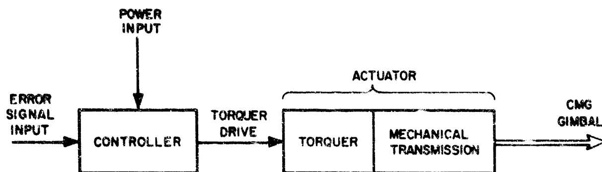
Figure 1. Basic Relationship Between Controller and Actuator
