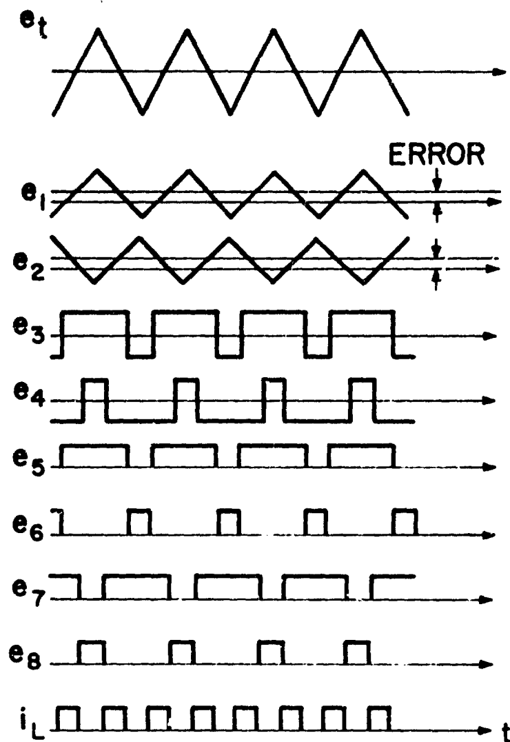
Figure 62. Positive Error Waveforms
