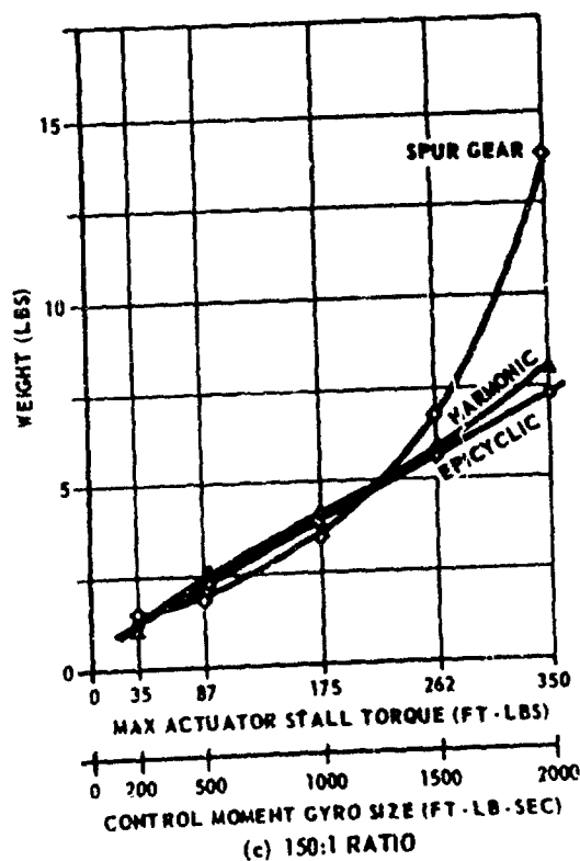
Figure 32. Transmission Weight Versus Stall Torque
