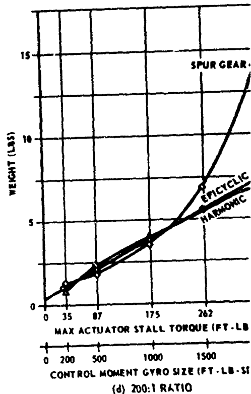
Figure 32. Transmission Weight Versus Stall Torque
