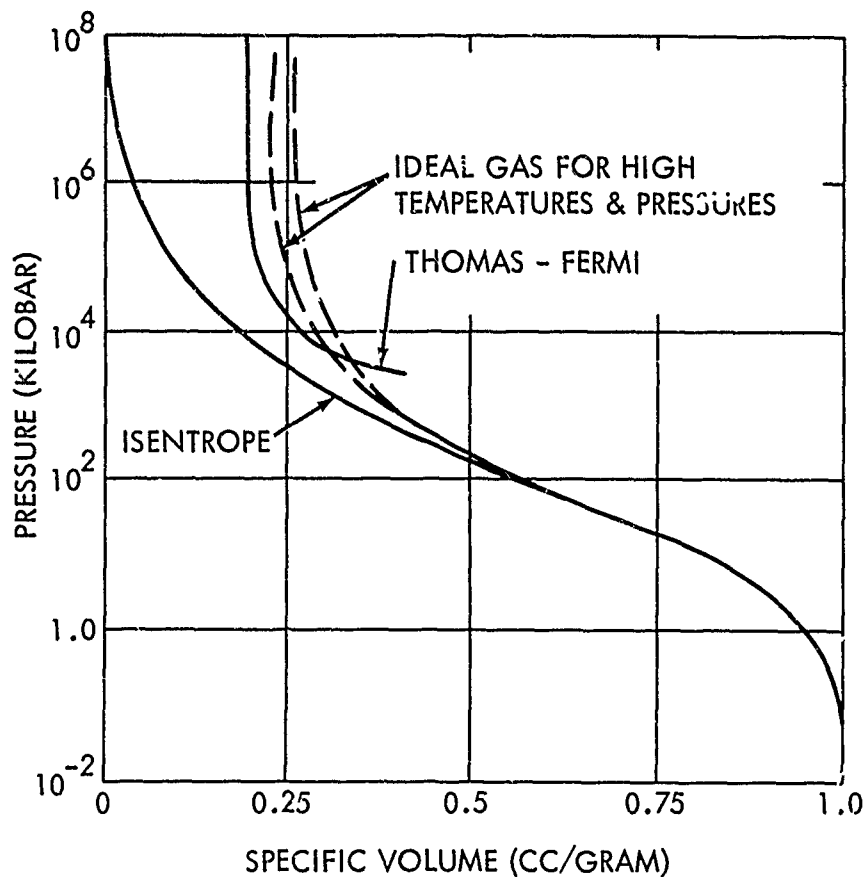
Figure 3.4 - Isentrope and Rankine-Hugoniot Adiat for Water (Schematic)
