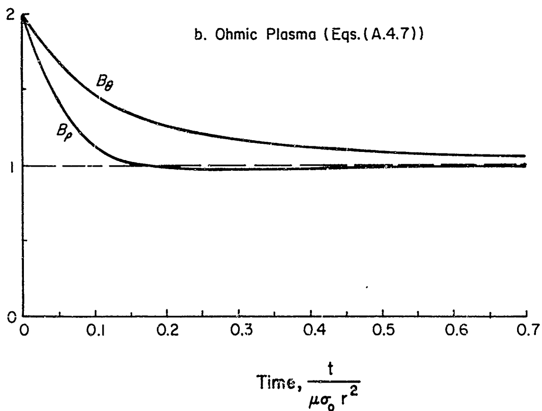
Fig. 2. 5 Magnetic Fields for a Horizontal Dipole in a Semi-infinite Plasma
