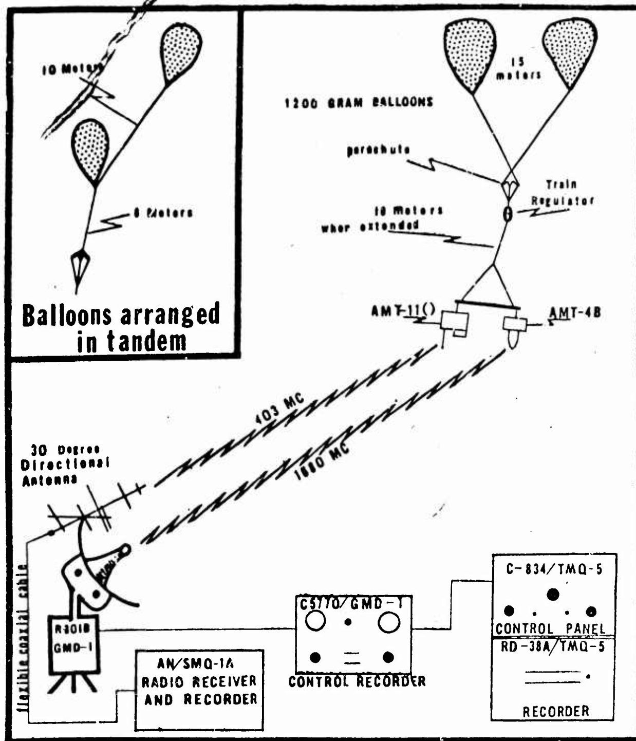
Figure 1. Ground and Flight Equipment Configuration. Inset shows tandem balloon arrangement used in flights seven, eight, and nine.
