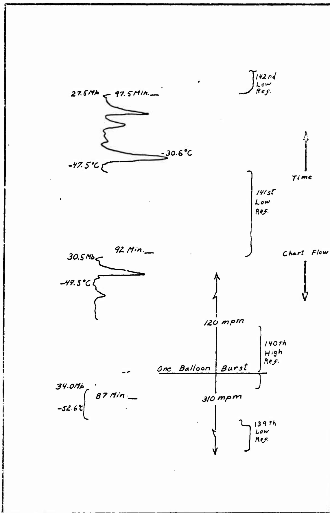
Figure 5. Heat Spikes Observed During Slow Ascent.
