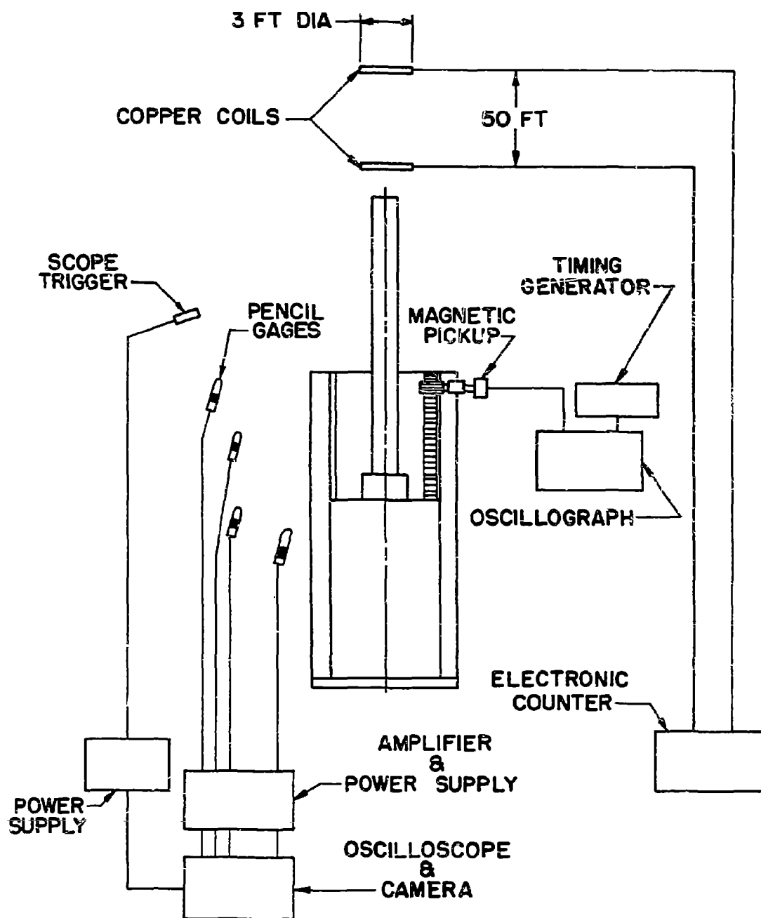
INSTRUMENTATION SCHEMATIC
