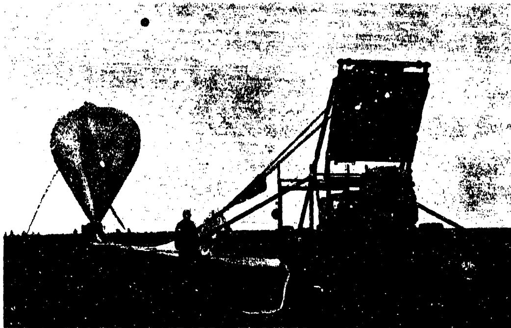
Balloon train layout with University of Chicago sphere on M-36 launch truck.
