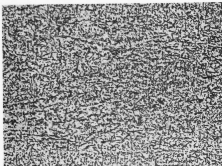
Figure 14. Micrograph of Ti-Zr-B (21-68-11) Alloy.
