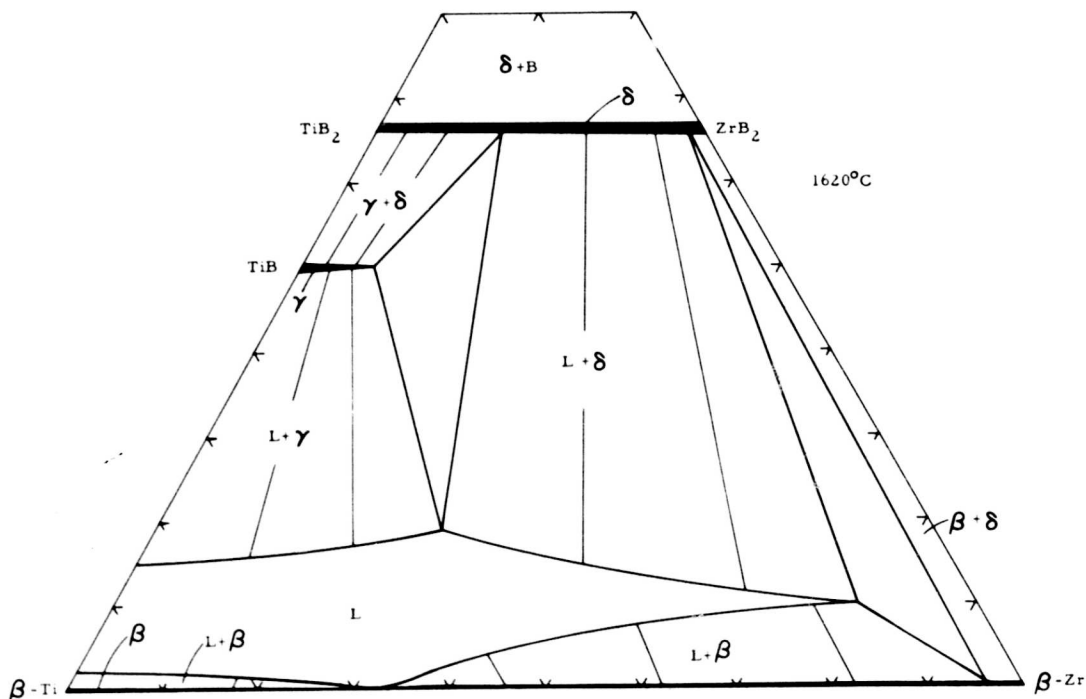
Figure 32. Isothermal Section at 1620°C.
