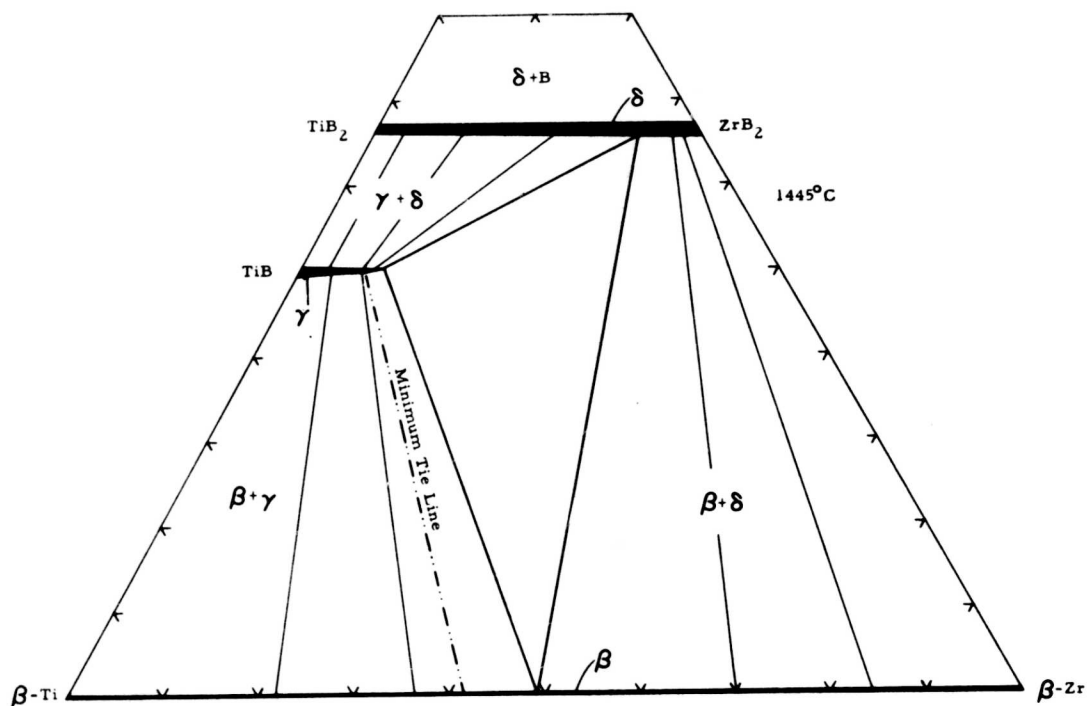
Figure 22. Isothermal Section at 1445°C.
