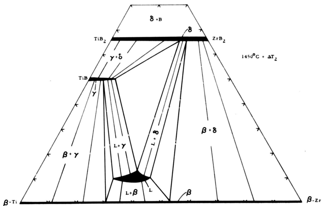
Figure 30. Isothermal Section at 1450°C + \Delta T_2 .
