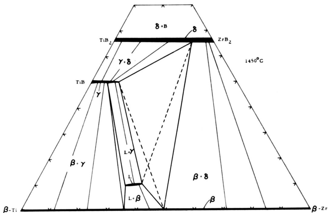
Figure 29. Isothermal Section at 1450°C.
