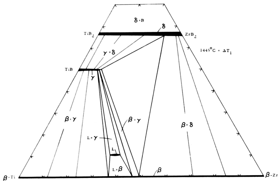
Figure 28. Isothermal Section at 1445°C + \Delta T_1 .
