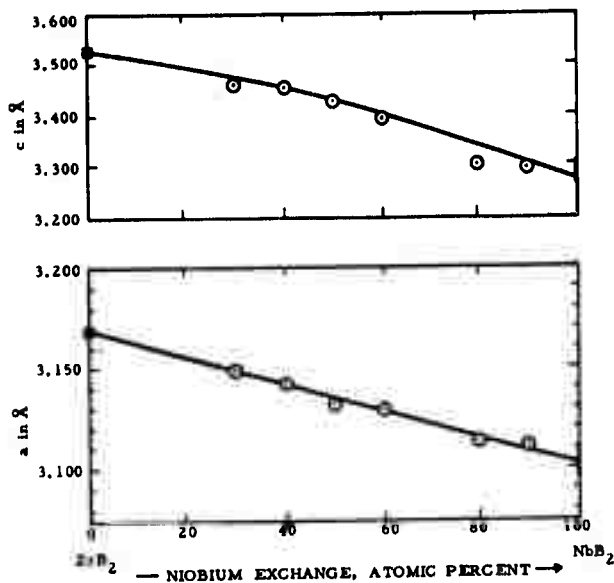
Figure 41. Lattice Parameters of Pseudo-Binary \text{ZrB}_2 - \text{NbB}_2 .
