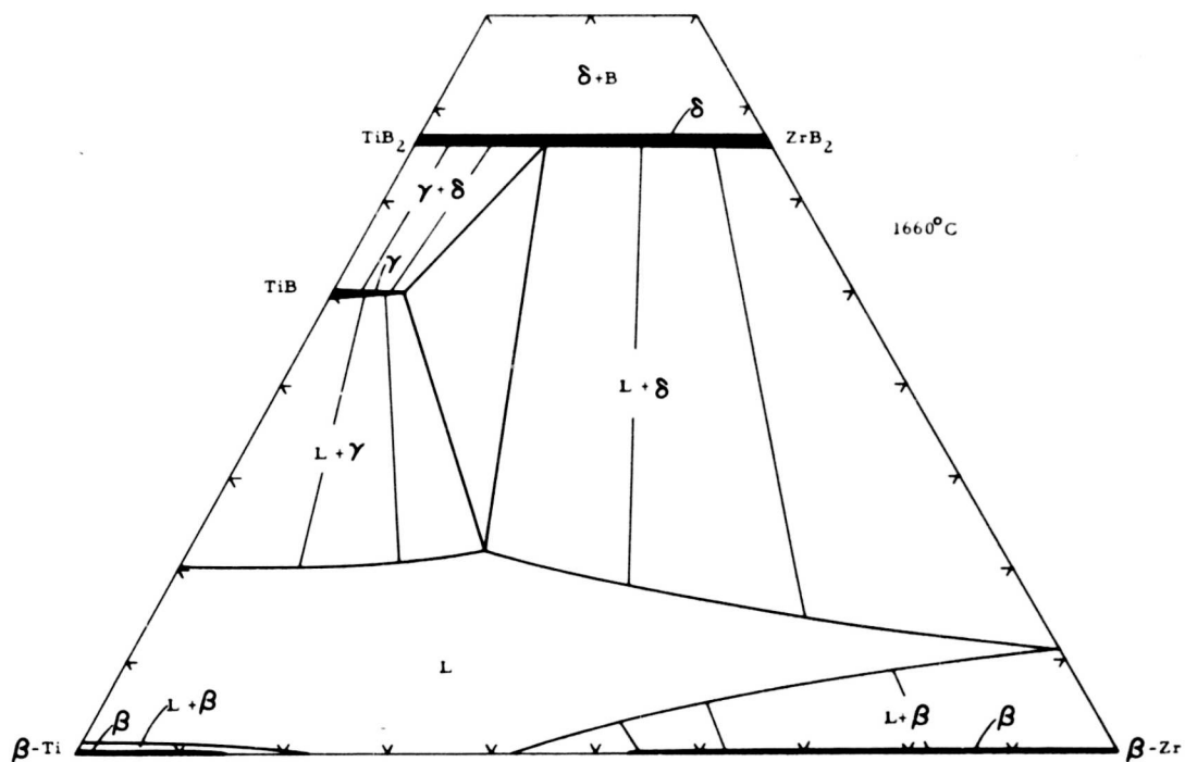
Figure 33. Isothermal Section at 1660°C.
