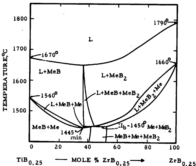
Figure 3. Ti-Zr-B: Isopleth Across 20 Atomic Percent Boron
