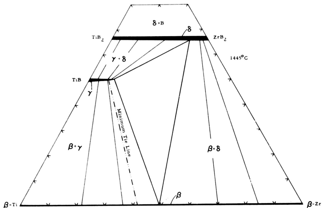
Figure 27. Isothermal Section at 1445°C.
