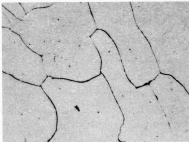
Figure 20. Micrograph of Ti-Zr-B (28-5-67) Alloy.
