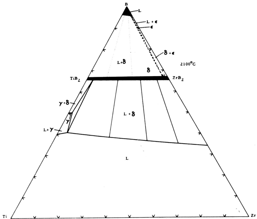
Figure 38. Isothermal Section at 2100°C.
