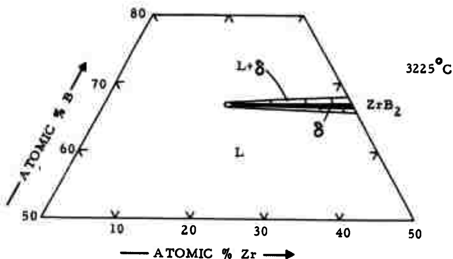
Figure 40. Isothermal Section at 3225°C.
