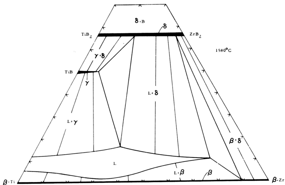
Figure 31. Isothermal Section at 1580°C.
