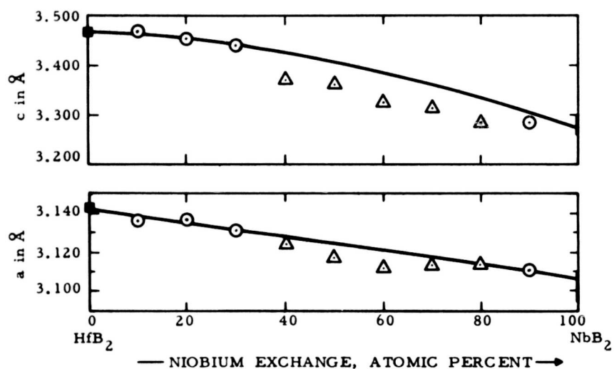
Figure 45. Lattice Parameters of Pseudo-Binary \text{HfB}_2\text{-NbB}_2 .
