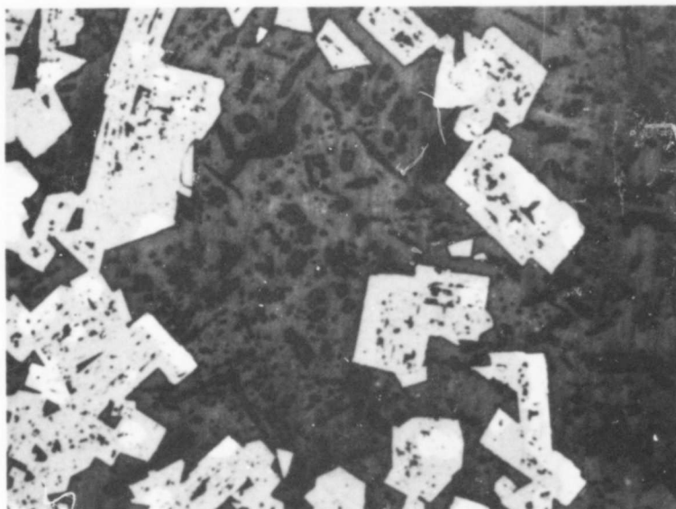
Figure 15. Micrograph of Ti-Zr-B (40-30-30) Alloy.
