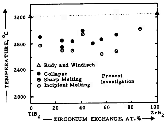
Figure 25. Observed Melting Temperatures of Ternary Diboride Alloys.
