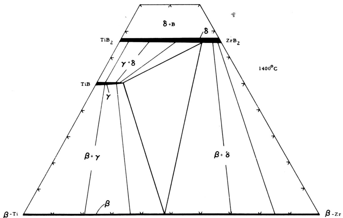
Figure 9. Isothermal Section at 1400°C.
