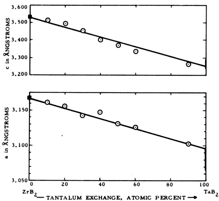
Figure 43. Lattice Parameters of Pseudo-Binary \text{ZrB}_2 - \text{TaB}_2 .
