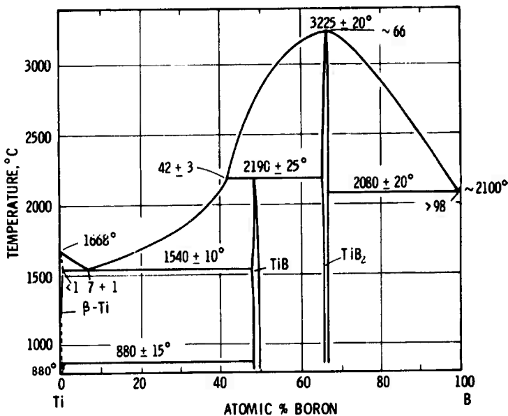
Figure 5. Phase Diagram Titanium-Boron.
