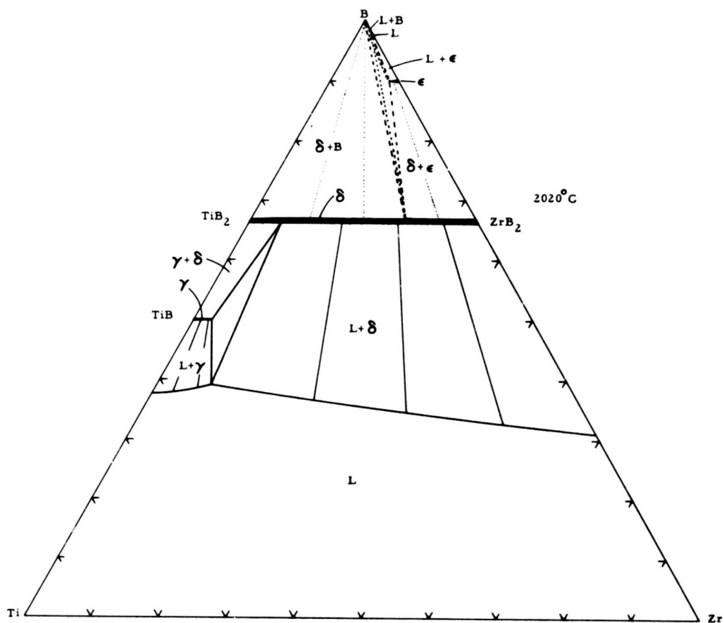
Figure 36. Isothermal section at 2020°C.
