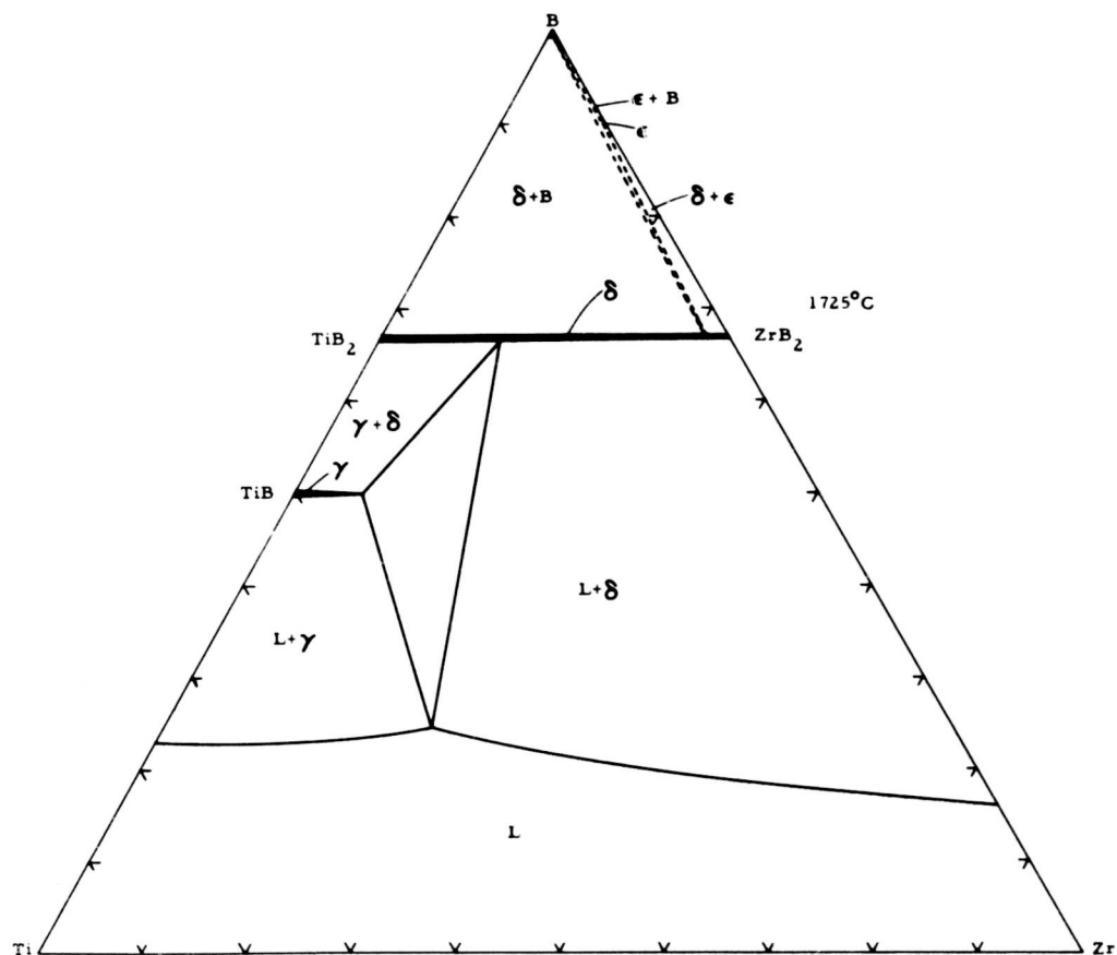
Figure 34. Isothermal Section at 1725°C.
