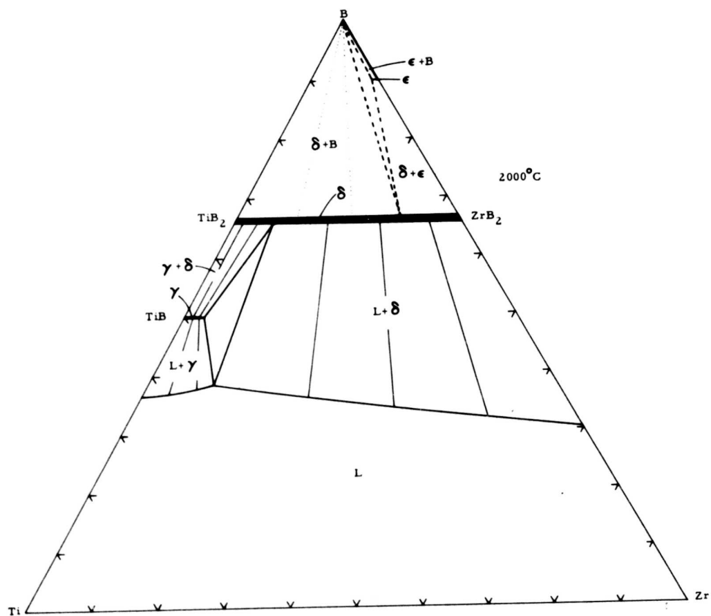
Figure 35. Isothermal Section at 2000°C.
