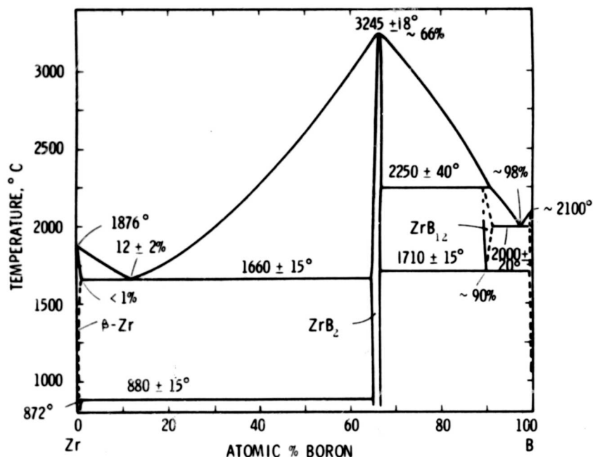
Figure 6. Phase Diagram Zirconium-Boron
