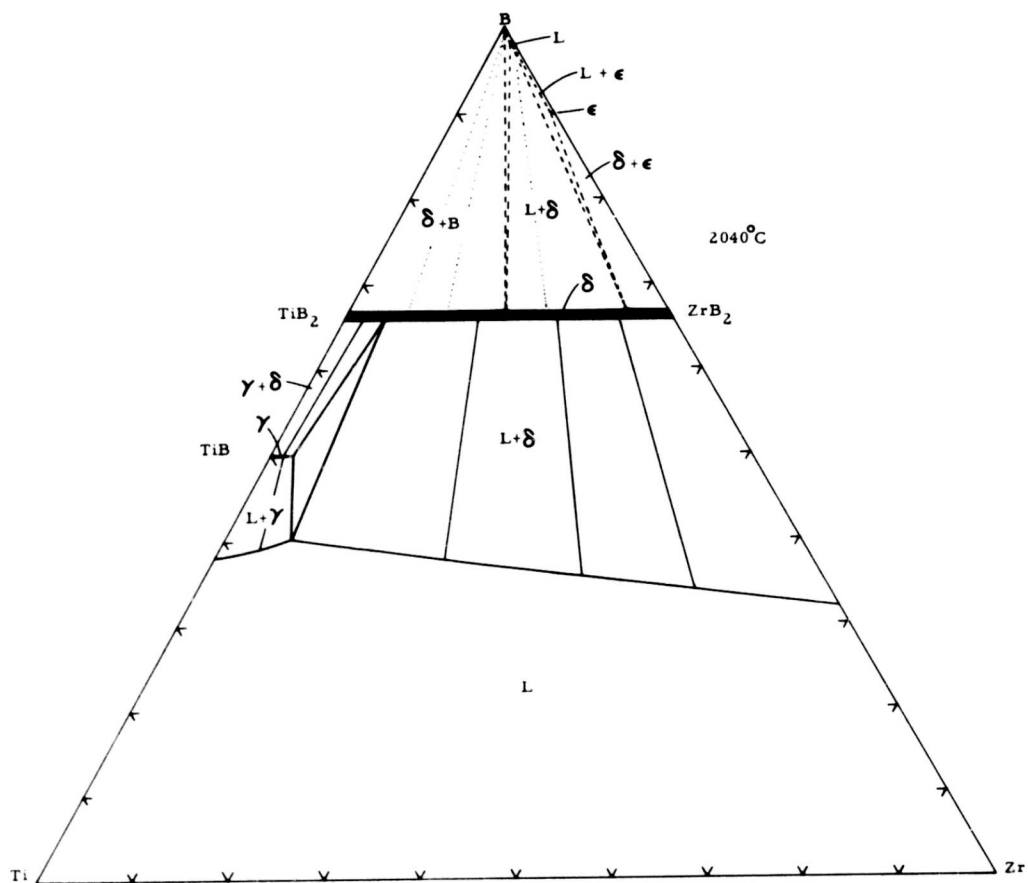
Figure 37. Isothermal Section at 2040°C.
