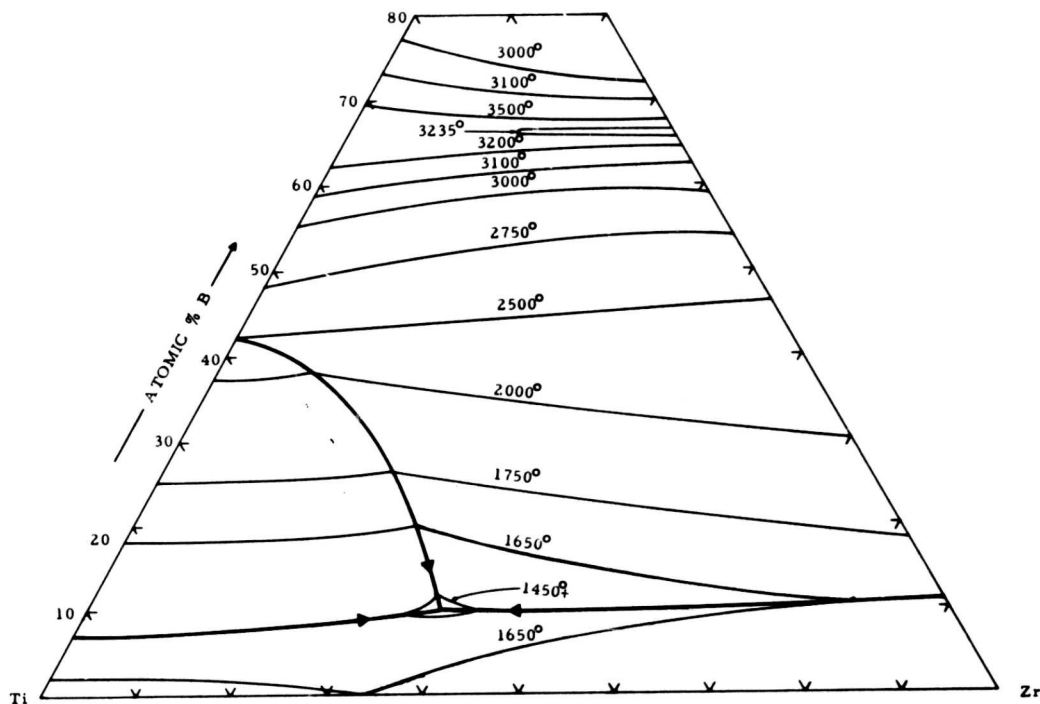
Figure 24. Plot of Liquidus Projections.
