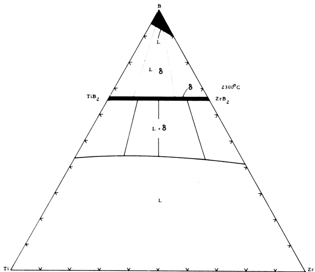
Figure 39. Isothermal Section at 2300°C.
