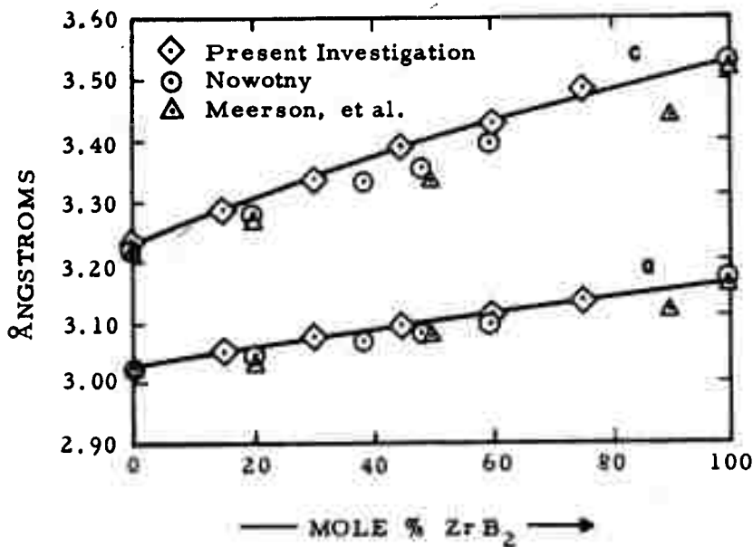
Figure 19. Lattice Parameters of Ternary Diboride Alloys Equilibrated at 1400°C.
