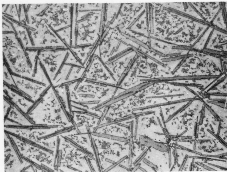
Figure 13. Micrograph of an Arc-Melted, Ti-Zr-B (10-60-30) Alloy.
