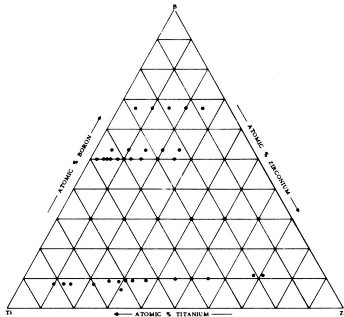
Figure 8. Composition of Alloys Investigated for the Solid State Section at 1400°C.
