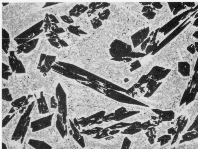
Figure 10. Primary Monoboride and Monoboride-Metal Eutectic. Ti-Zr-B: 60-10-30.
