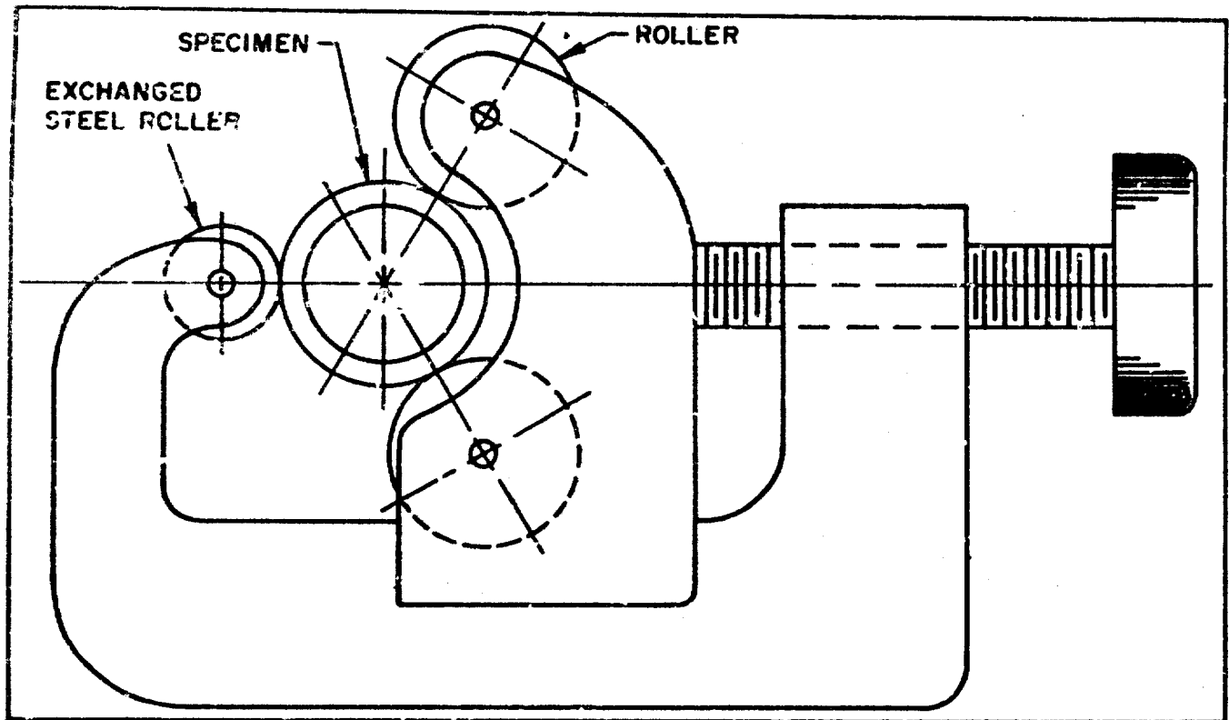
Figure 4. Rolling Device
