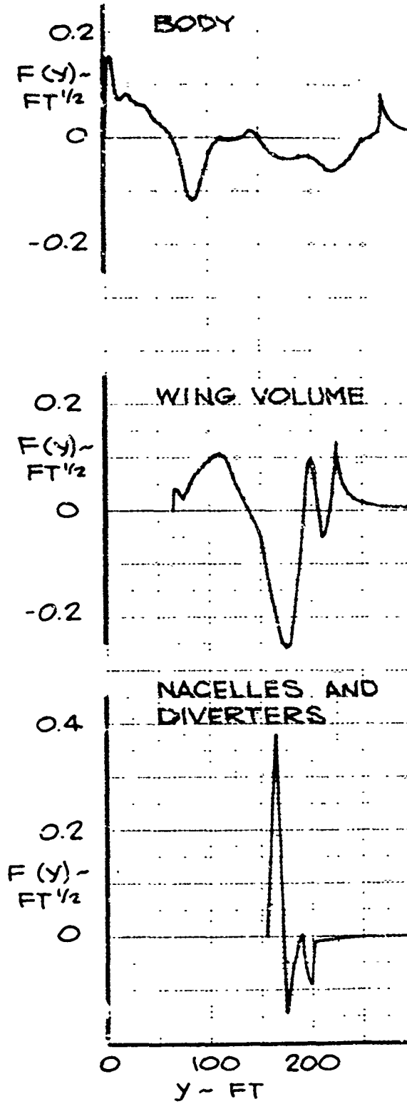
FIG. 2-8 COMPONENT AREA DISTRIBUTIONS AND F(Y) FUNCTIONS ( M=1.5 )
