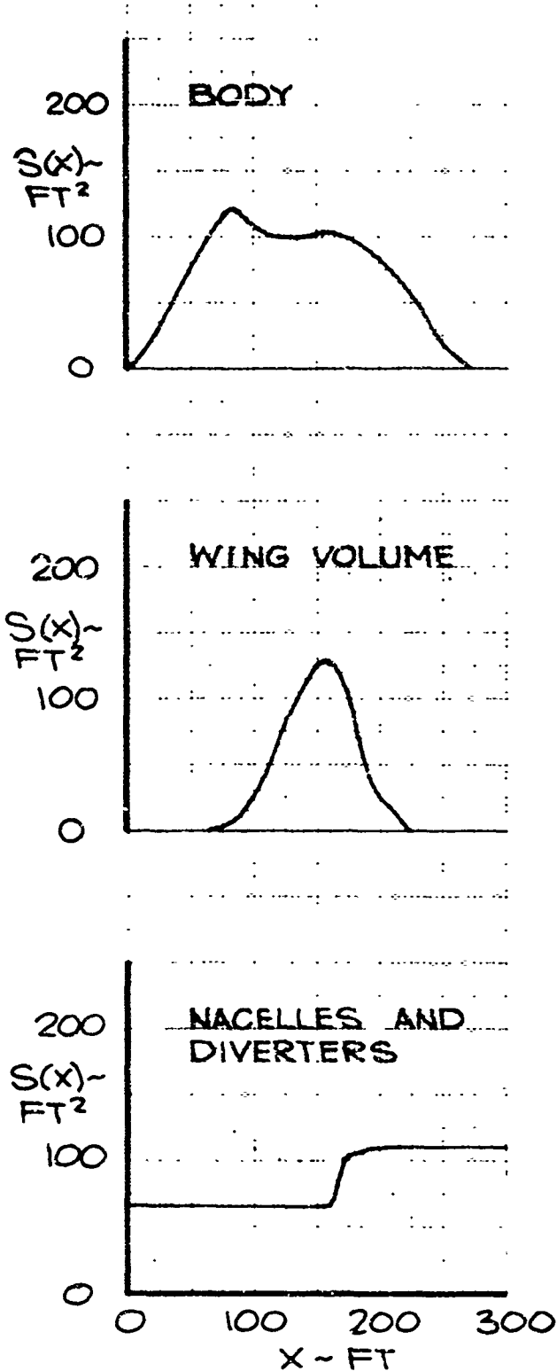
FIG. 2-8 COMPONENT AREA DISTRIBUTIONS AND F(Y) FUNCTIONS ( M=1.5 )
