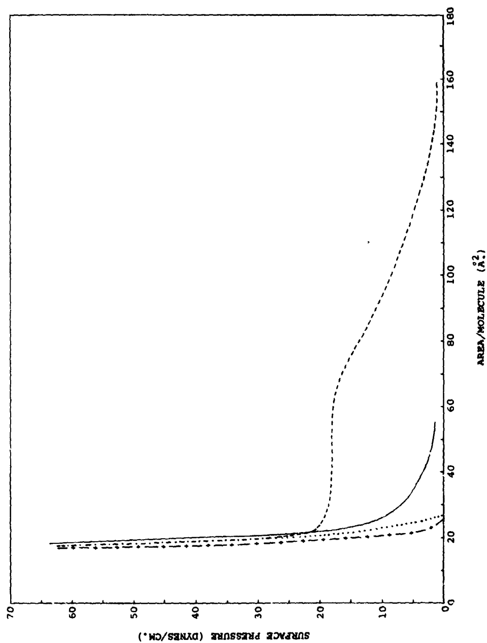
Fig. 9.— Pressure-area curves for stearic acid (—), an equimolar mixture of stearic acid and compound A013 (.....), an equimolar mixture of stearic acid and compound A014 (---) and an equimolar mixture of stearic acid and compound A029 (—). At 27.5 dynes/cm., the ascending curve (---) represents the merged isotherms for the runs with A013 and A014.
