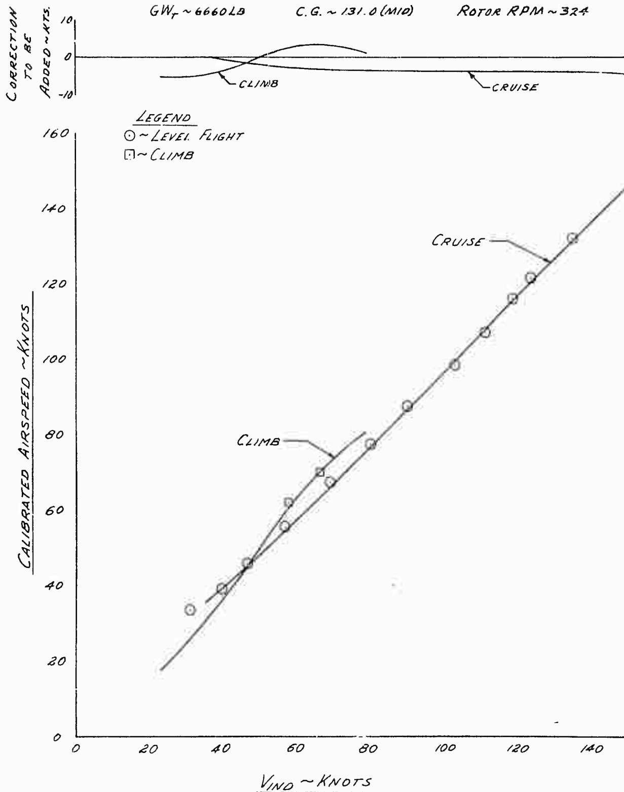
FIGURE No. 33 AIRSPED CALIBRATION UH-1B USA S/N 63-8684 BELL MODEL 540 ROTOR SYSTEM SHIPS SYSTEM
