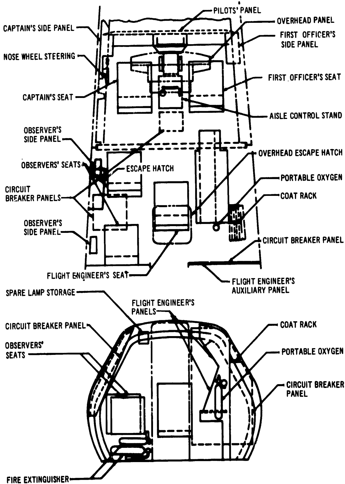
Fig. 6-1 Flight Deck Arrangement
