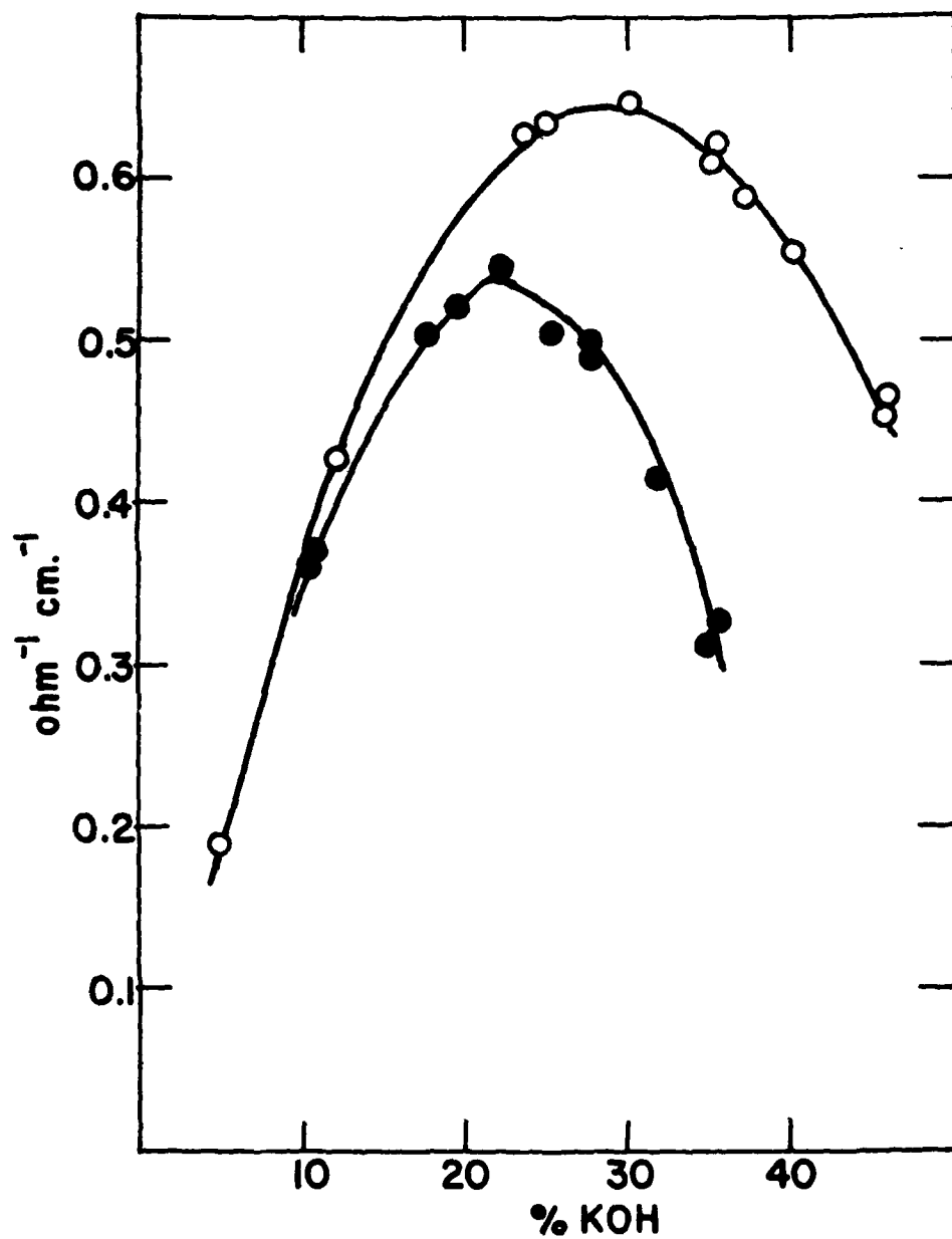
Figure 7. Specific conductance of KOH solutions at 25° C. Open circles, KOH solutions; closed circles, KOH solutions saturated with \text{ZnO} .
