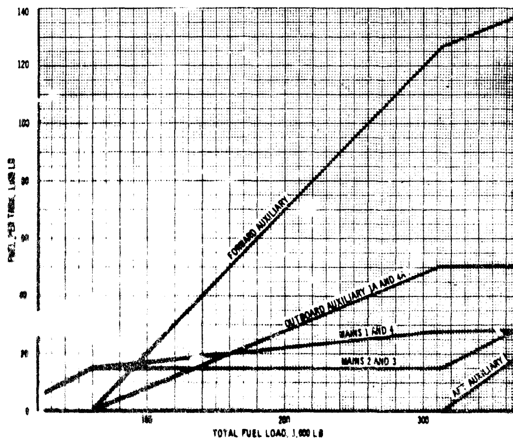
Figure 5-2. Fuel Loading
