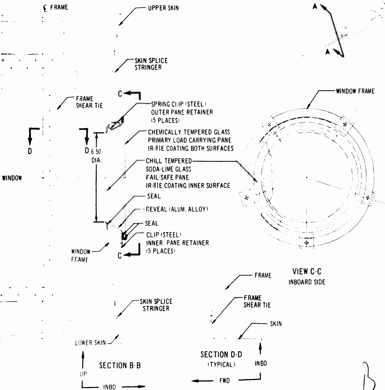
Figure 3-39. Passenger Window
