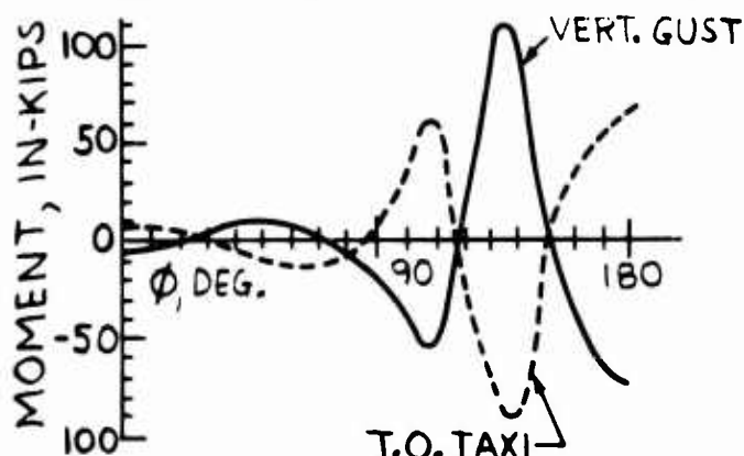
Figure 4-50. Typical Fuselage Frame Analysis
