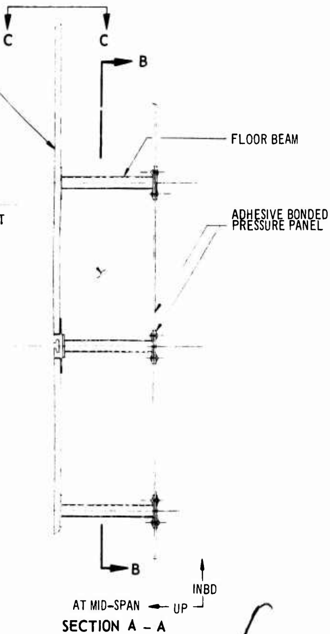
Figure 3-38. Floor Structure
