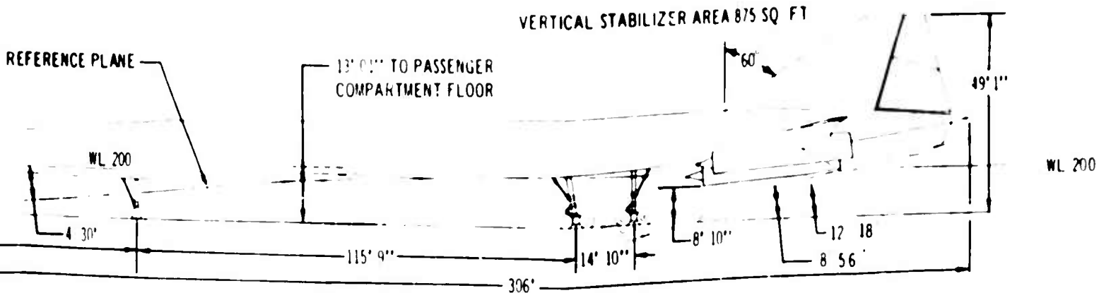
Figure 1-1. Airplane Three-View
