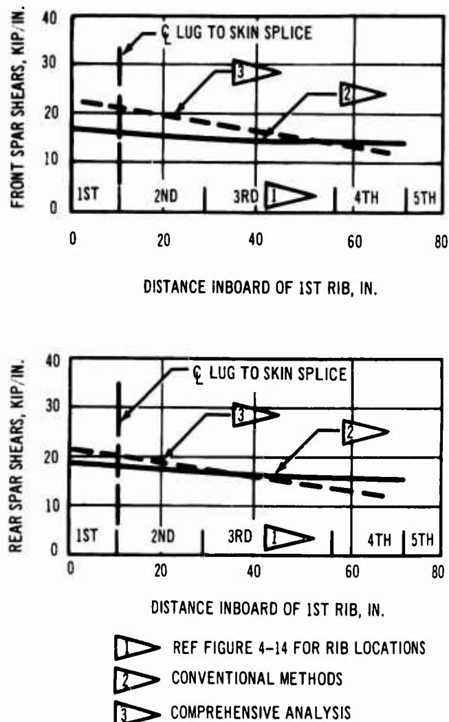
Figure 4-16 Relative Spar Shears Inboard Wing
