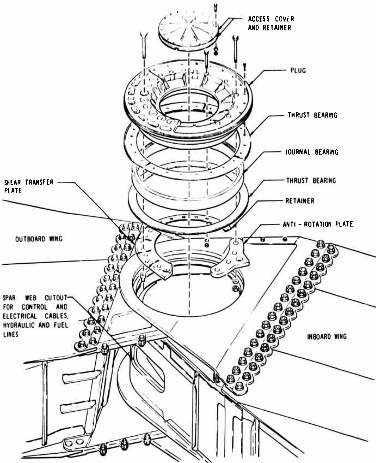
Figure 3-23. Pivot Arrangement
