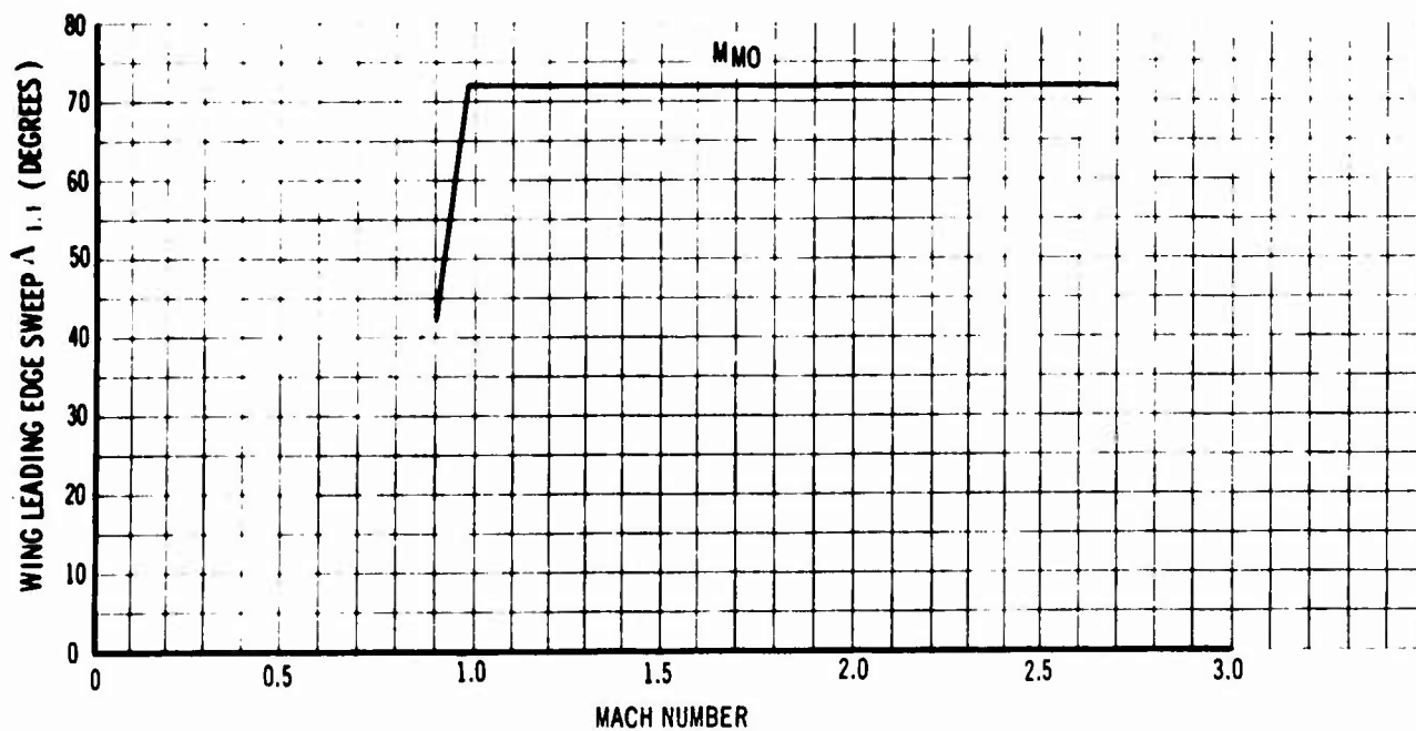
Figure 2-6. Wing Sweep Placard
