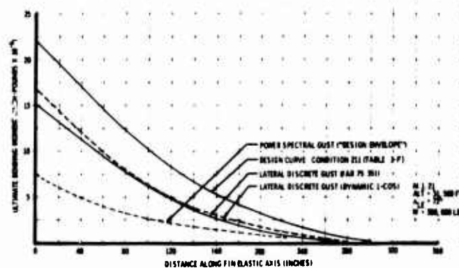
Figure 3-35. Fin Bending Moment Distribution
