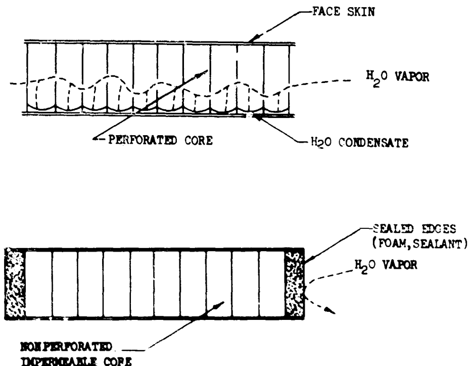
Figure 3-6. Sandwich Design
