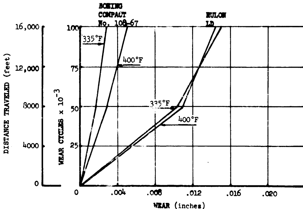
Figure 3-67. Wear Rate of Boeing Compact and Rulon LD
