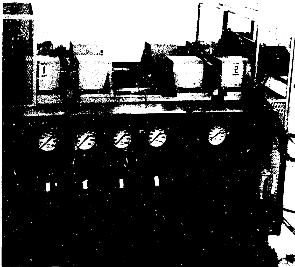
Figure 4-20. Reverse Load, Oscillating Motion, Bearing Test Machine
