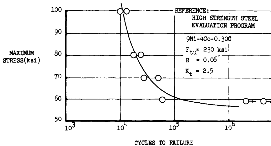
Figure 2-48. Fatigue Properties of 4340M and 9Ni-4Co-0.30C Steels
