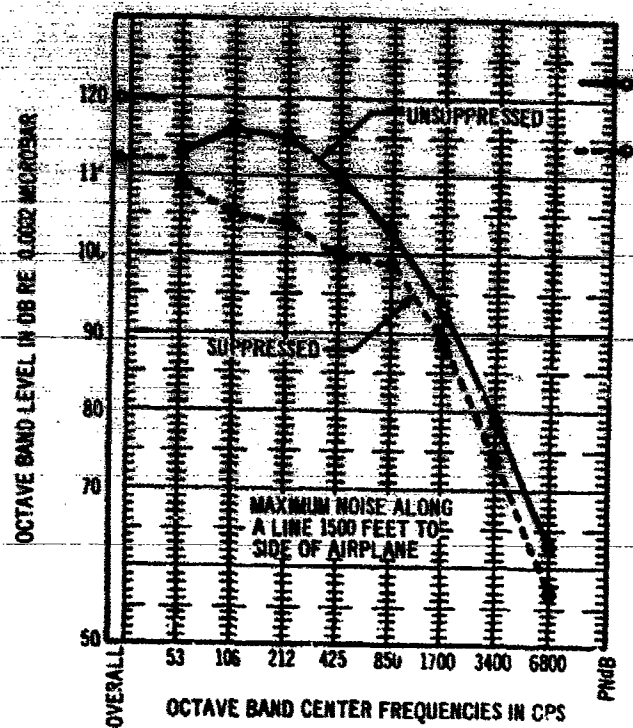
Figure 4-8. Boeing Jet Noise Suppression For Turbojet Engine
